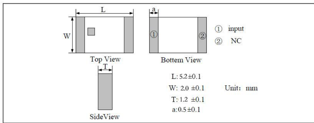
贴片陶瓷天线/SMD ceramic antennas
