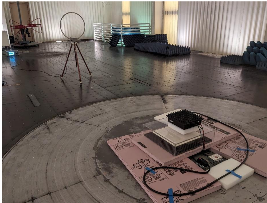
Photograph 2: Back View Radiated Emissions, Part 18
