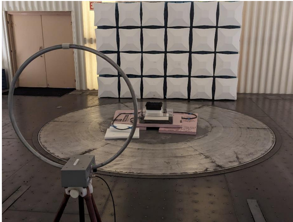
Photograph 1: Front View Radiated Emissions, Part 18
