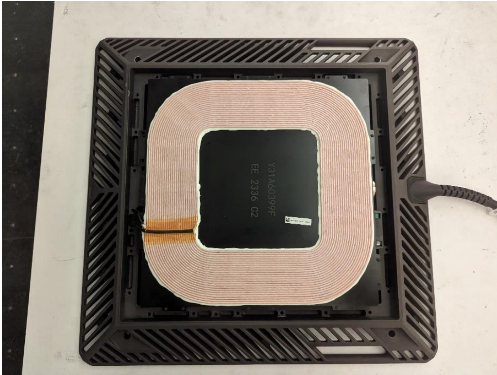
Photograph 7 – View of Power Transfer Coil
