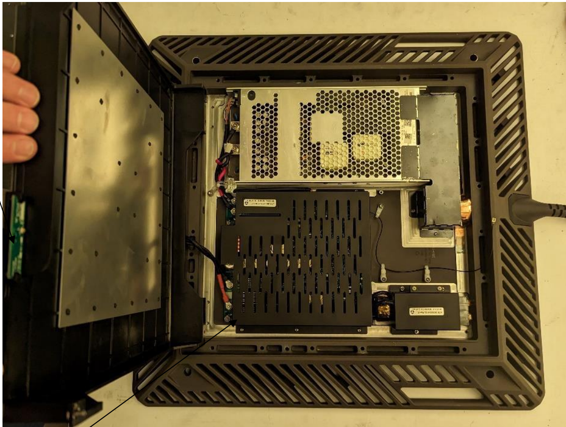
Photograph 6 – View of the PCB Mounting in the Enclosure
