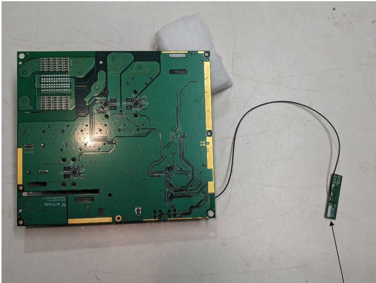
Photograph 2 – Back View of the PCBA
