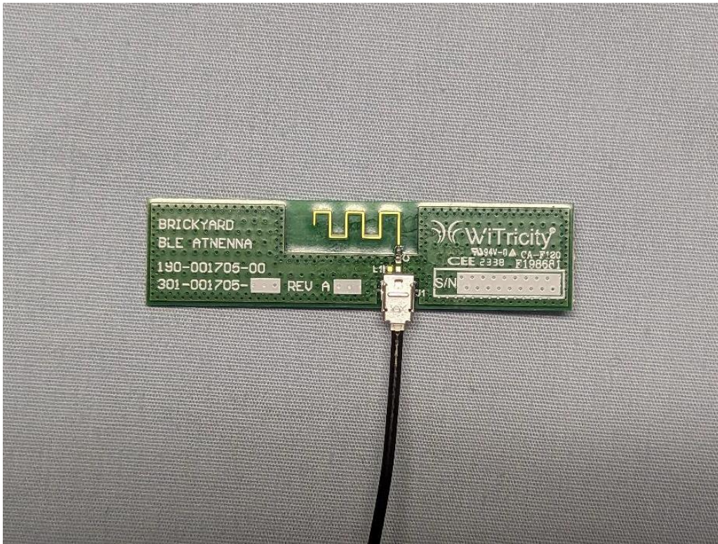
Photograph 4 – Top view of Antenna PCBA
