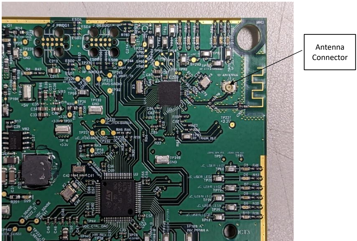
Photograph 3 – Close-up view of RF section
