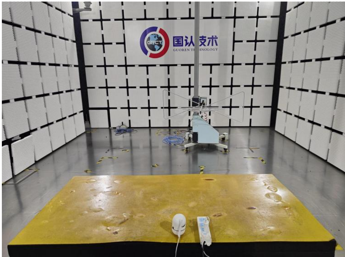
Test Setup Photos of the EUT
