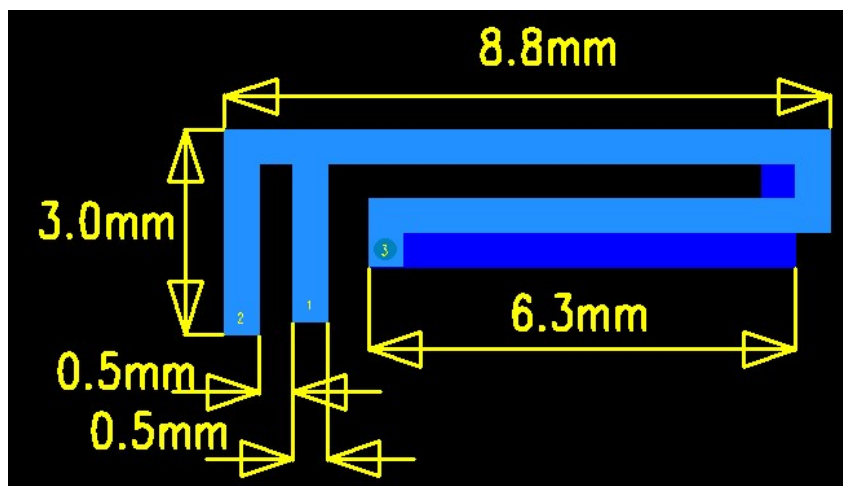
Figure 1 :Dongle Antenna
