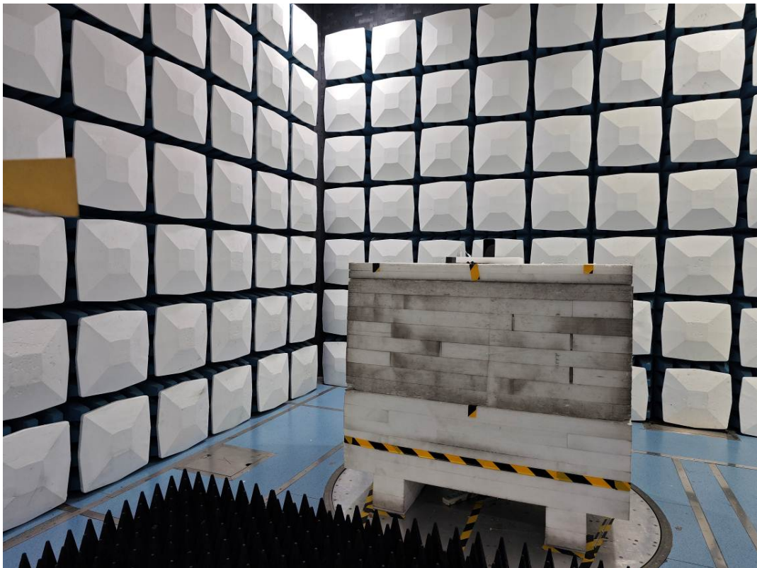
Radiated Emission Above 1GHz View-18-25G
