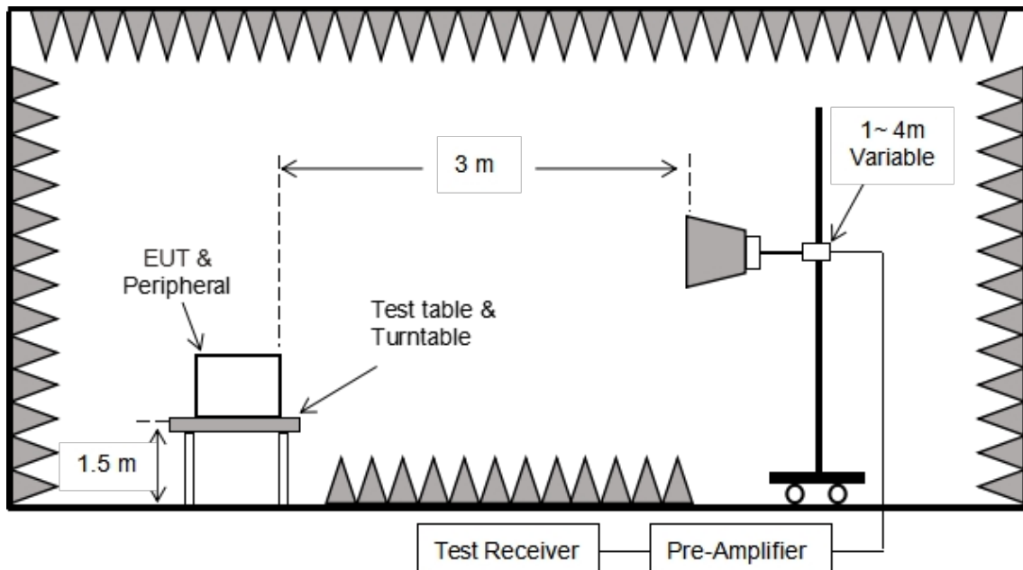
Figure 3. Above 1 GHz
