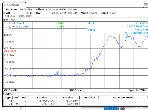
GFSK_Hopping_Lower
