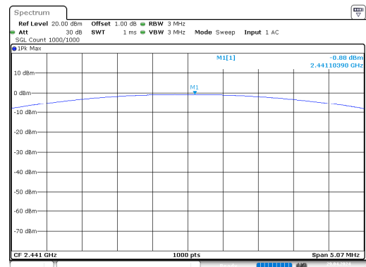
GFSK_Middle
