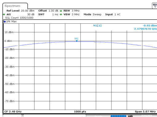
GFSK_High
