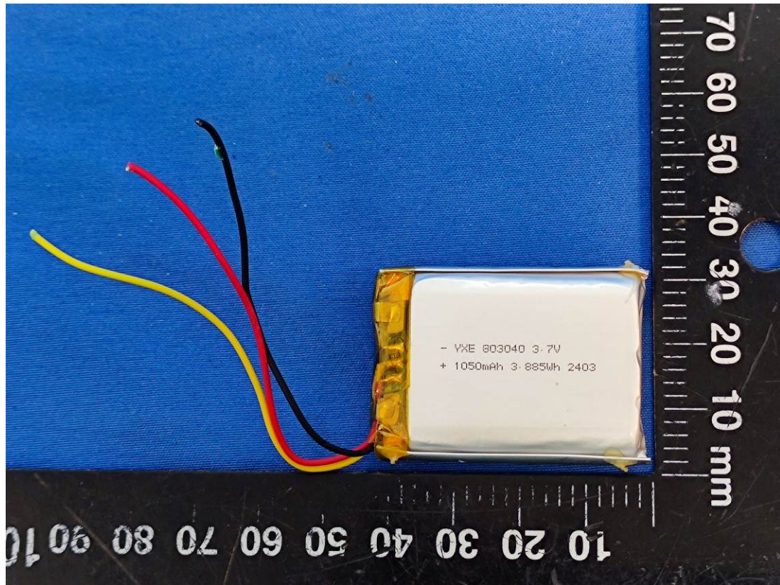
Battery
