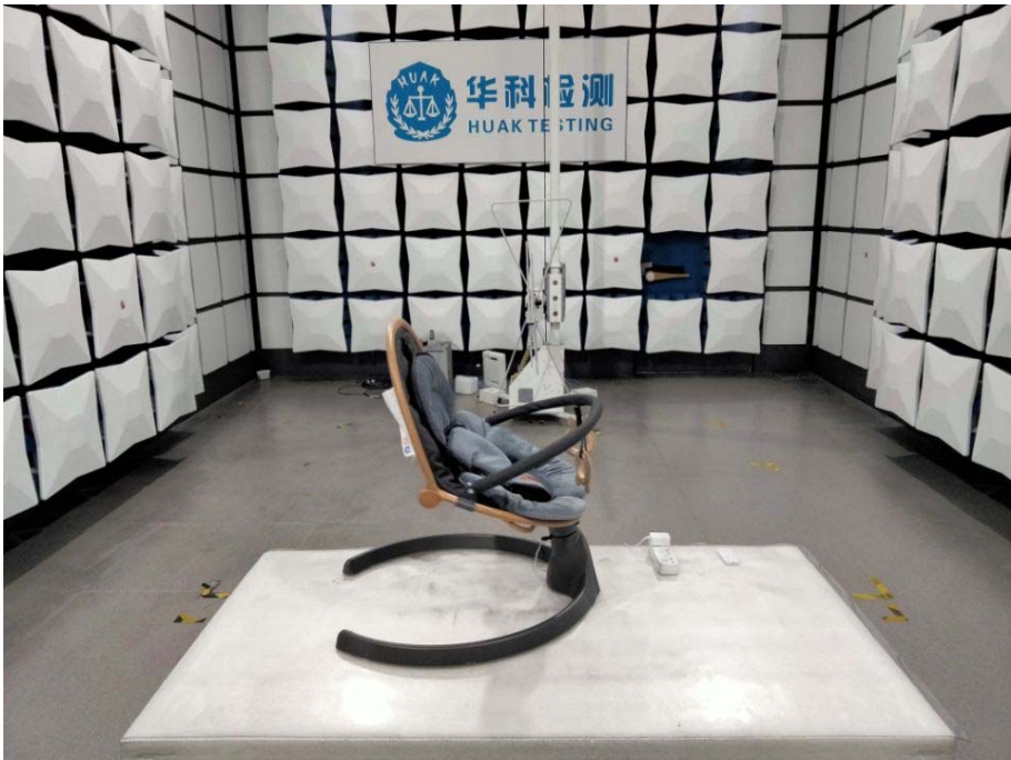
Test Model: BB2006 Radiated Emissions
