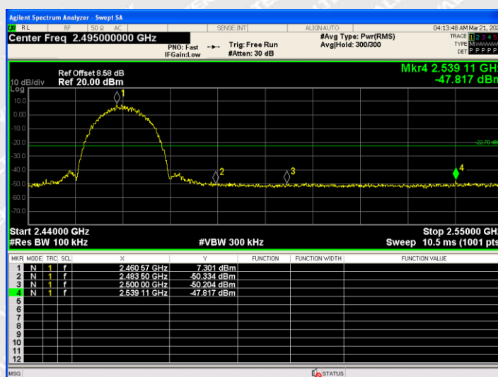
802.11b_High Channel
