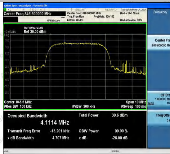
Band5-4233-2-PASS
