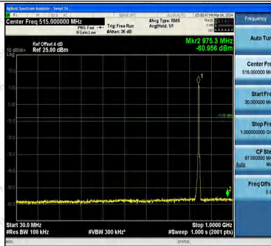
Band5-4233-2-30~1000MHz-PASS
