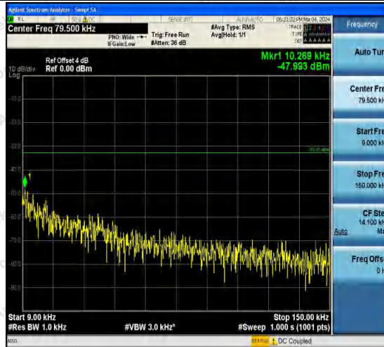
Band5-4132-1-0.009~0.15MHz-PASS
