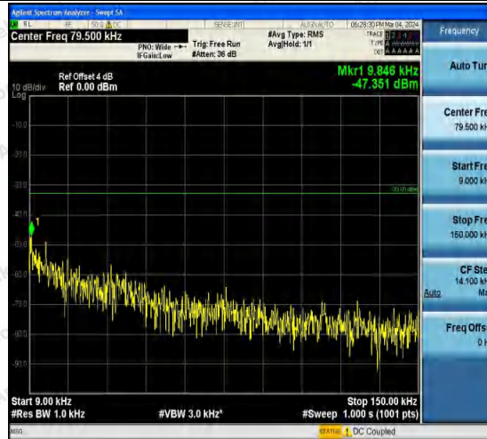
Band5-4132-4-0.009~0.15MHz-PASS
