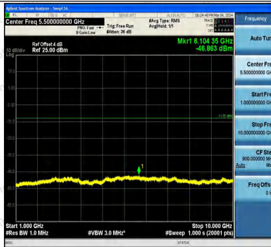
Band5-4182-2-1000~10000MHz-PASS
