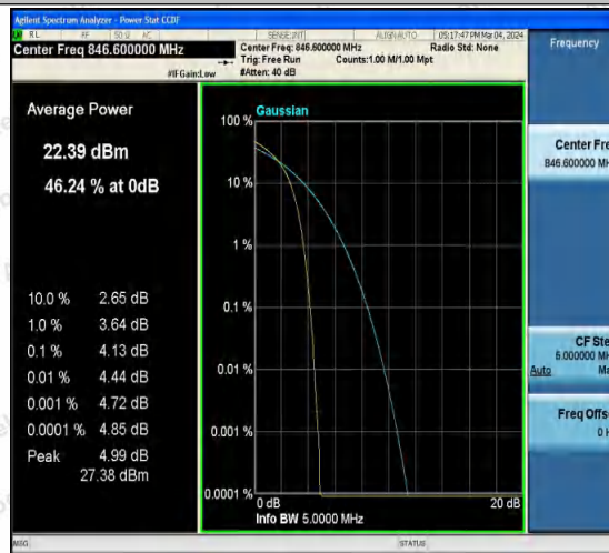
Band5-4233-5-PASS
