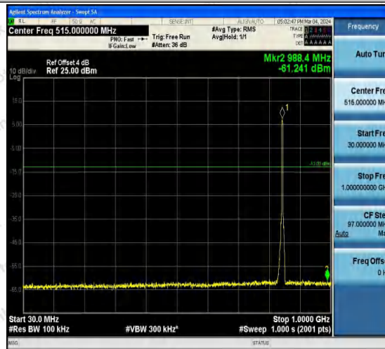
Band5-4233-3-30~1000MHz-PASS
