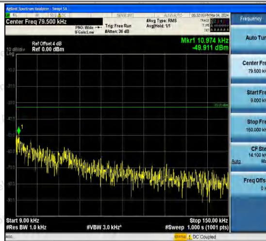
Band5-4233-5-0.009~0.15MHz-PASS
