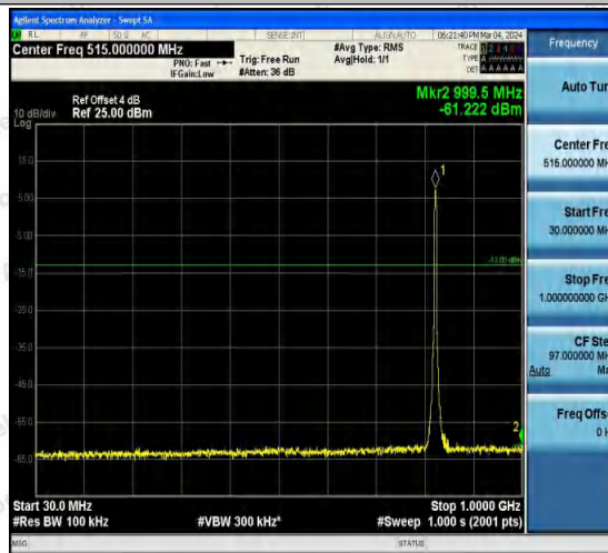
Band5-4132-1-30~1000MHz-PASS
