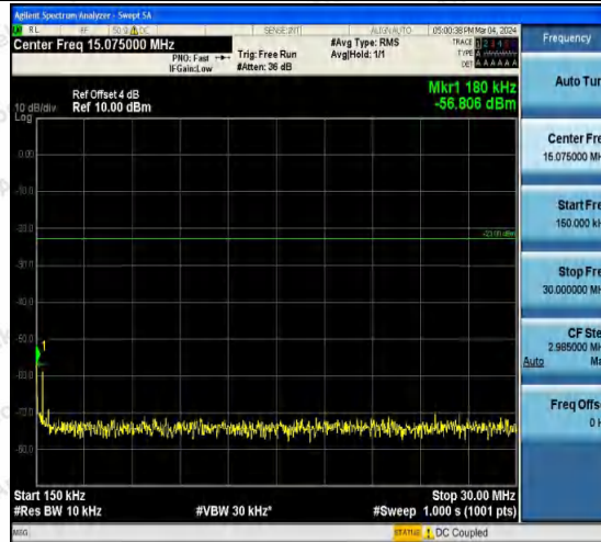
Band5-4233-2-0.15~30MHz-PASS
