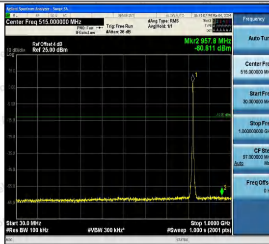
Band5-4132-5-30~1000MHz-PASS
