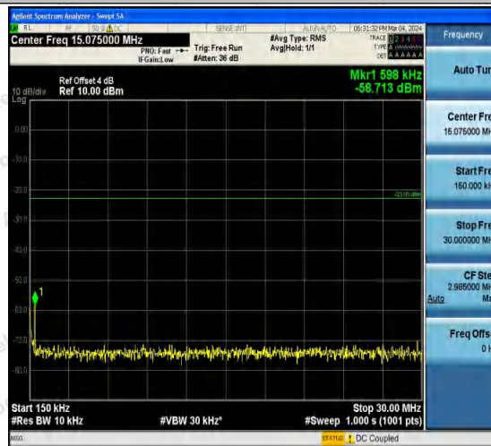
Band5-4182-5-0.15~30MHz-PASS
