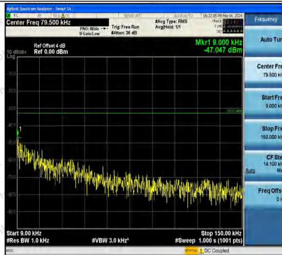
Band5-4182-1-0.009~0.15MHz-PASS
