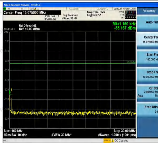
Band5-4132-3-0.15~30MHz-PASS
