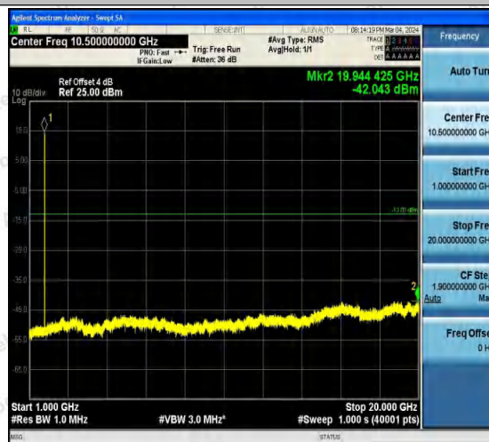
Band4-1513-3-1000~20000MHz-PASS
