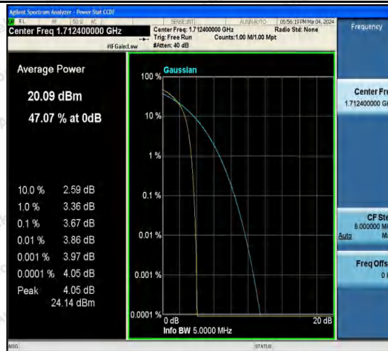
Band4-1312-5-PASS
