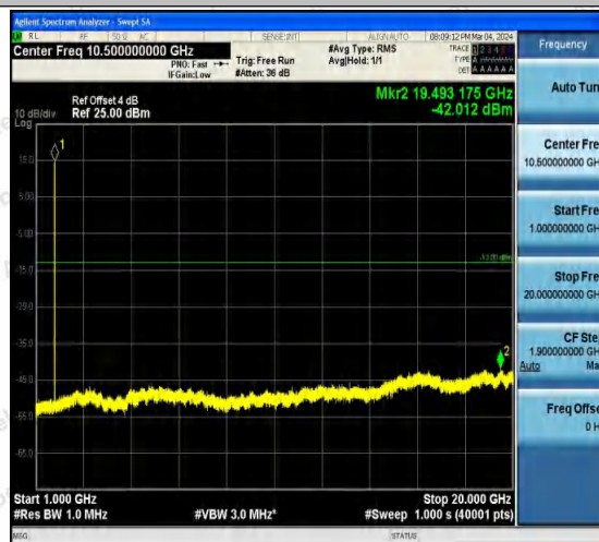
Band4-1513-1-1000~20000MHz-PASS
