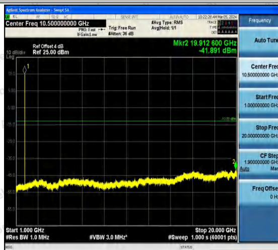
Band4-1513-2-1000~20000MHz-PASS
