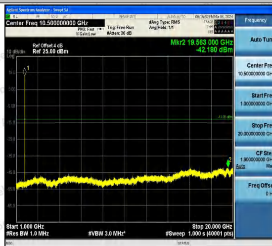
Band4-1513-4-1000~20000MHz-PASS
