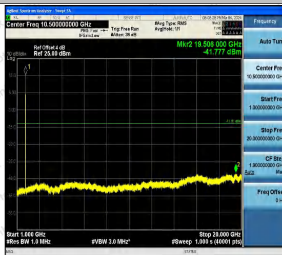
Band4-1413-1-1000~20000MHz-PASS
