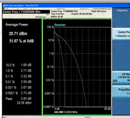
Band4-1413-1-PASS
