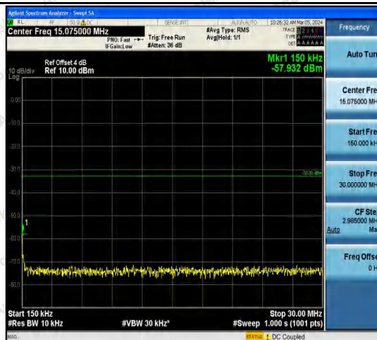
Band4-1513-4-0.15~30MHz-PASS
