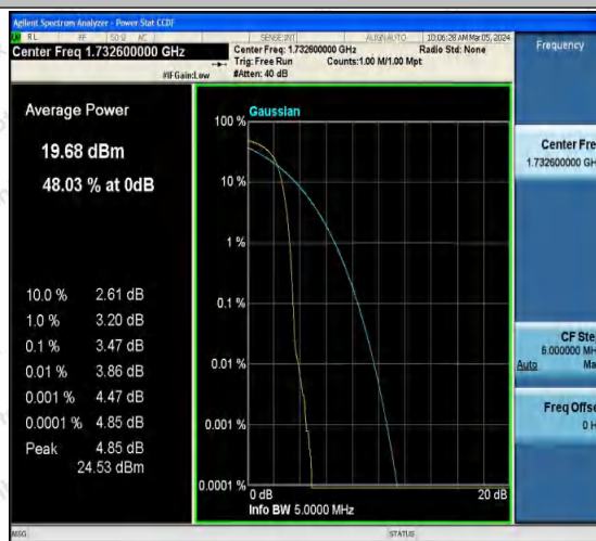
Band4-1413-2-PASS
