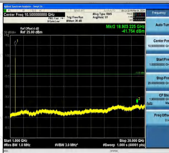
Band4-1413-3-1000~20000MHz-PASS
