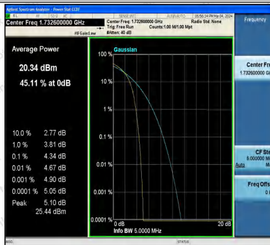
Band4-1326-5-PASS
