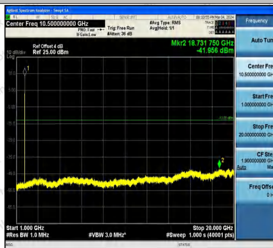
Band4-1413-2-1000~20000MHz-PASS
