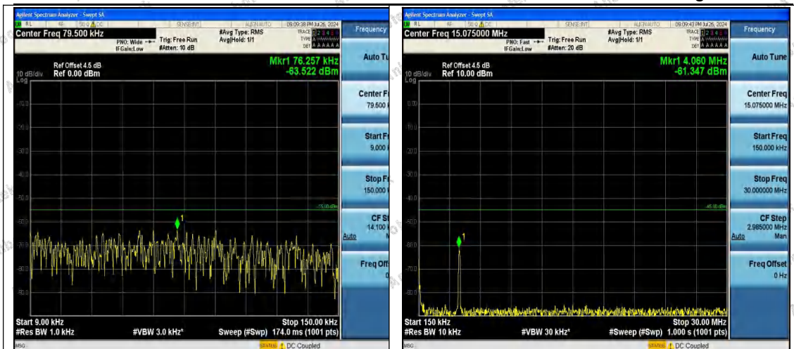
Band7_5MHz_16QAM_21425_1RB#0_0.009~0.15_0.009~0.15
