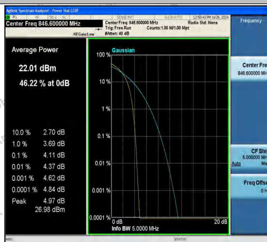
Band5-4233-5-PASS
