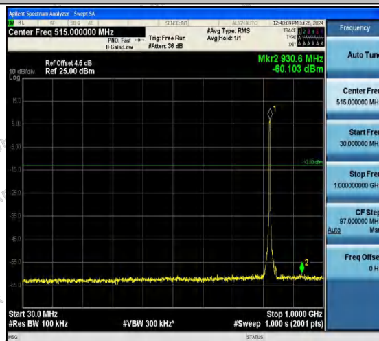
Band5-4132-2-30~1000MHz-PASS
