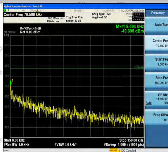
Band5-4182-1-0.009~0.15MHz-PASS
