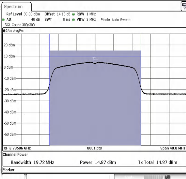
11AC20SISO-Ant1-5785-PASS
