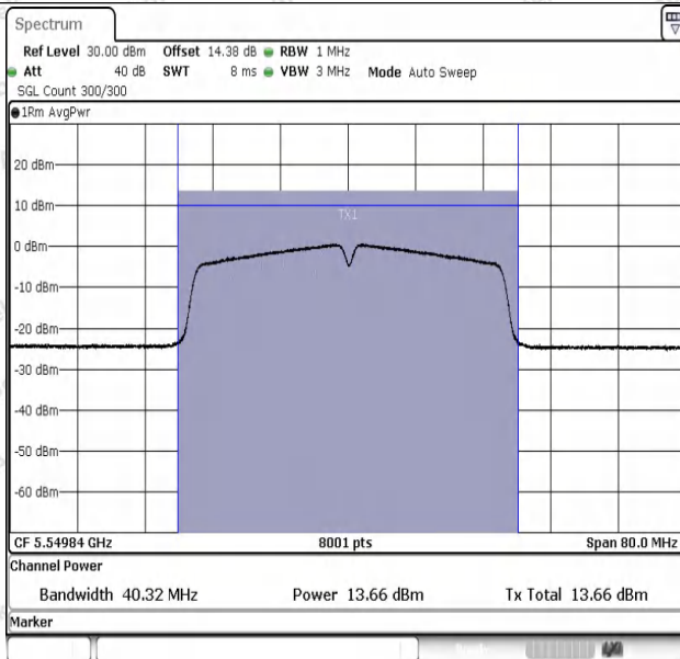
11AC40SISO-Ant1-5550-PASS
