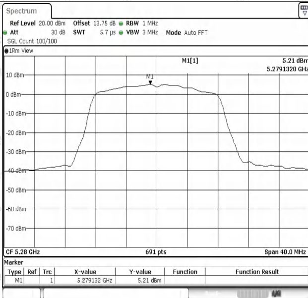
11A-Ant1-5280-PASS
