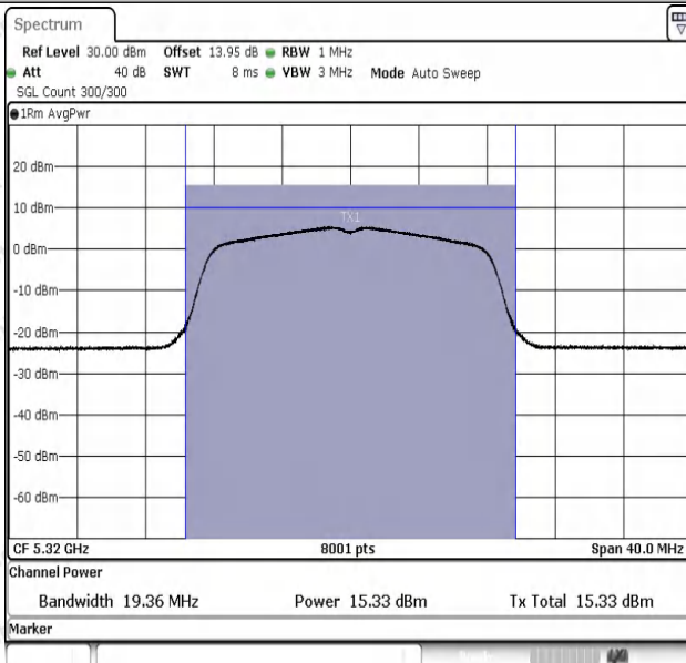
11A-Ant1-5320-PASS
