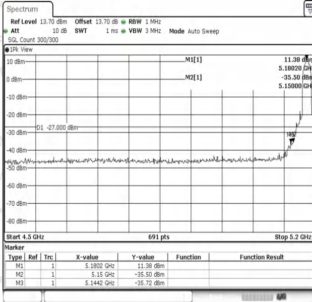
11AC20SISO-Ant1-5180-PASS
