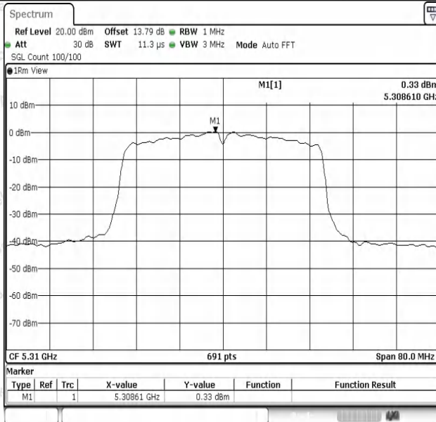
11AC40SISO-Ant1-5310-PASS
