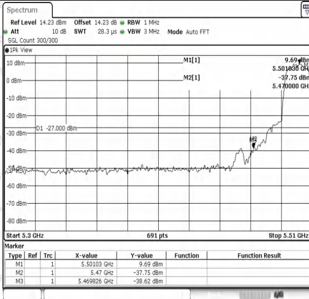
11A-Ant1-5500-PASS
