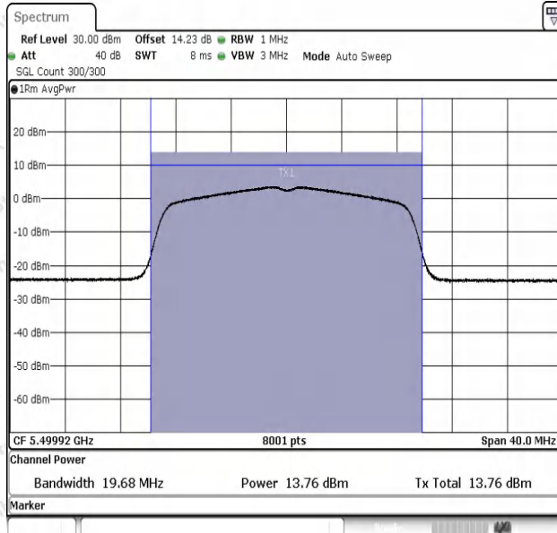
11AC20SISO-Ant1-5500-PASS
