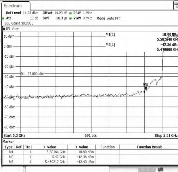
11AC20SISO-Ant1-5500-PASS
