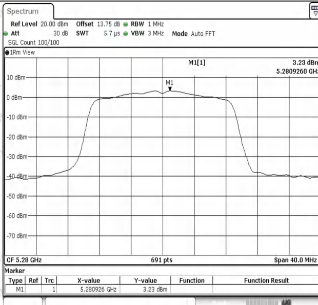
11AC20SISO-Ant1-5280-PASS
