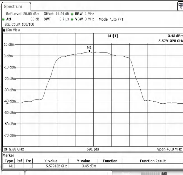
11A-Ant1-5580-PASS
