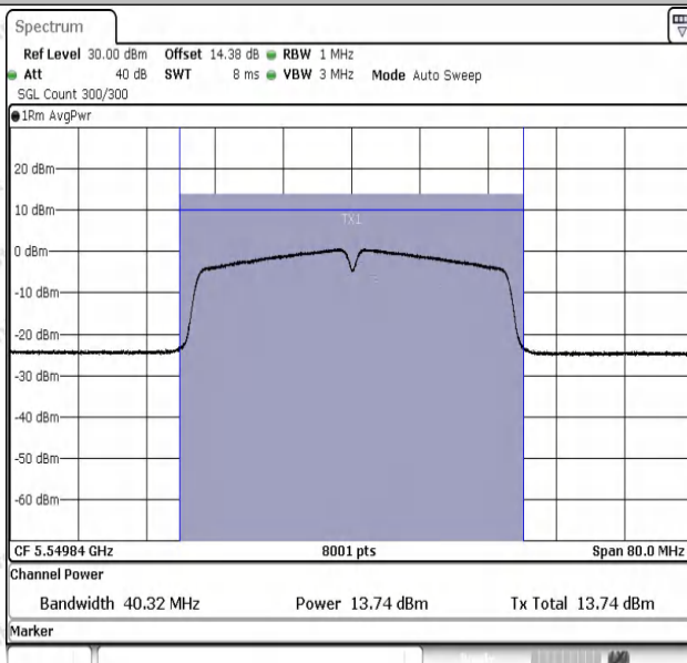
11N40SISO-Ant1-5550-PASS
