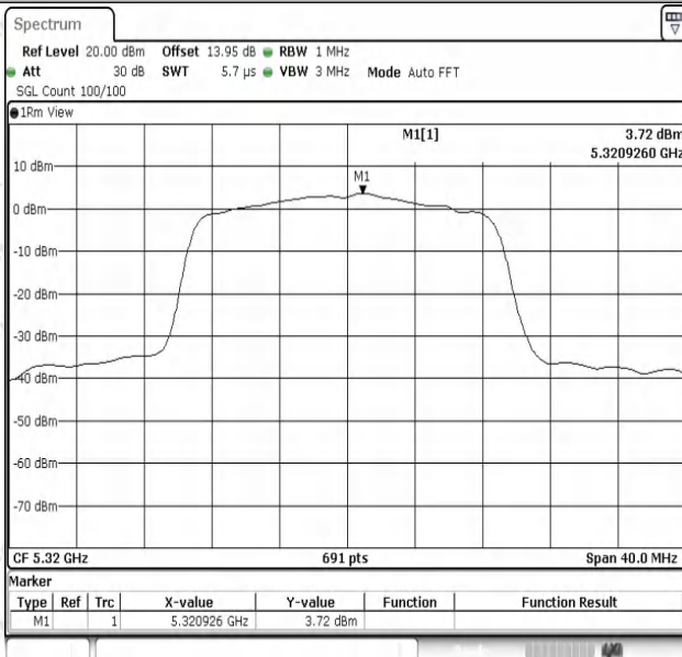
11N20SISO-Ant1-5320-PASS
