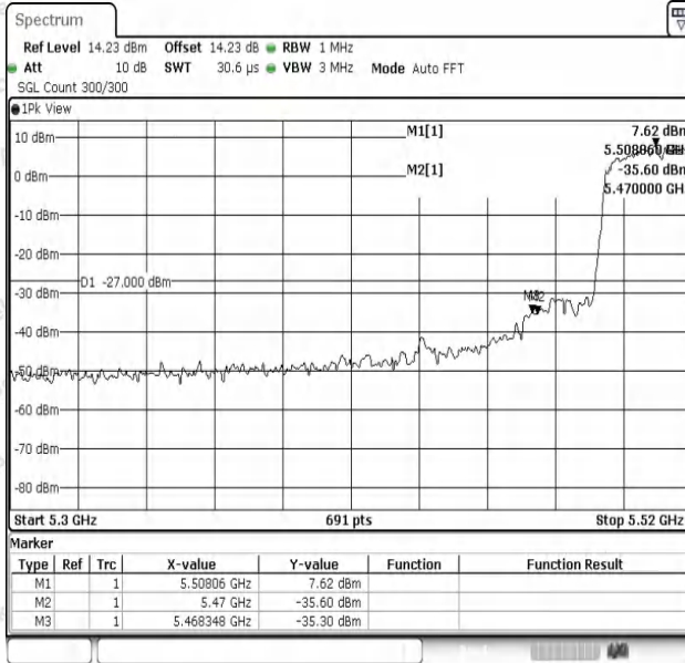
11N40SISO-Ant1-5510-PASS
