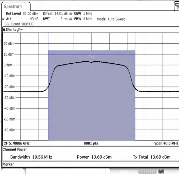
11A-Ant1-5700-PASS
