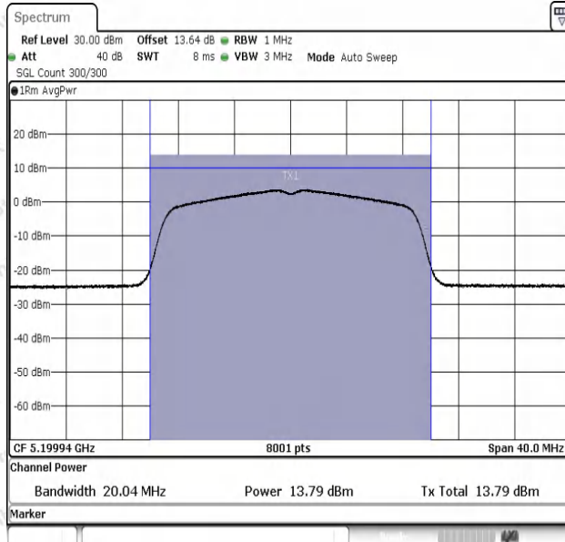
11N20SISO-Ant1-5200-PASS
