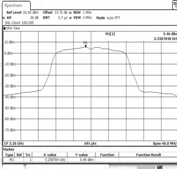
11A-Ant1-5260-PASS
