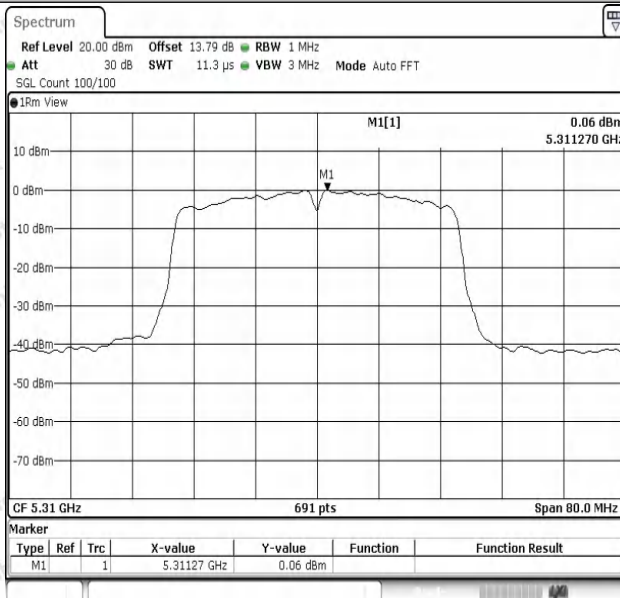
11N40SISO-Ant1-5310-PASS
