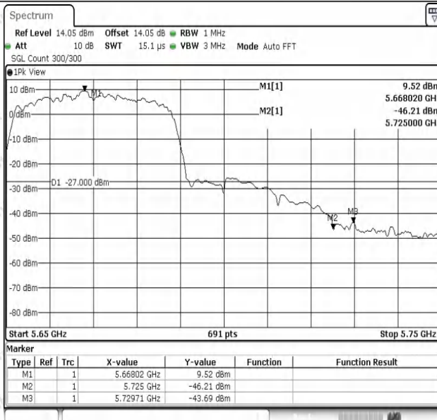
11AC40SISO-Ant1-5670-PASS
