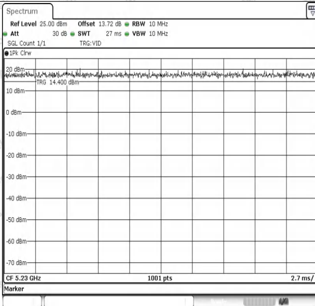
NTNV-11AC40SISO-Ant1-5230
