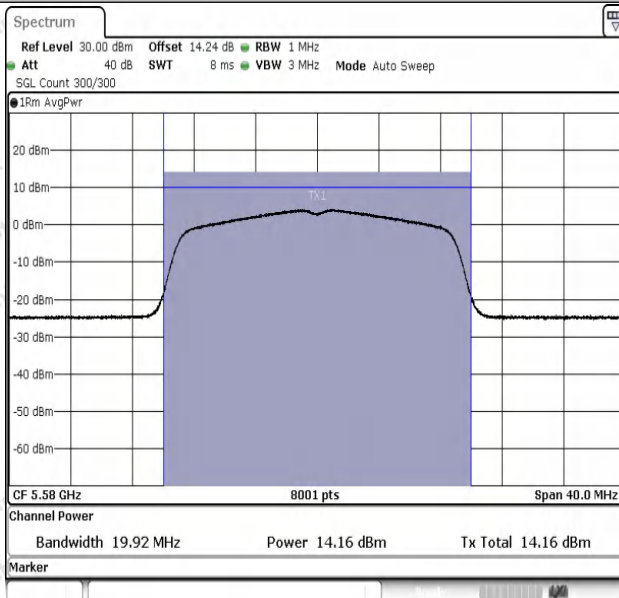
11N20SISO-Ant1-5580-PASS
