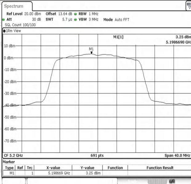
11AC20SISO-Ant1-5200-PASS
