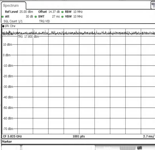
NTNV-11AC20SISO-Ant1-5825
