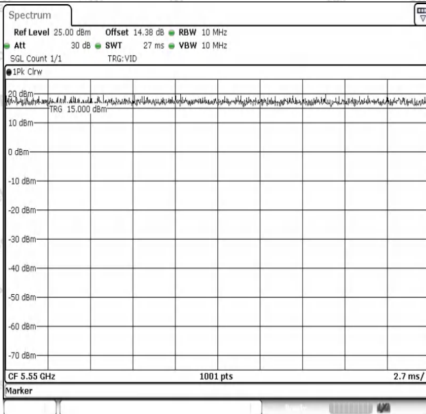
NTNV-11AC40SISO-Ant1-5550
