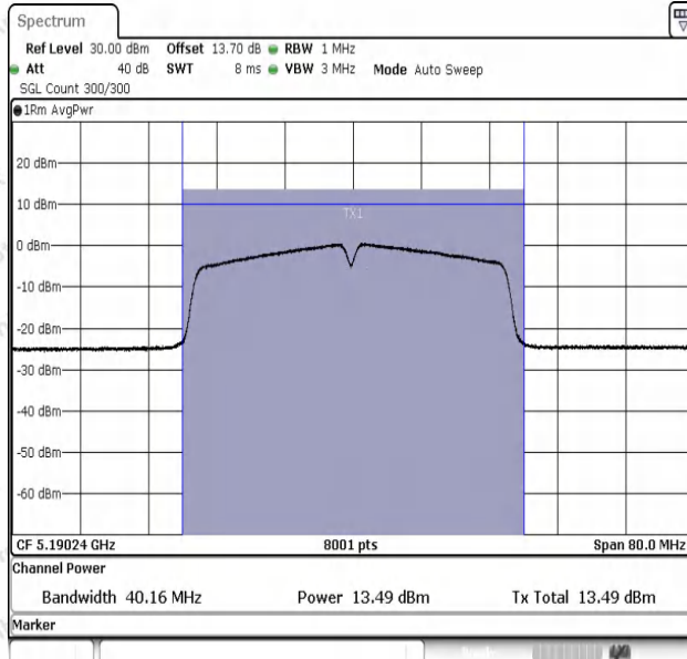
11AC40SISO-Ant1-5190-PASS
