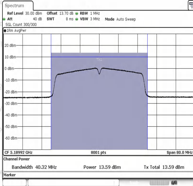
11N40SISO-Ant1-5190-PASS
