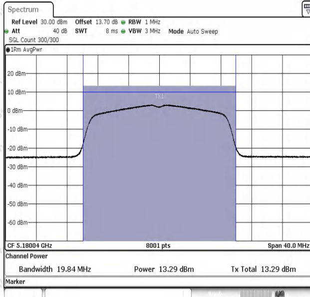
11AC20SISO-Ant1-5180-PASS
