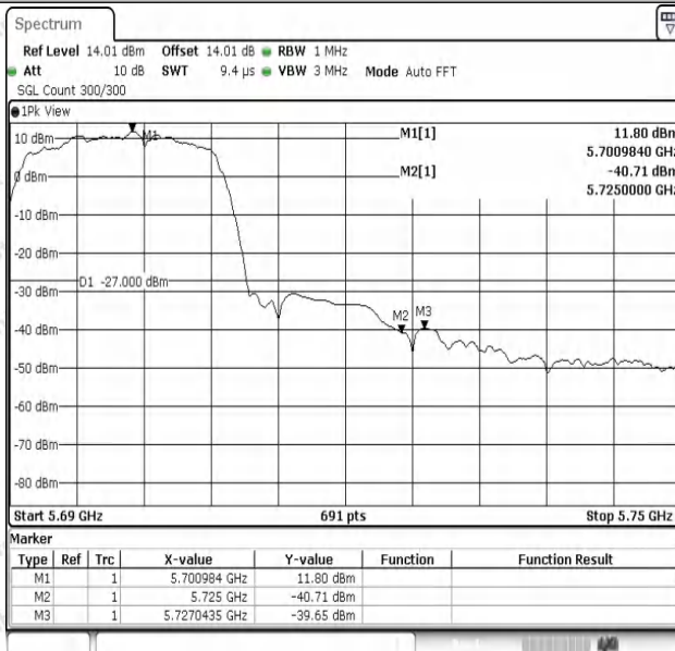
11N20SISO-Ant1-5700-PASS
