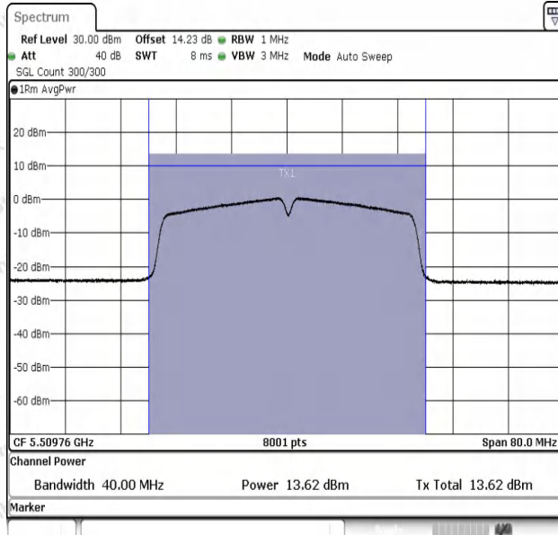
11AC40SISO-Ant1-5510-PASS
