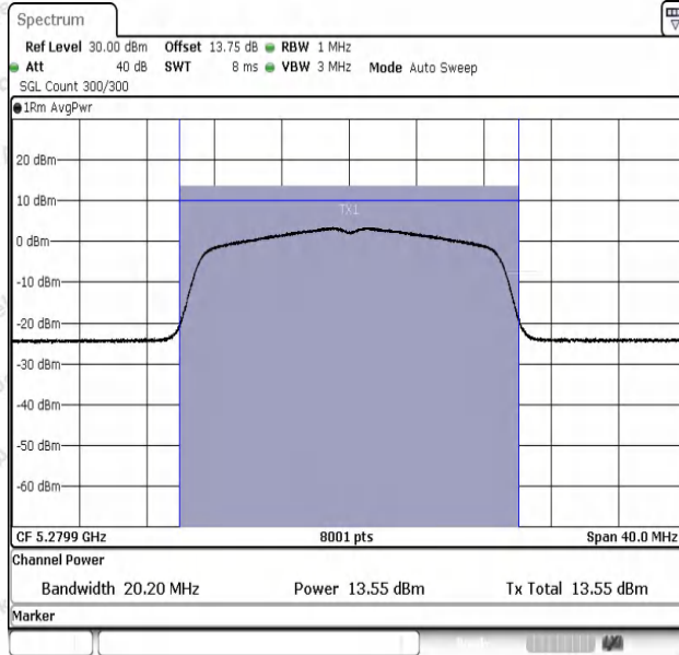
11N20SISO-Ant1-5280-PASS
