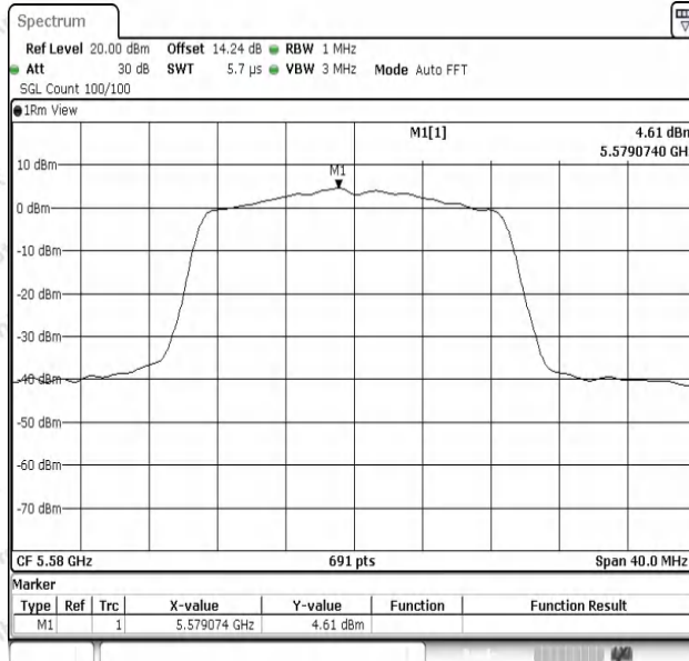
11N20SISO-Ant1-5580-PASS
