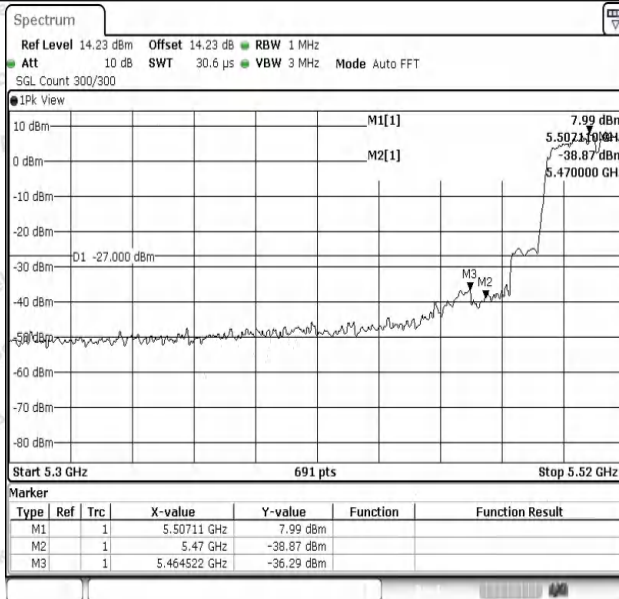
11AC40SISO-Ant1-5510-PASS
