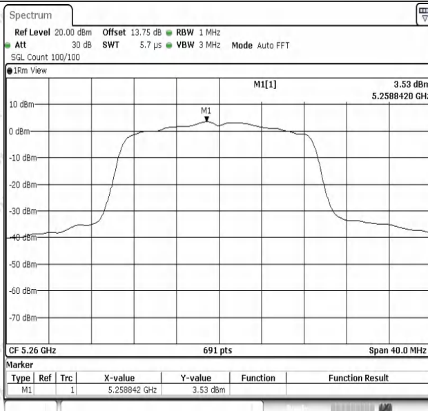
11N20SISO-Ant1-5260-PASS
