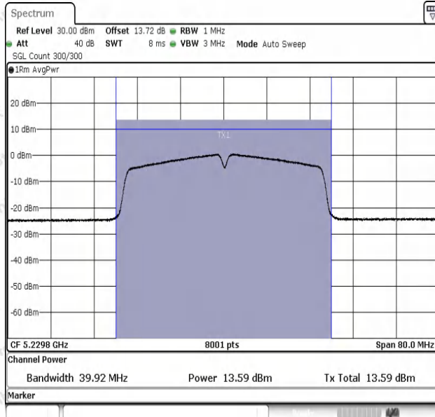
11N40SISO-Ant1-5230-PASS
