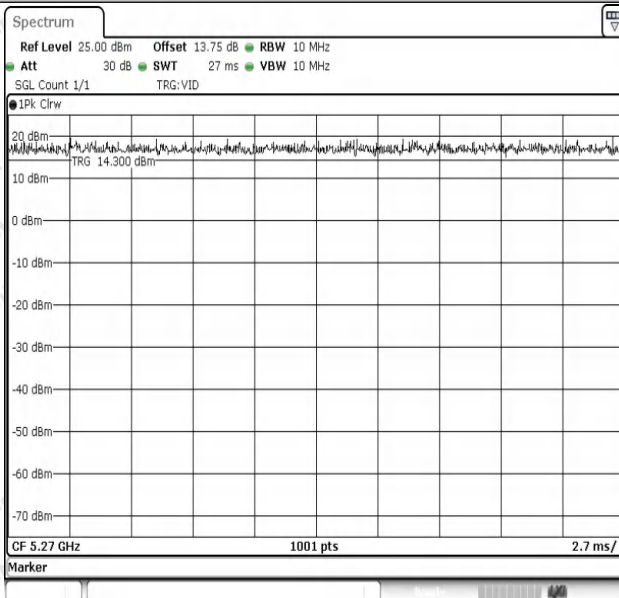
NTNV-11AC40SISO-Ant1-5270
