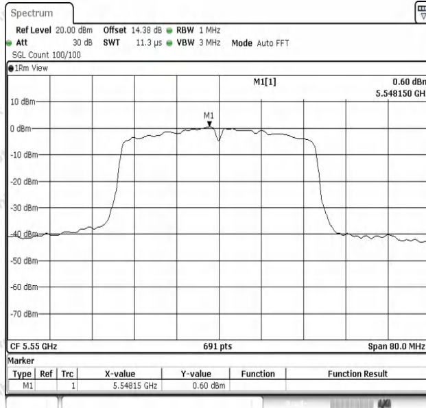
11N40SISO-Ant1-5550-PASS
