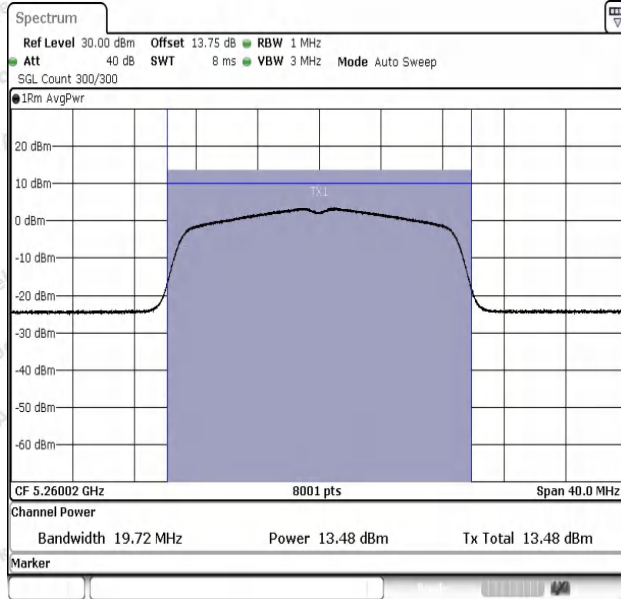
11AC20SISO-Ant1-5260-PASS
