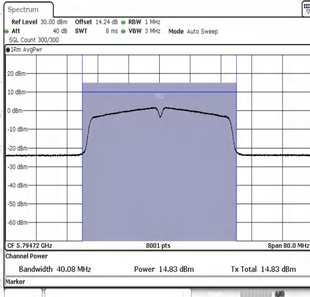
11AC40SISO-Ant1-5795-PASS
