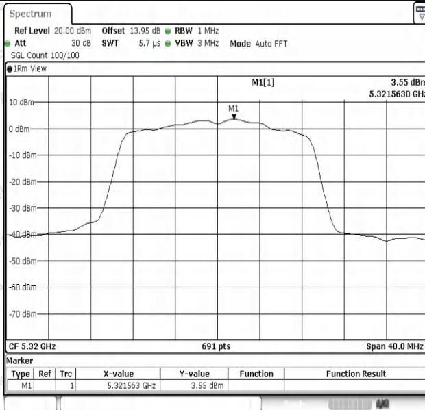
11AC20SISO-Ant1-5320-PASS
