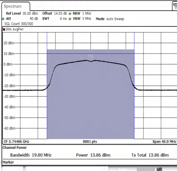
11A-Ant1-5745-PASS
