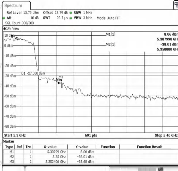
11N40SISO-Ant1-5310-PASS
