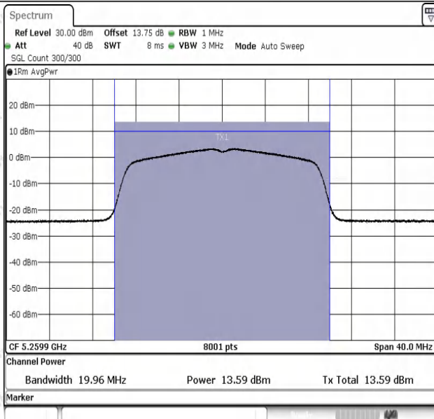
11N20SISO-Ant1-5260-PASS
