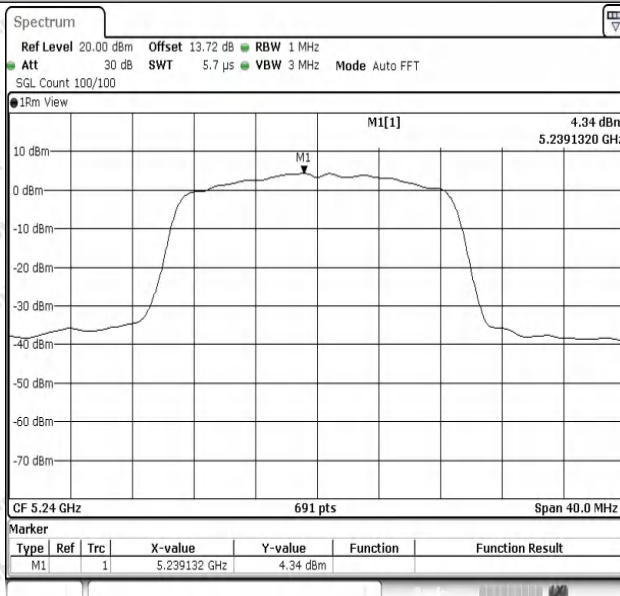
11AC20SISO-Ant1-5240-PASS
