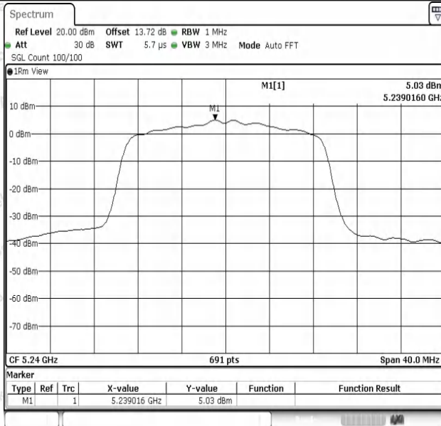
11N20SISO-Ant1-5240-PASS
