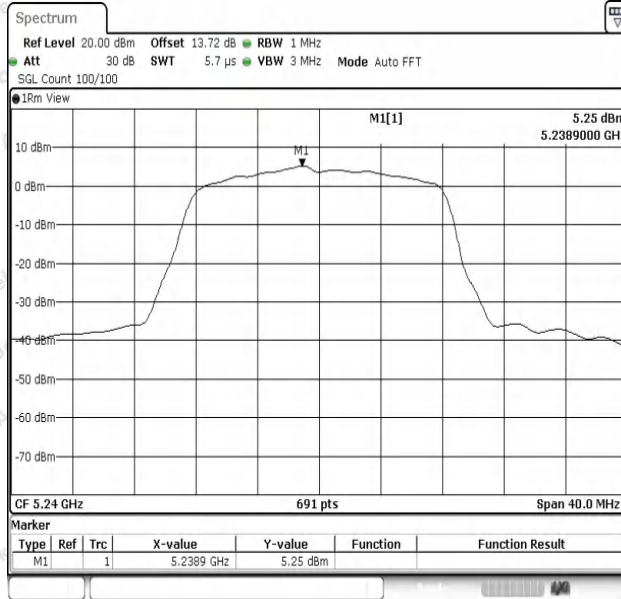
11A-Ant1-5240-PASS
