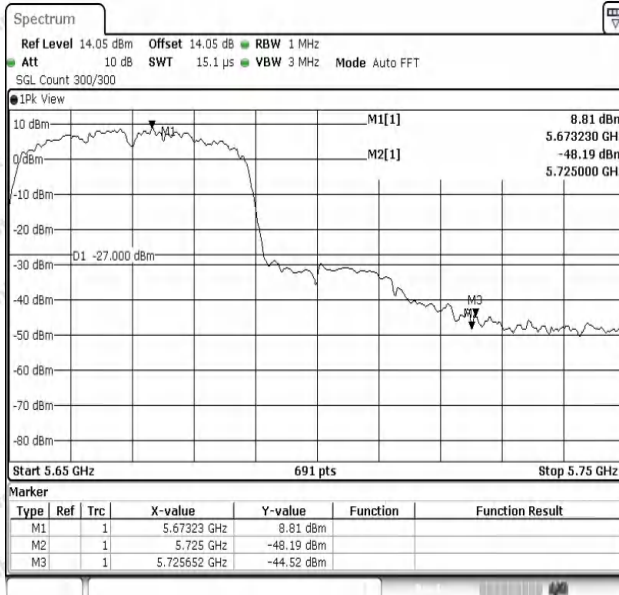
11N40SISO-Ant1-5670-PASS
