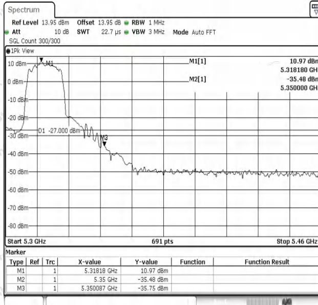
11N20SISO-Ant1-5320-PASS
