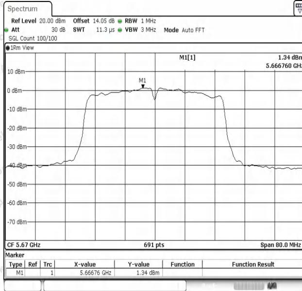
11N40SISO-Ant1-5670-PASS
