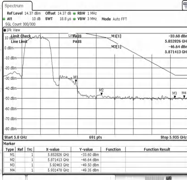
11AC20SISO-Ant1-5825-PASS
