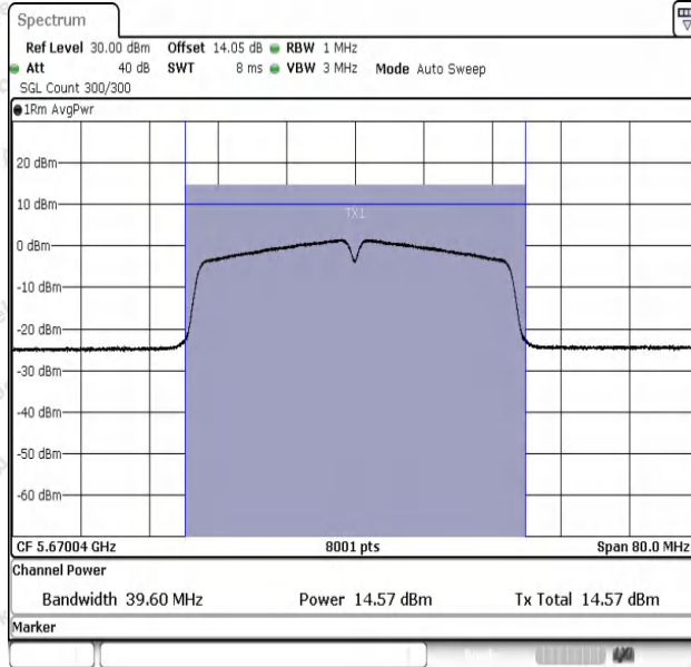
11N40SISO-Ant1-5670-PASS
