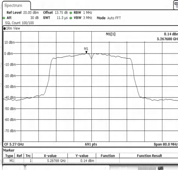
11AC40SISO-Ant1-5270-PASS
