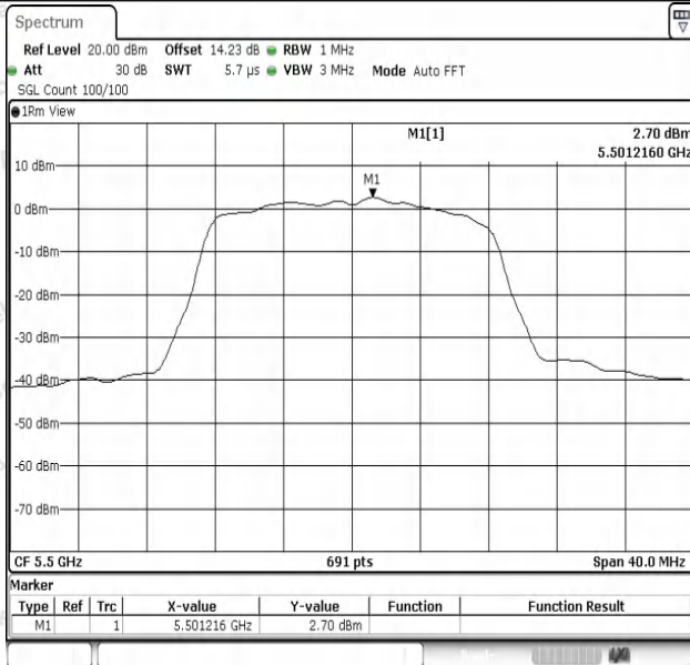
11A-Ant1-5500-PASS
