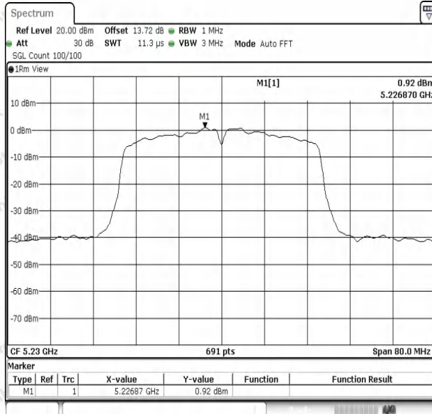
11N40SISO-Ant1-5230-PASS
