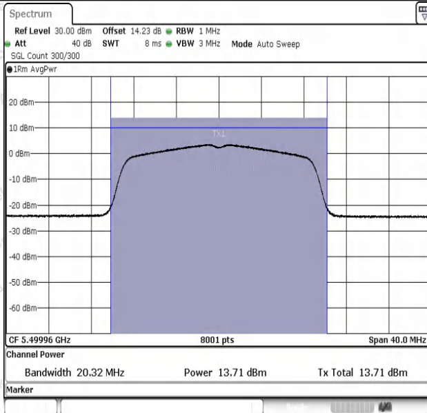
11N20SISO-Ant1-5500-PASS
