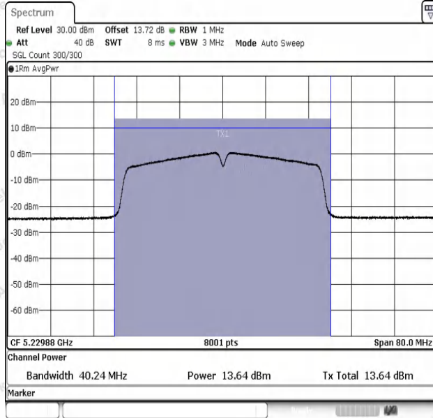
11AC40SISO-Ant1-5230-PASS
