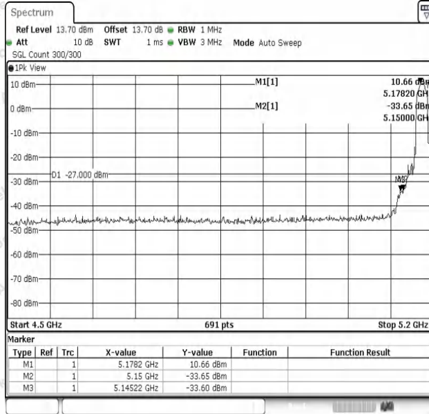
11N20SISO-Ant1-5180-PASS
