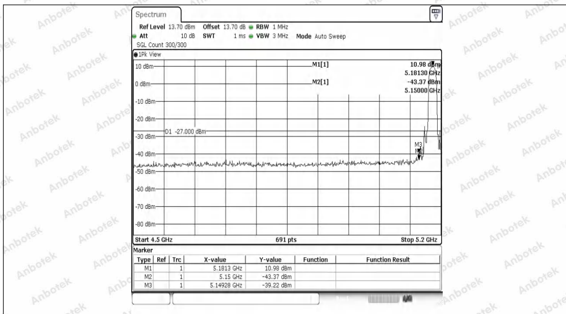
11A-Ant1-5180-PASS
