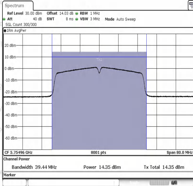
11AC40SISO-Ant1-5755-PASS
