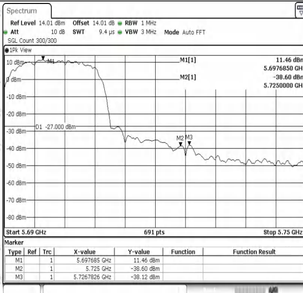
11AC20SISO-Ant1-5700-PASS
