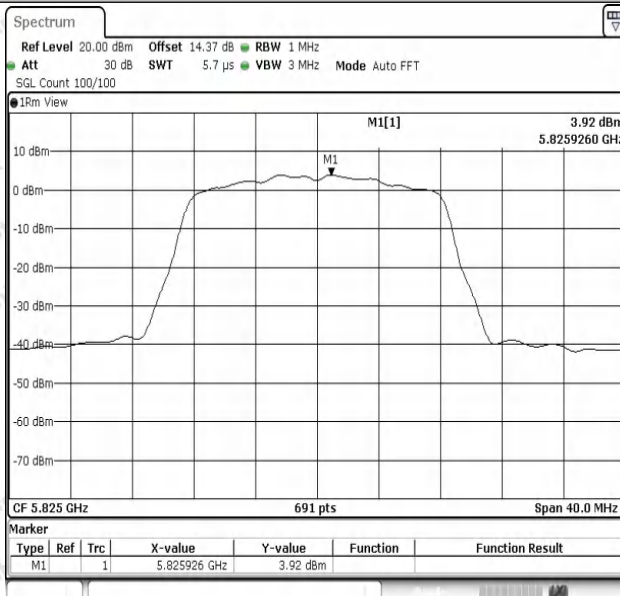
11A-Ant1-5825-PASS
