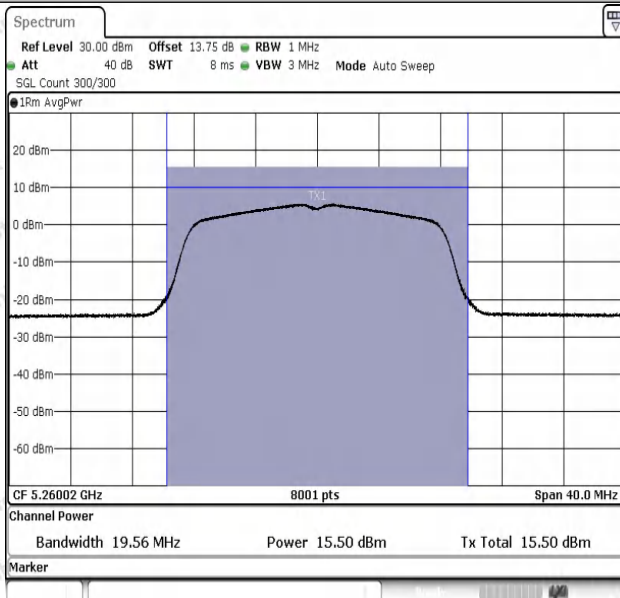
11A-Ant1-5260-PASS
