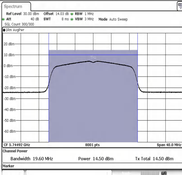
11N20SISO-Ant1-5745-PASS
