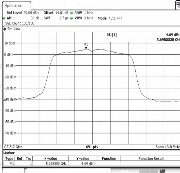
11AC20SISO-Ant1-5700-PASS
