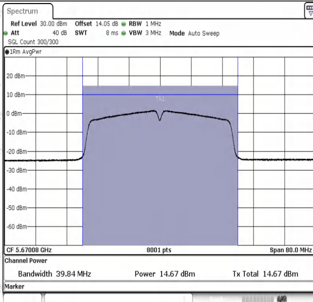
11AC40SISO-Ant1-5670-PASS
