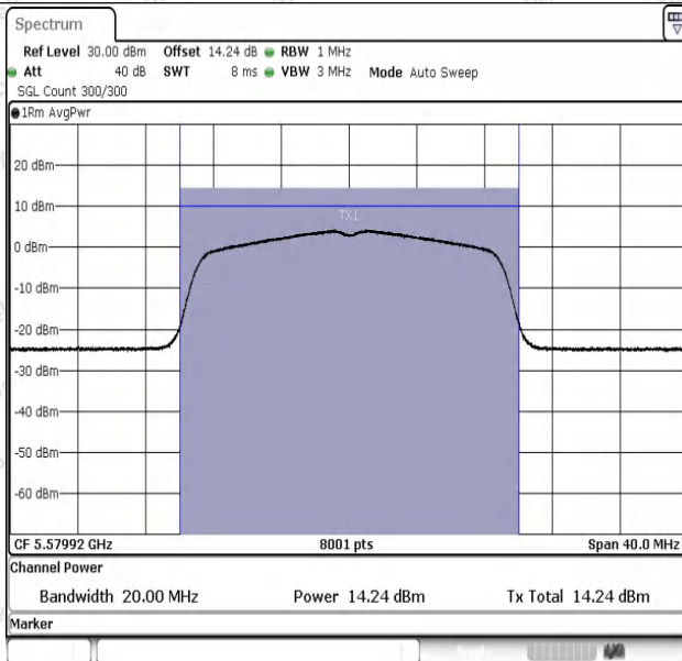
11AC20SISO-Ant1-5580-PASS
