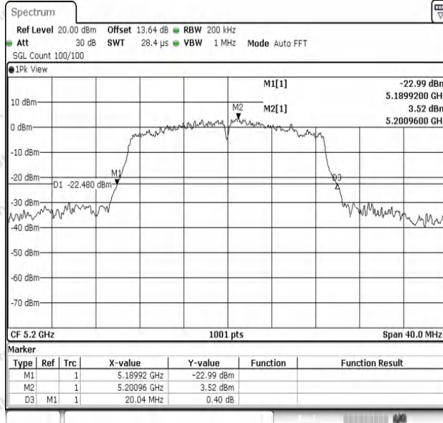
11N20SISO-Ant1-5200
