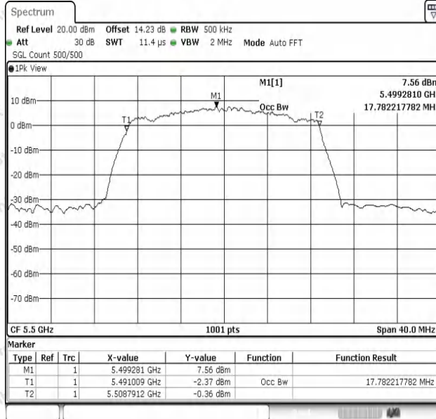
11AC20SISO-Ant1-5500
