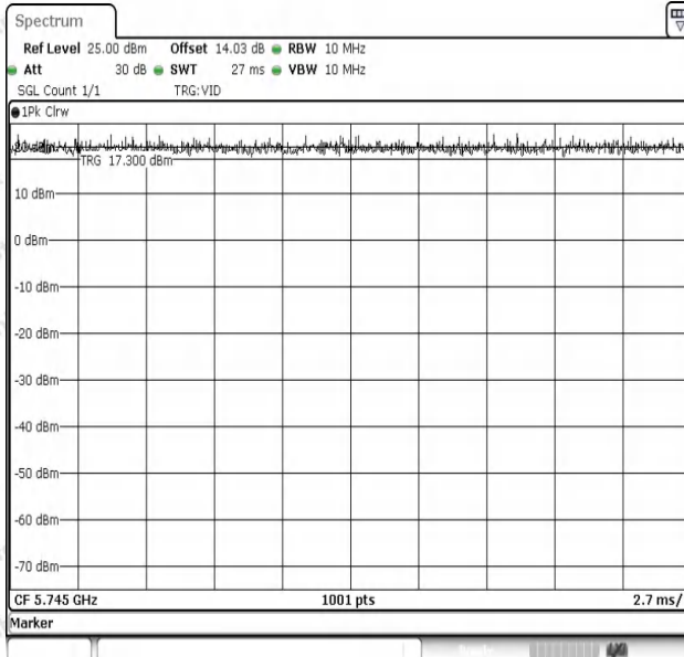
NTVN-11A-Ant1-5745
