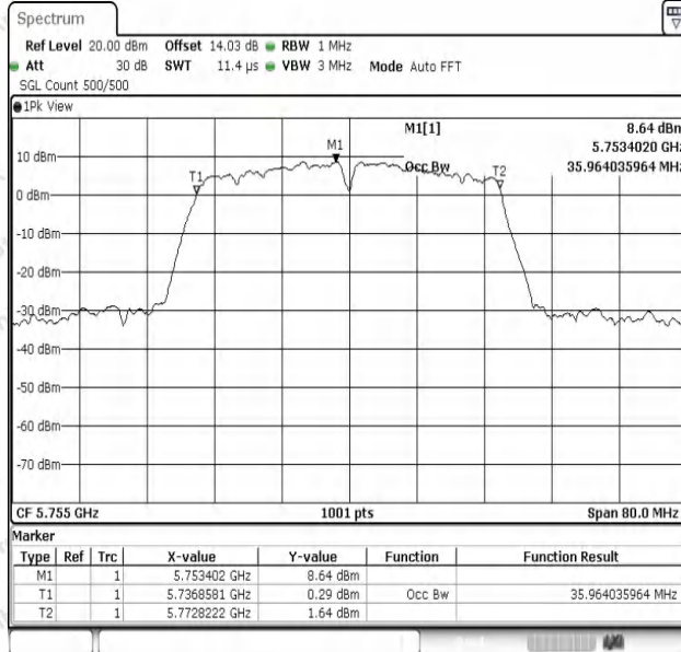
11N40SISO-Ant1-5755
