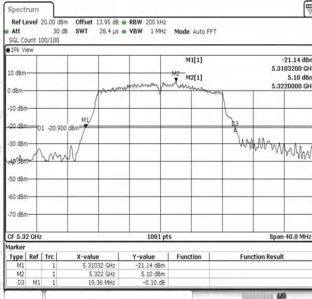
11A-Ant1-5320
