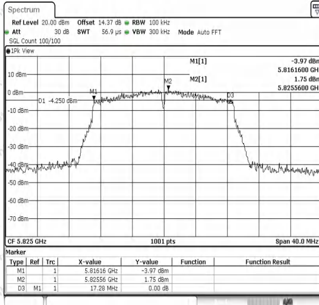
11N20SISO-Ant1-5825-PASS
