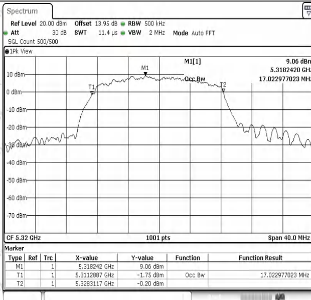
11A-Ant1-5320
