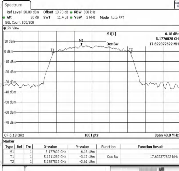
11AC20SISO-Ant1-5180
