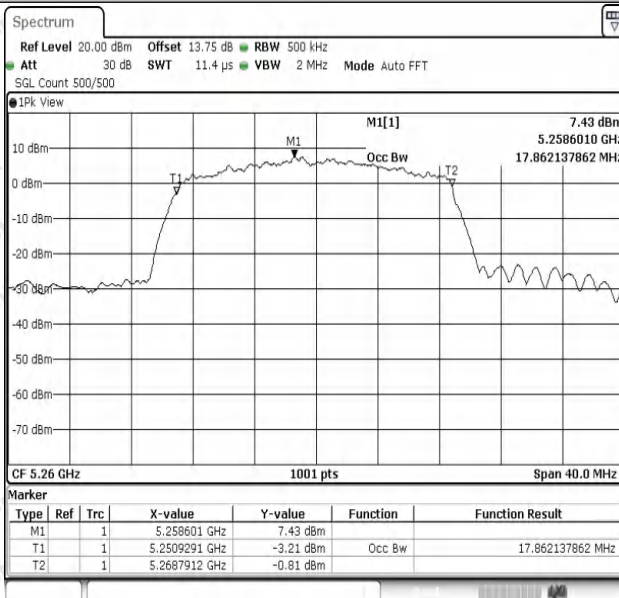
11N20SISO-Ant1-5260
