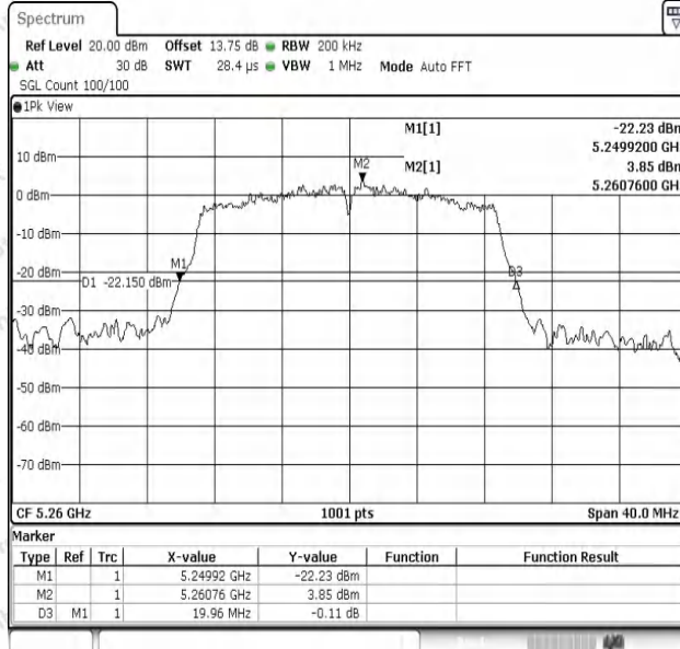
11N20SISO-Ant1-5260
