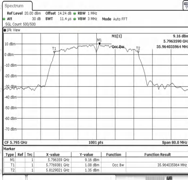
11AC40SISO-Ant1-5795
