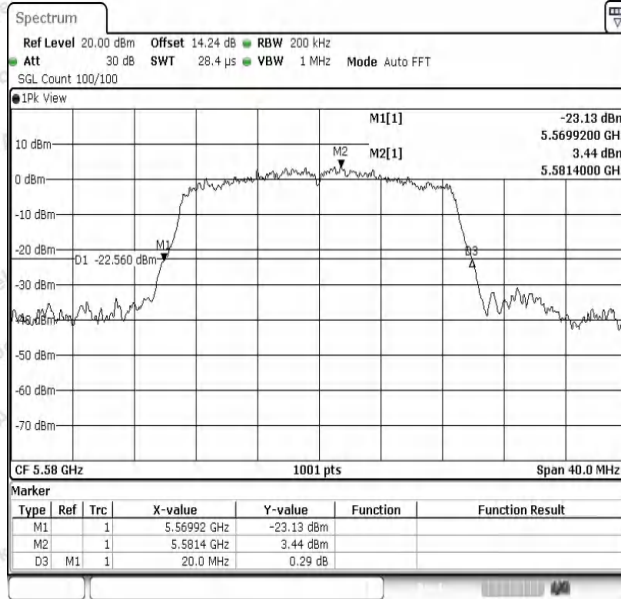
11AC20SISO-Ant1-5580
