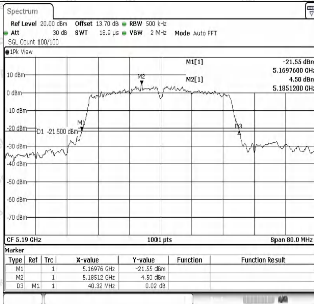
11N40SISO-Ant1-5190
