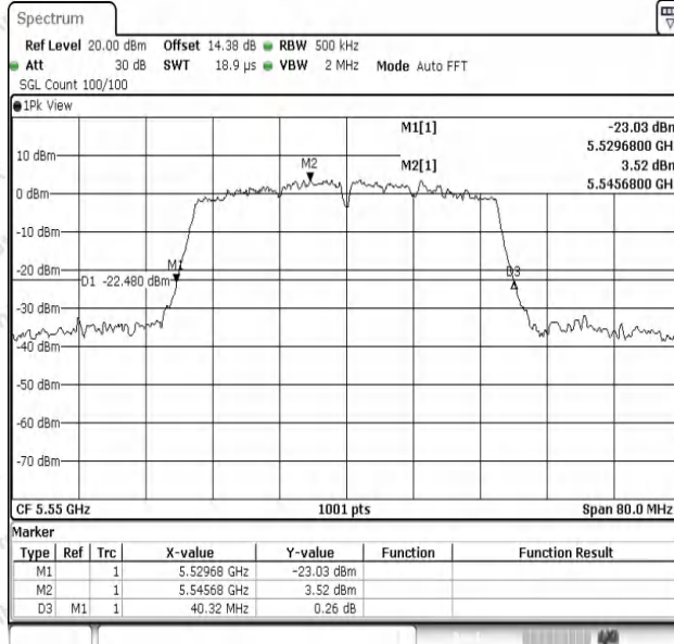
11N40SISO-Ant1-5550
