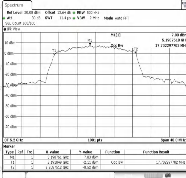
11N20SISO-Ant1-5200
