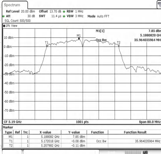
11AC40SISO-Ant1-5190
