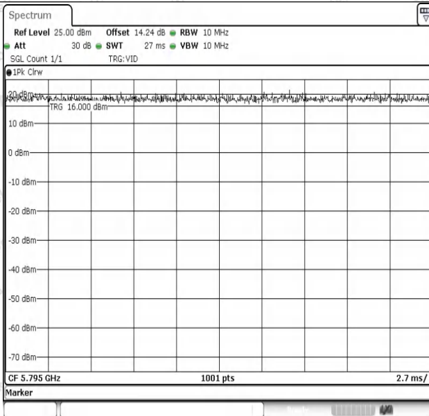
NTNV-11N40SISO-Ant1-5795
