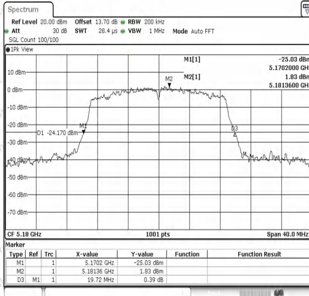
11AC20SISO-Ant1-5180
