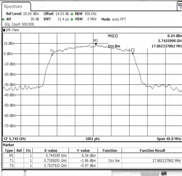
11AC20SISO-Ant1-5745
