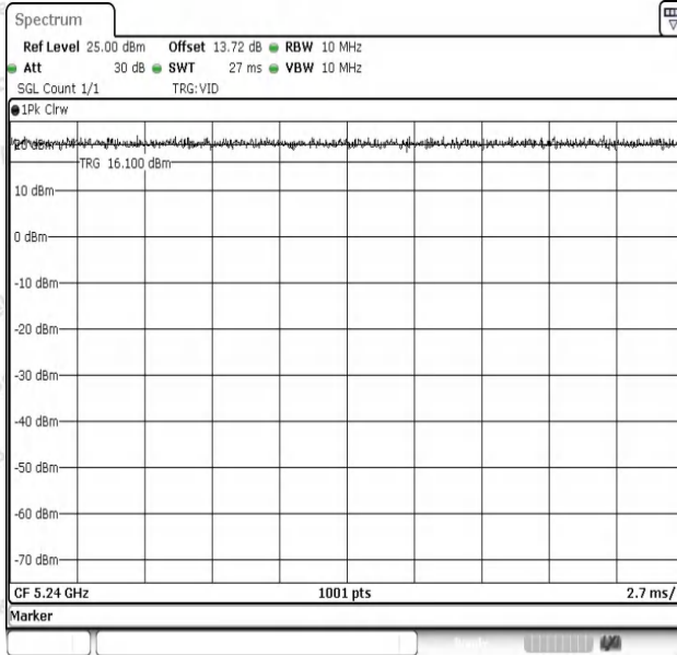
NTNV-11N20SISO-Ant1-5240
