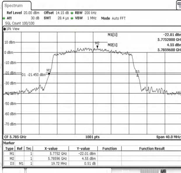
11AC20SISO-Ant1-5785
