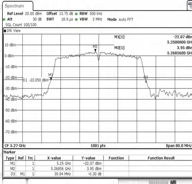
11AC40SISO-Ant1-5270
