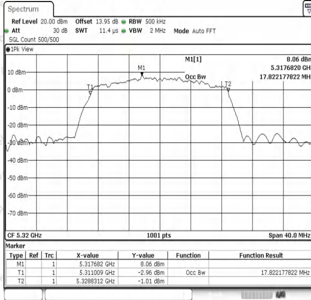
11AC20SISO-Ant1-5320
