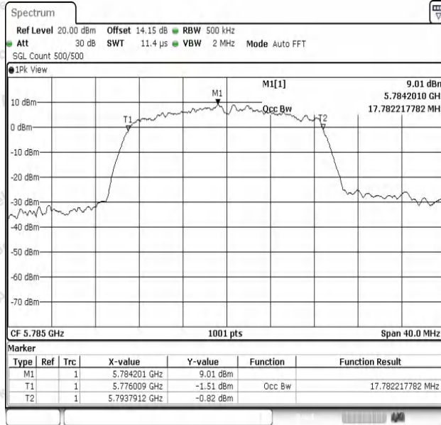
11N20SISO-Ant1-5785
