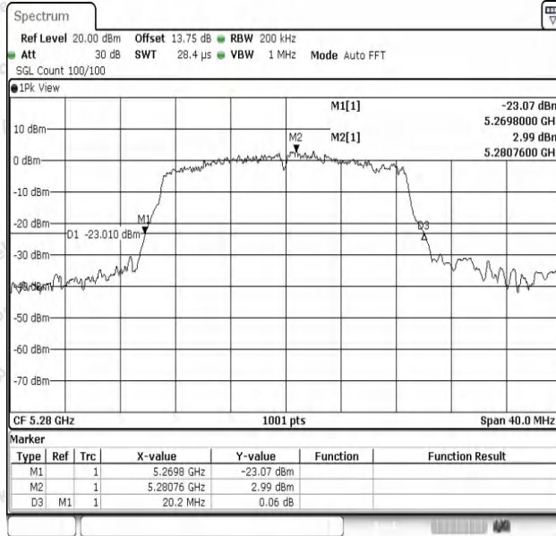
11N20SISO-Ant1-5280
