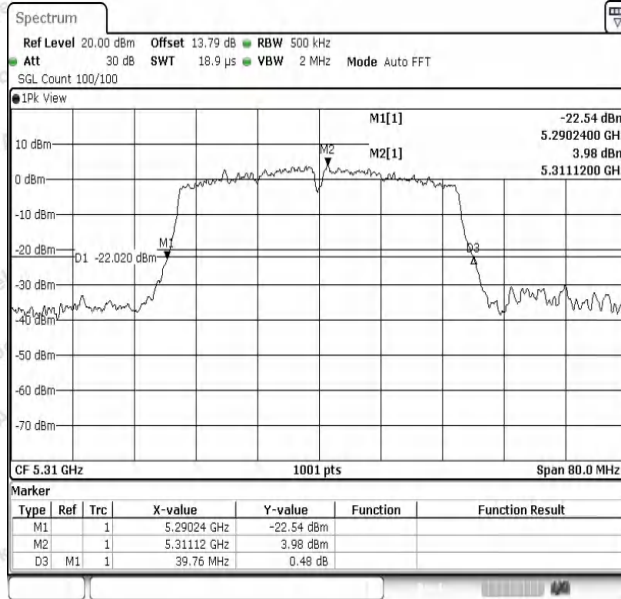
11AC40SISO-Ant1-5310
