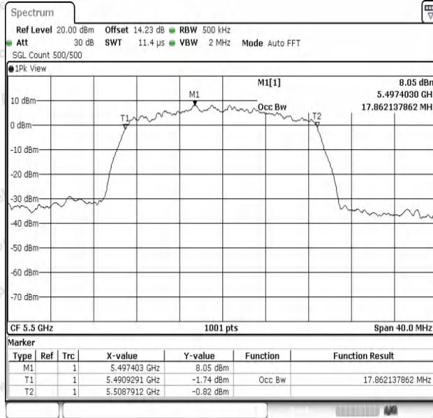
11N20SISO-Ant1-5500
