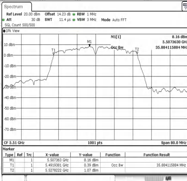
11N40SISO-Ant1-5510
