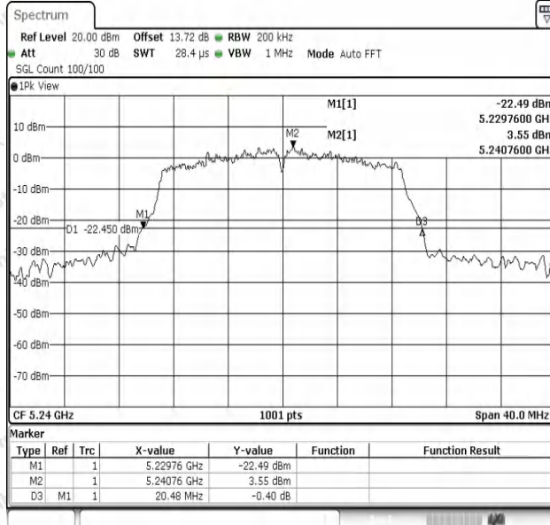
11AC20SISO-Ant1-5240
