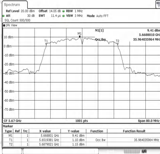
11N40SISO-Ant1-5670
