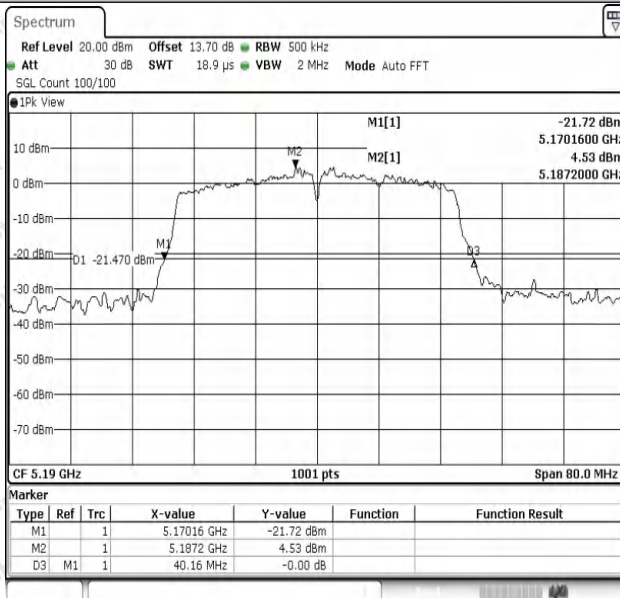
11AC40SISO-Ant1-5190
