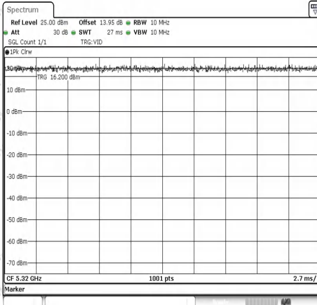
NTVN-11N20SISO-Ant1-5320
