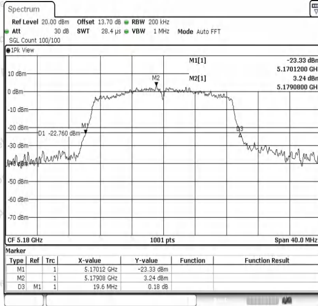
11N20SISO-Ant1-5180
