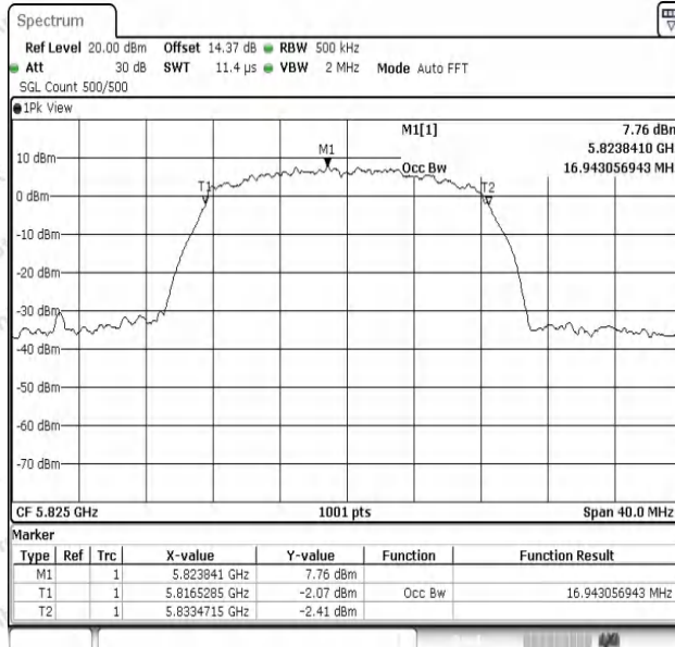
11A-Ant1-5825
