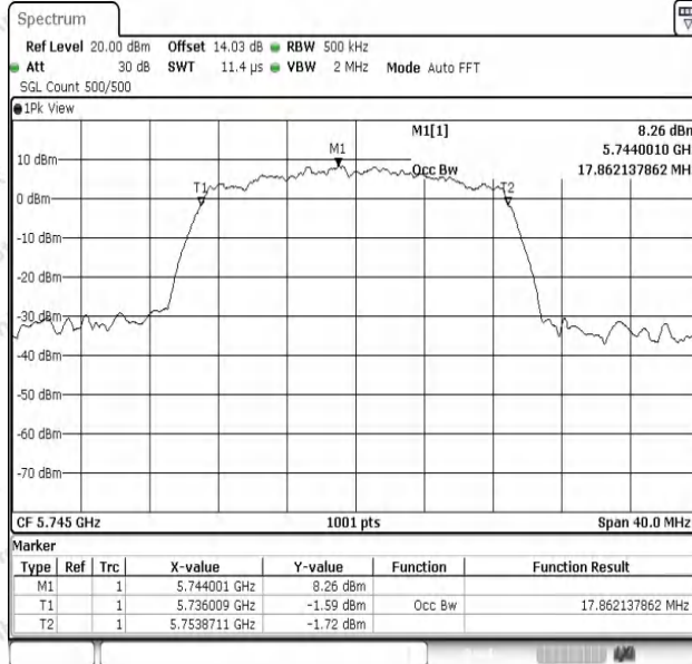
11N20SISO-Ant1-5745
