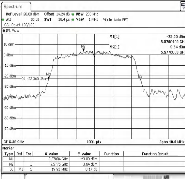
11N20SISO-Ant1-5580
