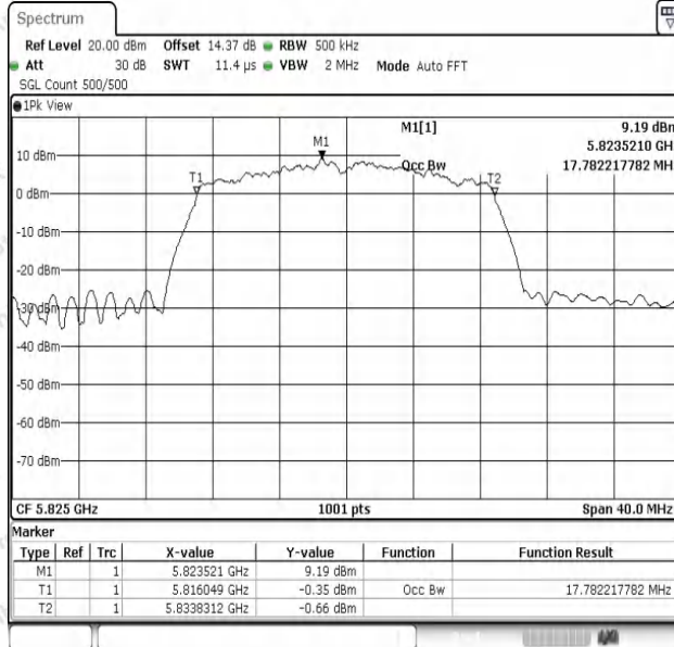
11N20SISO-Ant1-5825
