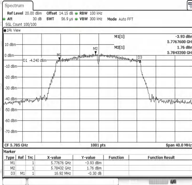
11N20SISO-Ant1-5785-PASS
