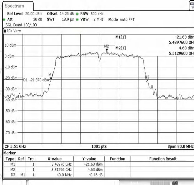
11AC40SISO-Ant1-5510
