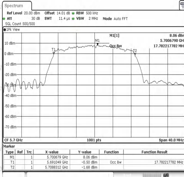
11AC20SISO-Ant1-5700
