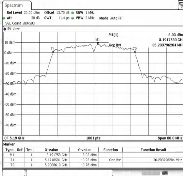
11N40SISO-Ant1-5190
