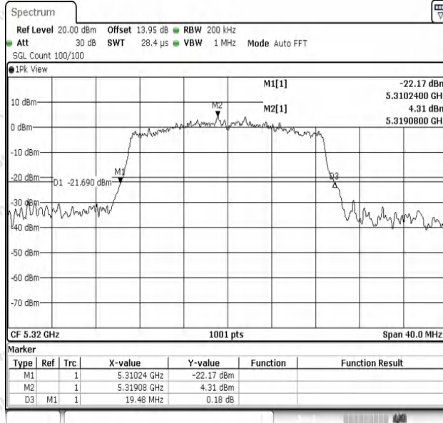
11N20SISO-Ant1-5320
