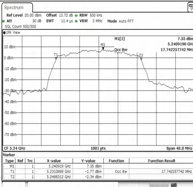
11AC20SISO-Ant1-5240
