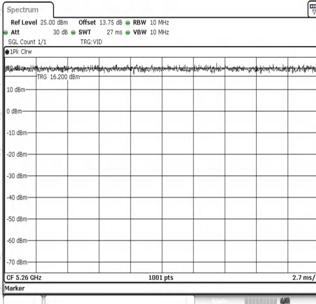
NTNV-11N20SISO-Ant1-5260
