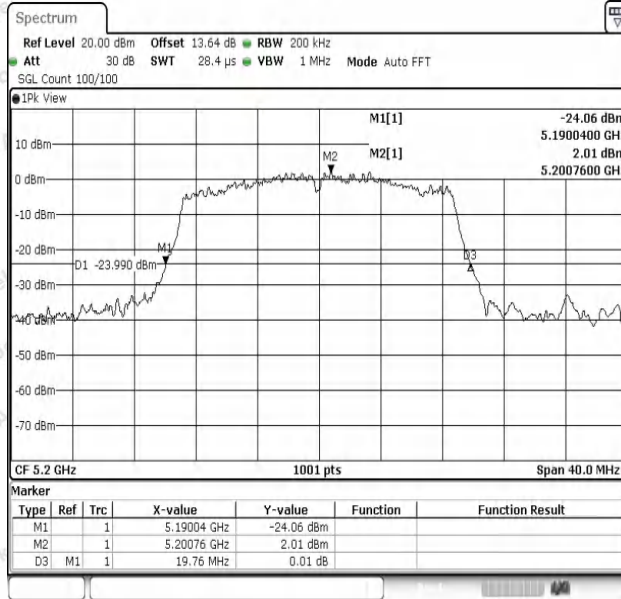
11AC20SISO-Ant1-5200
