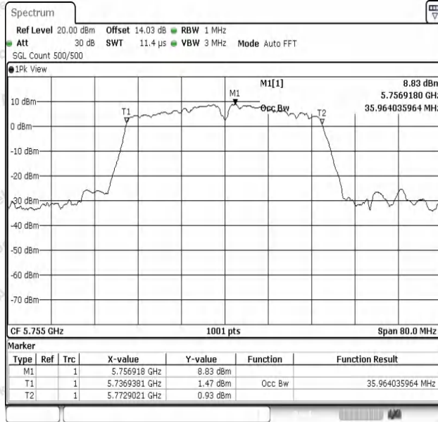
11AC40SISO-Ant1-5755
