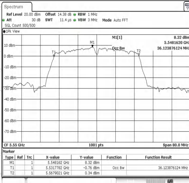
11N40SISO-Ant1-5550
