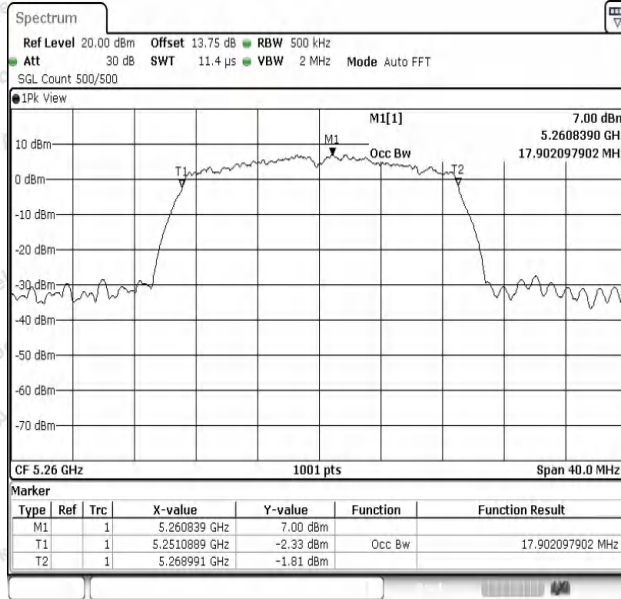
11AC20SISO-Ant1-5260
