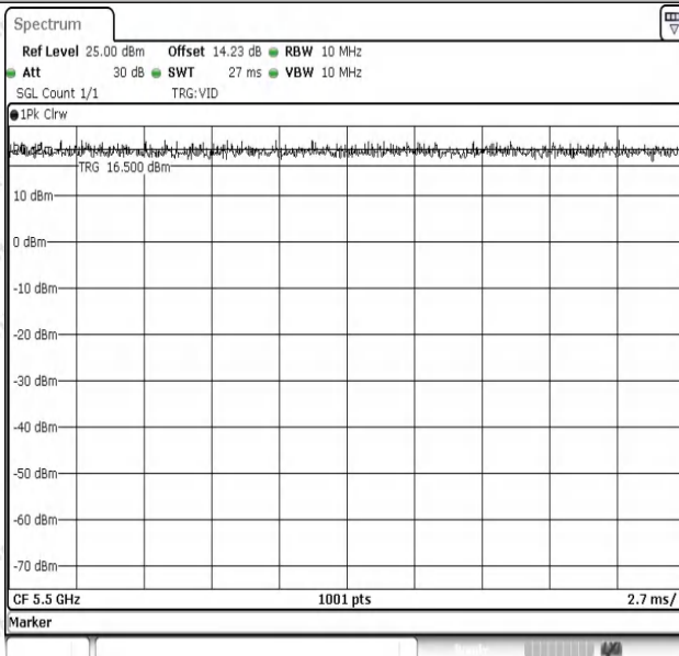
NTNV-11AC20SISO-Ant1-5500
