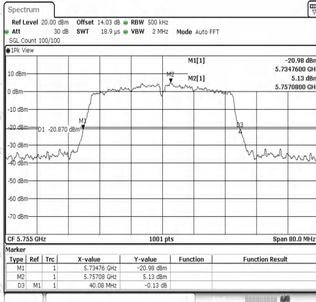
11N40SISO-Ant1-5755
