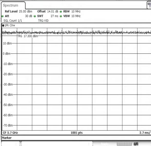
NTNV-11N20SISO-Ant1-5700
