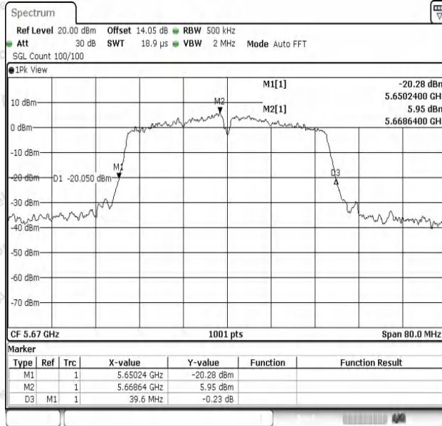
11N40SISO-Ant1-5670
