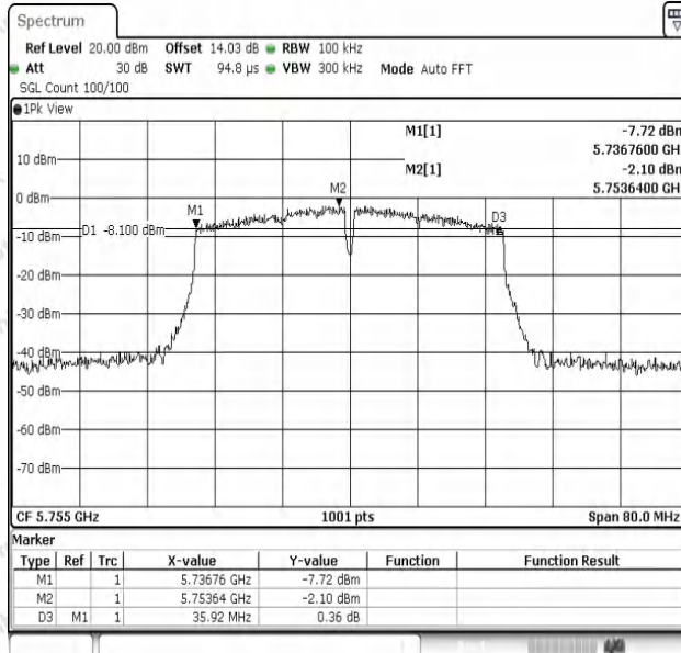
11AC40SISO-Ant1-5755-PASS
