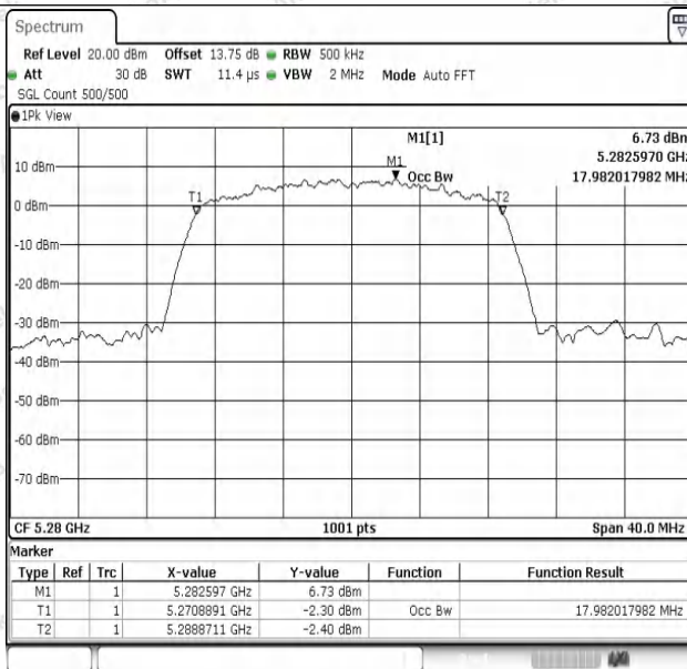
11N20SISO-Ant1-5280
