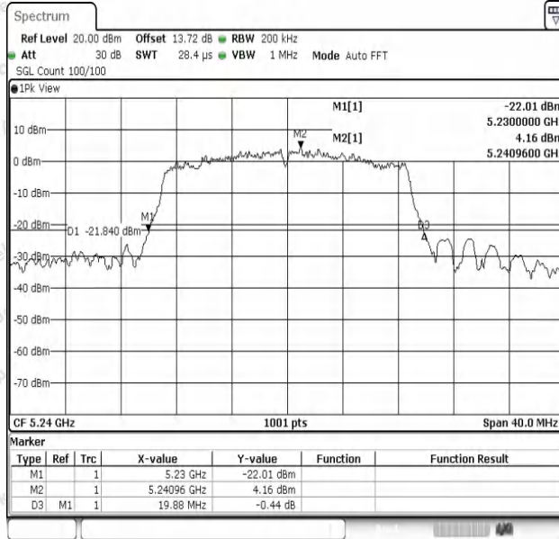
11N20SISO-Ant1-5240
