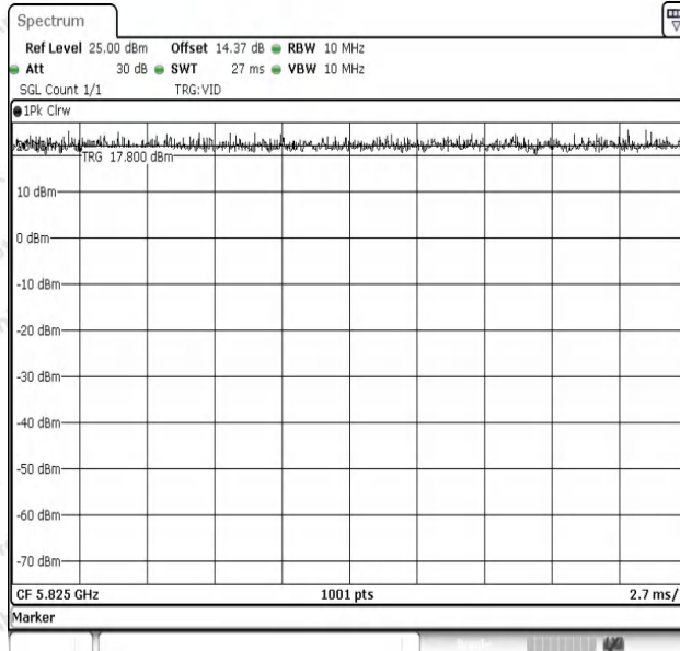
NTVN-11A-Ant1-5825
