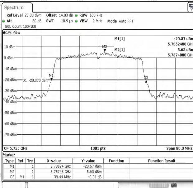
11AC40SISO-Ant1-5755
