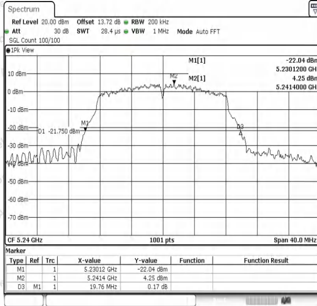
11A-Ant1-5240
