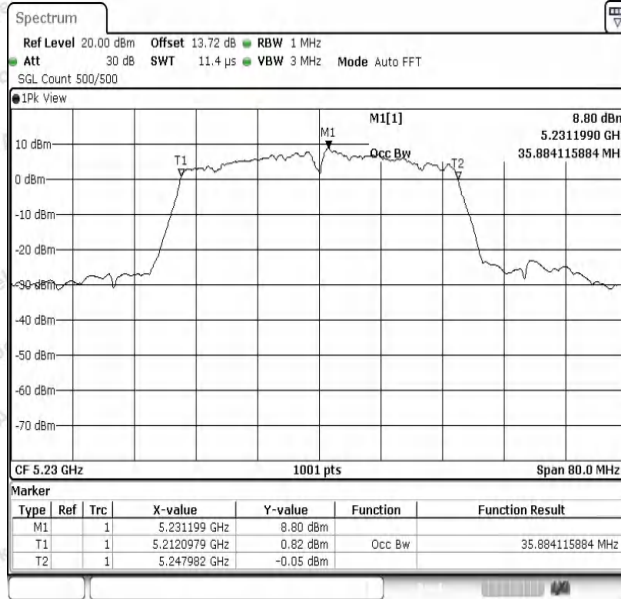
11AC40SISO-Ant1-5230
