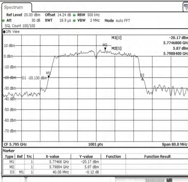
11AC40SISO-Ant1-5795
