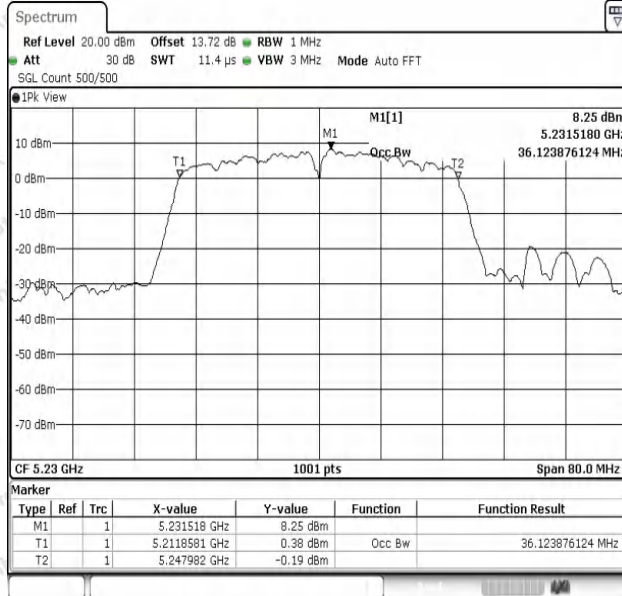
11N40SISO-Ant1-5230
