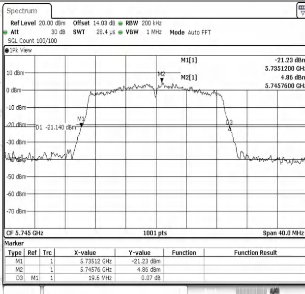
11N20SISO-Ant1-5745
