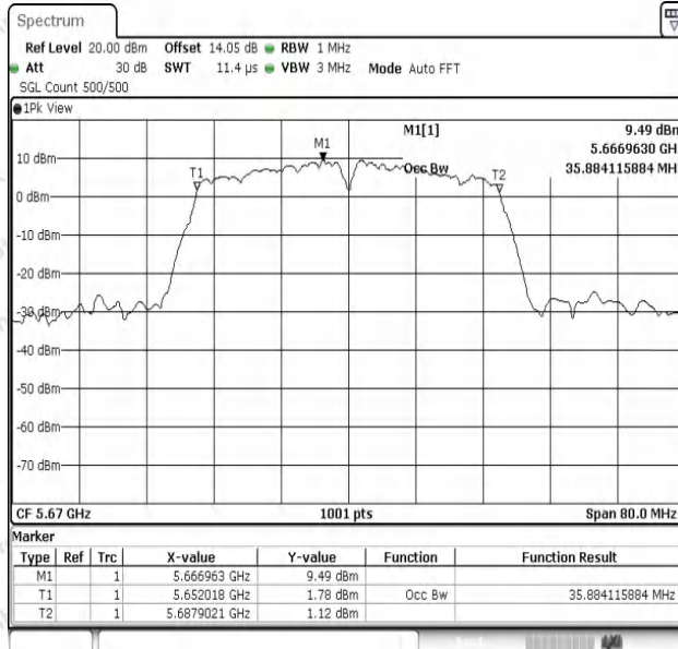
11AC40SISO-Ant1-5670
