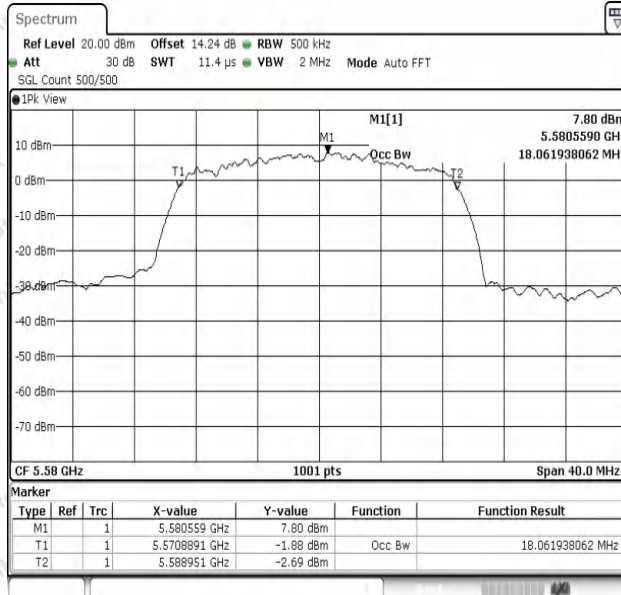
11N20SISO-Ant1-5580
