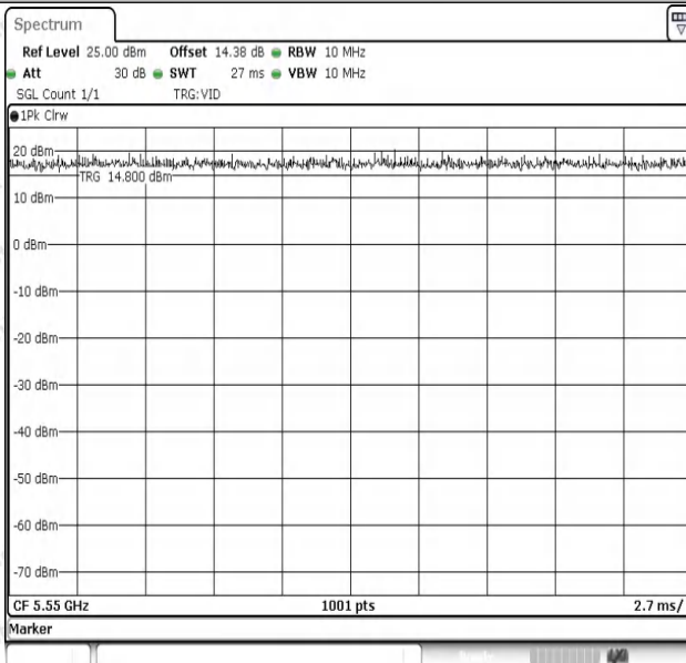
NTNV-11N40SISO-Ant1-5550
