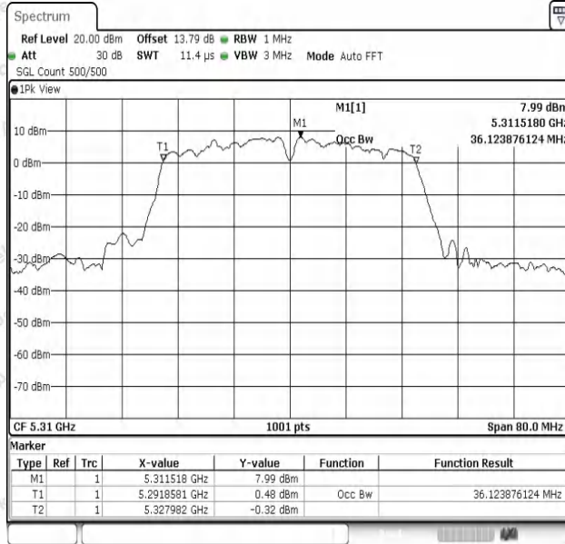
11AC40SISO-Ant1-5310
