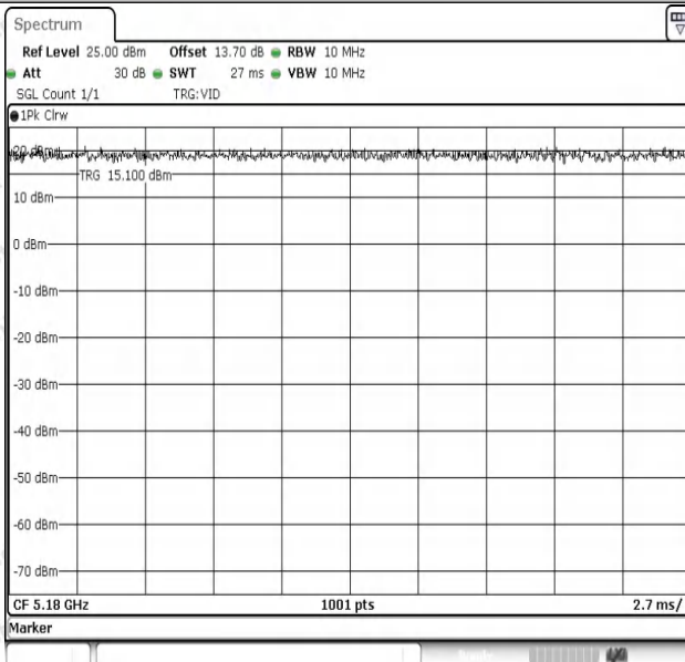
NTNV-11AC20SISO-Ant1-5180
