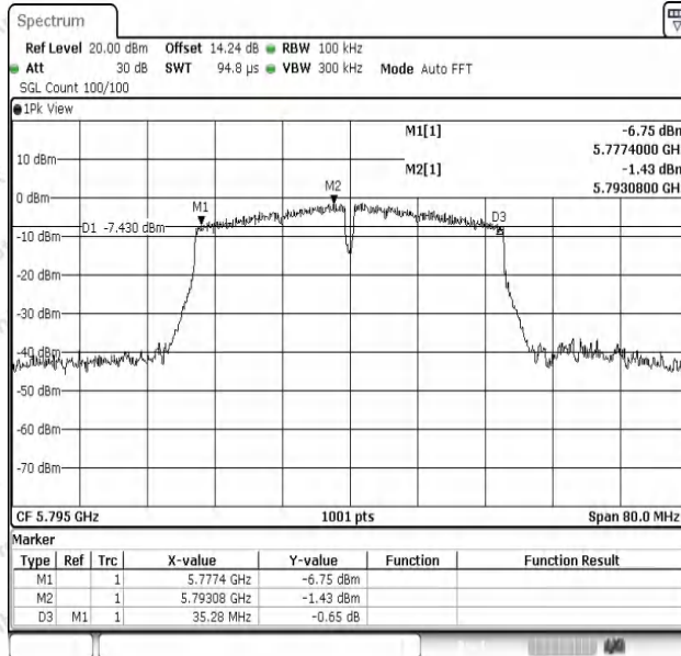
11N40SISO-Ant1-5795-PASS
