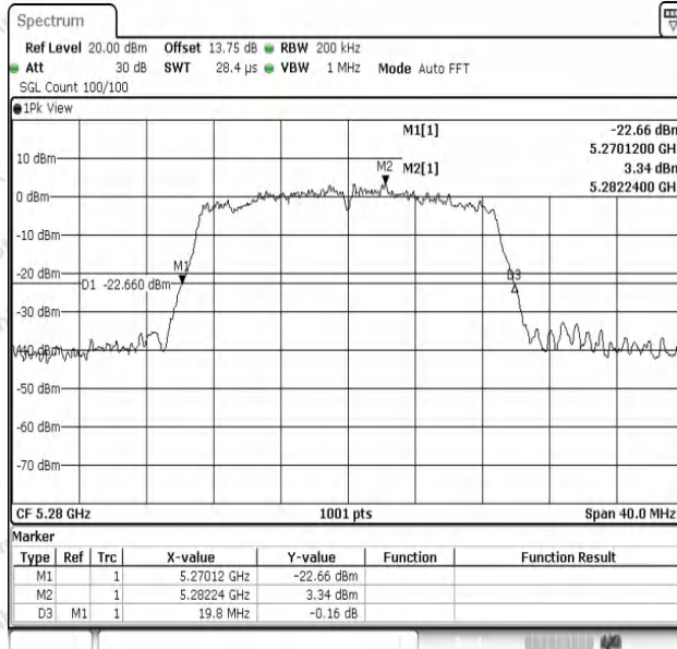
11AC20SISO-Ant1-5280
