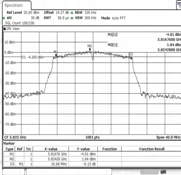
11AC20SISO-Ant1-5825-PASS
