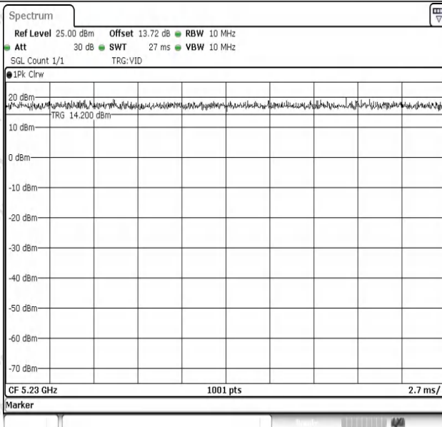
NTNV-11N40SISO-Ant1-5230
