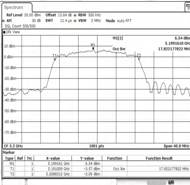
11AC20SISO-Ant1-5200
