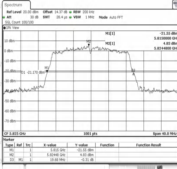
11N20SISO-Ant1-5825
