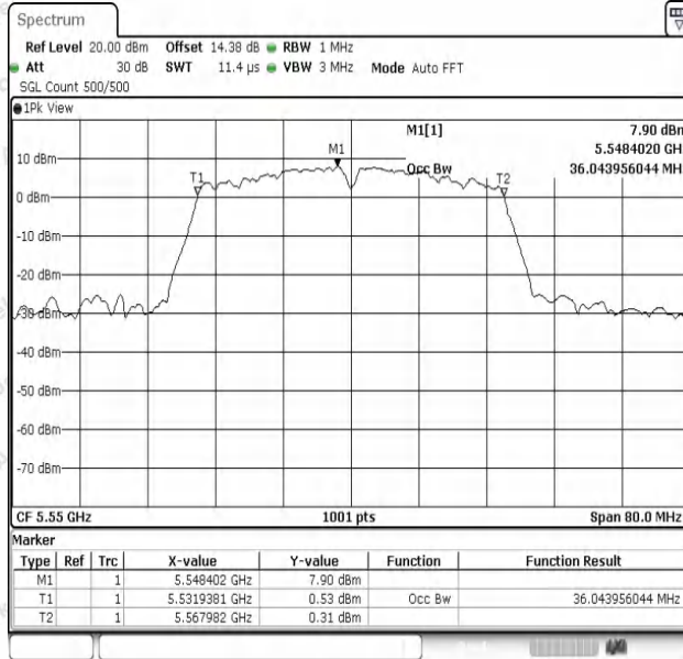
11AC40SISO-Ant1-5550
