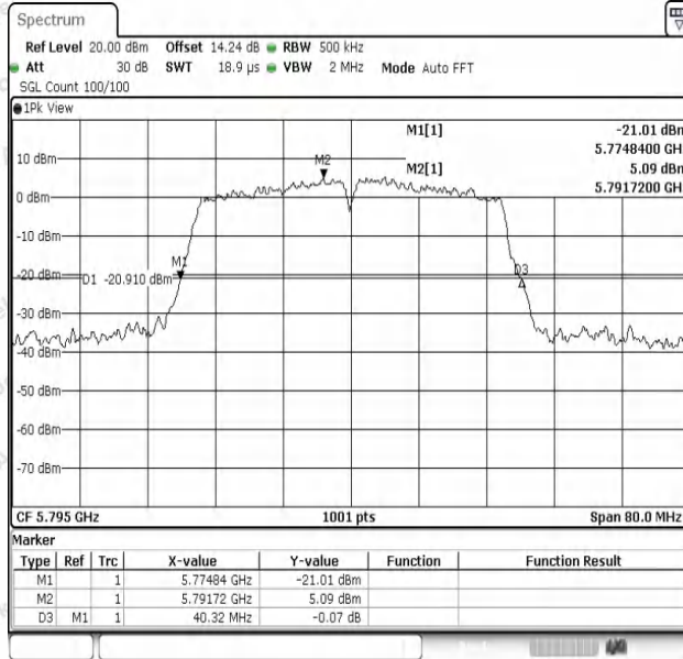
11N40SISO-Ant1-5795
