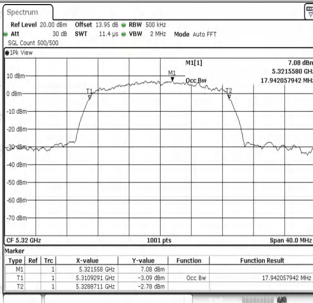
11N20SISO-Ant1-5320
