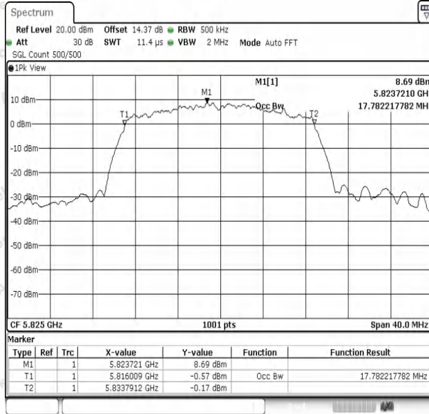
11AC20SISO-Ant1-5825
