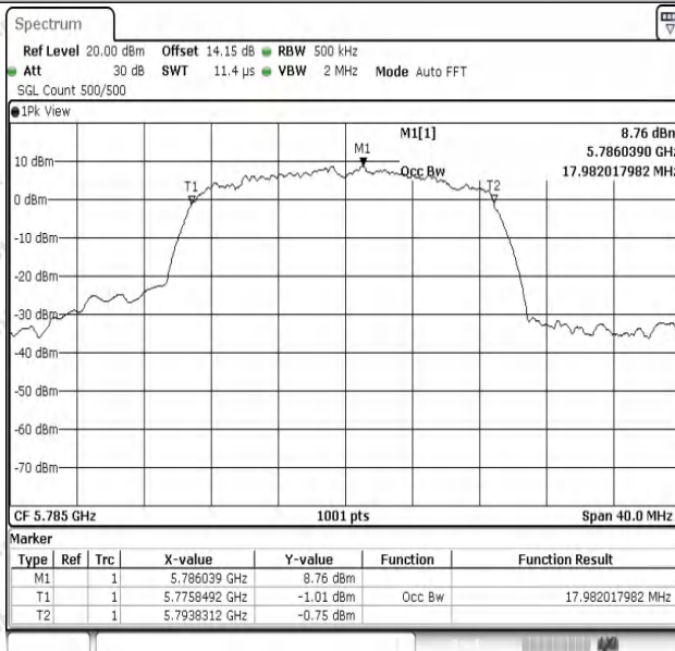
11AC20SISO-Ant1-5785
