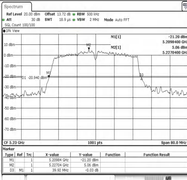
11N40SISO-Ant1-5230
