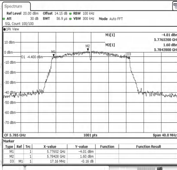
11AC20SISO-Ant1-5785-PASS
