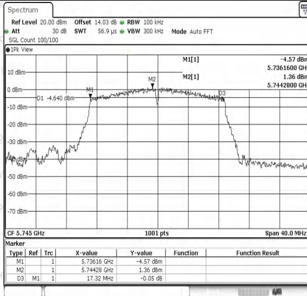
11AC20SISO-Ant1-5745-PASS
