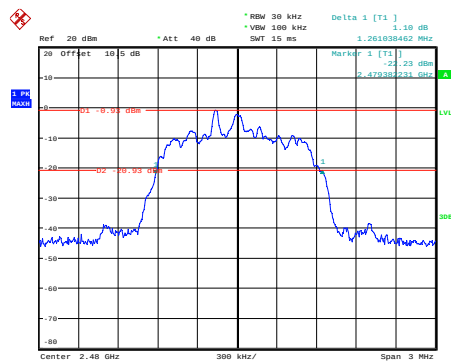
\pi/4 -DQPSK_High_2DH1
