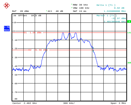
8DPSK_Low_3DH1
