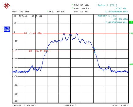
8DPSK_High_3DH1
