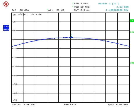
\pi/4 -DQPSK_High_2DH1
