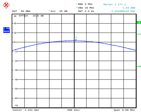
8DPSK_Mid_3DH1
