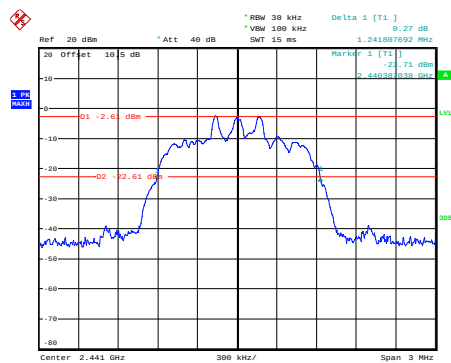
8DPSK_Mid_3DH1
