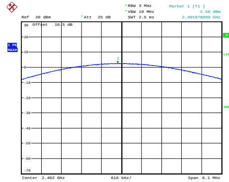
8DPSK_Low_3DH1
