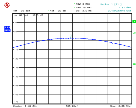
8DPSK_High_3DH1
