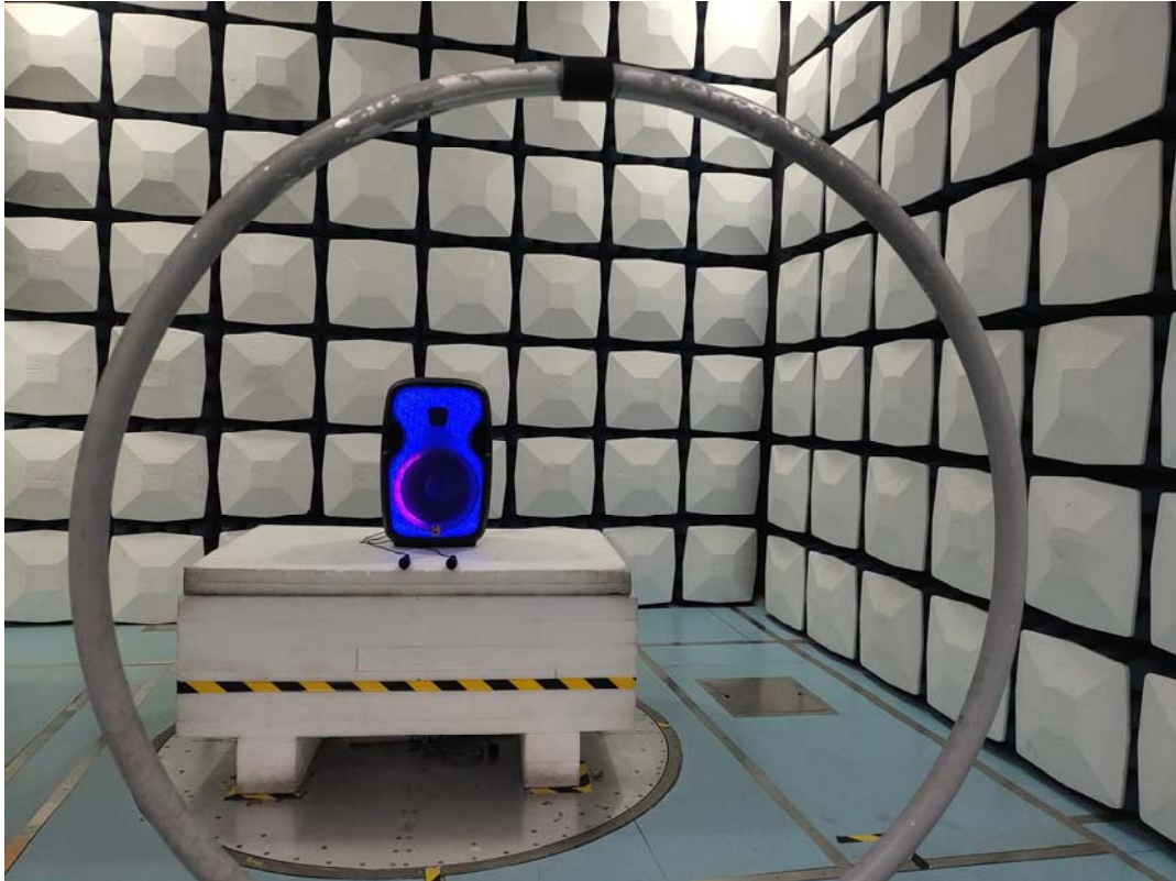
Radiated Emission 9k-30MHz Perpendicular View-AC
