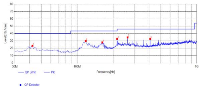
Suspected List
