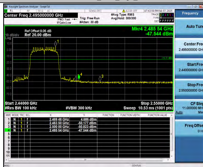
11AX20SISO_Ant0_High_2462
