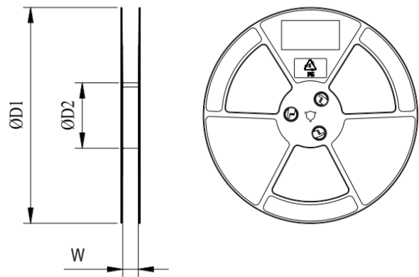
Figure 7-3-2 Tape dimension
