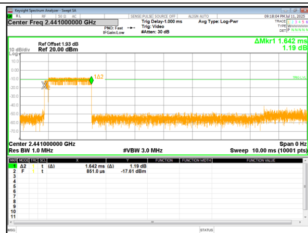
2DH5-2441MHz-One burst
