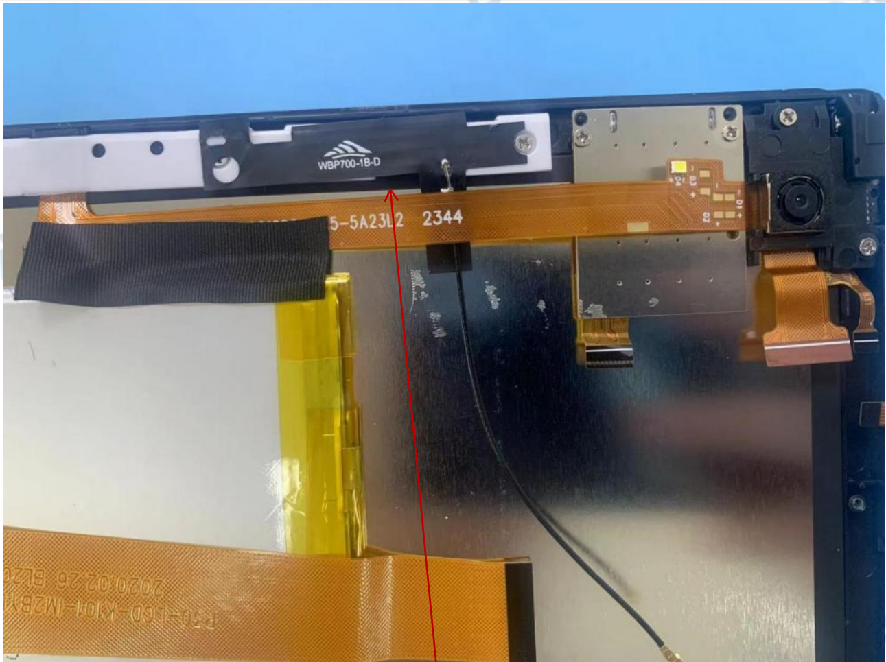
WIFI-ANT
