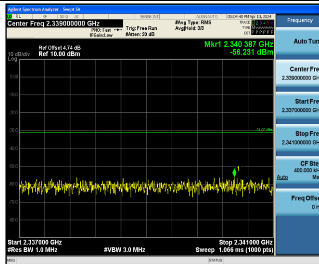
Band40-5MHz-16QAM-38725-1RB#0-Range11:2341~2345MHz
