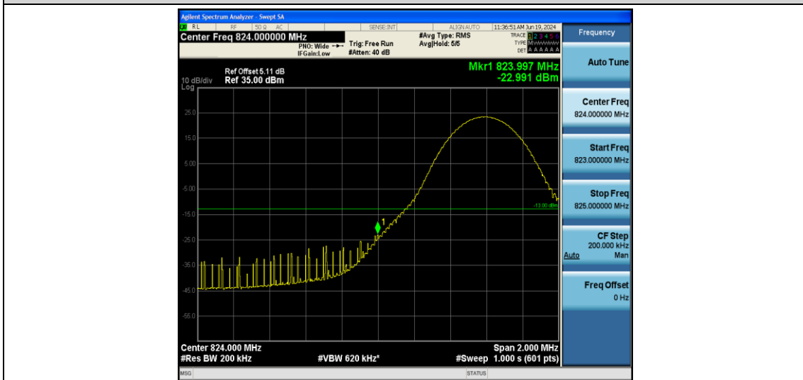
Band26-10MHz-QPSK-26840-1RB#49
