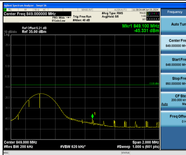
Band26-10MHz-QPSK-26990-1RB#49
