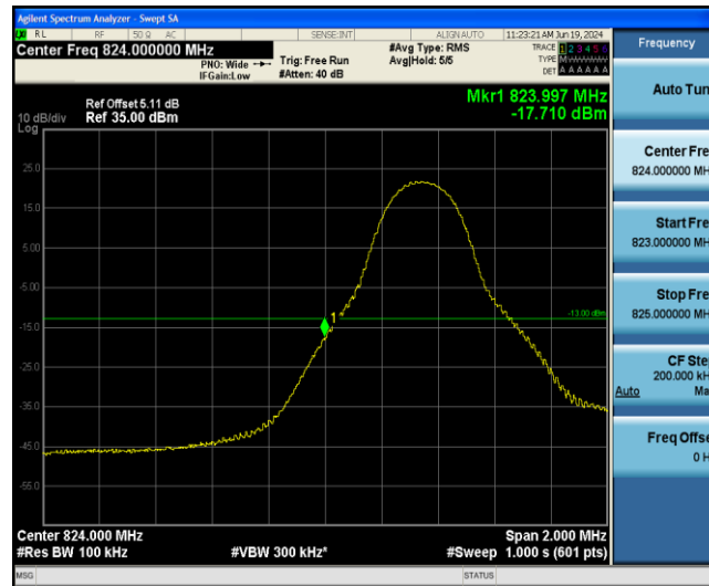
Band26-5MHz-16QAM-26815-1RB#24
