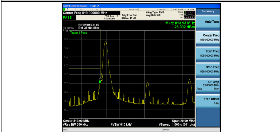
Band26-15MHz-16QAM-26765-1RB#74
