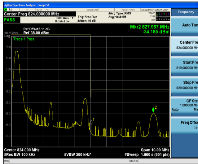
Band26-5MHz-QPSK-26765-1RB#24
