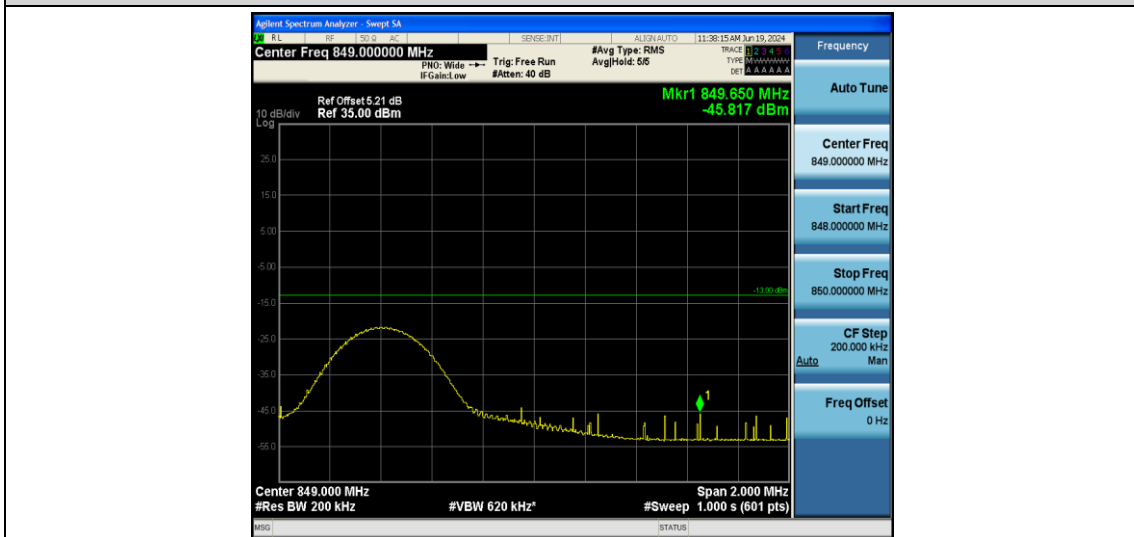
Band26-10MHz-16QAM-26990-1RB#49
