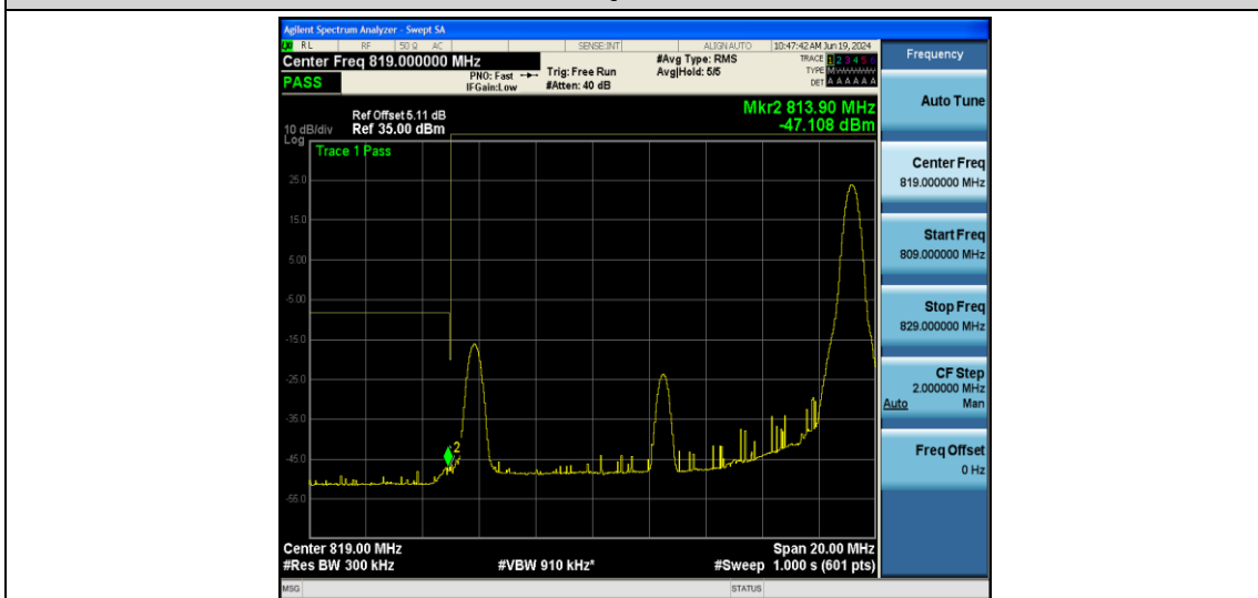
Band26-15MHz-QPSK-26765-75RB#0
