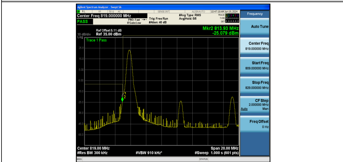
Band26-15MHz-QPSK-26765-1RB#74
