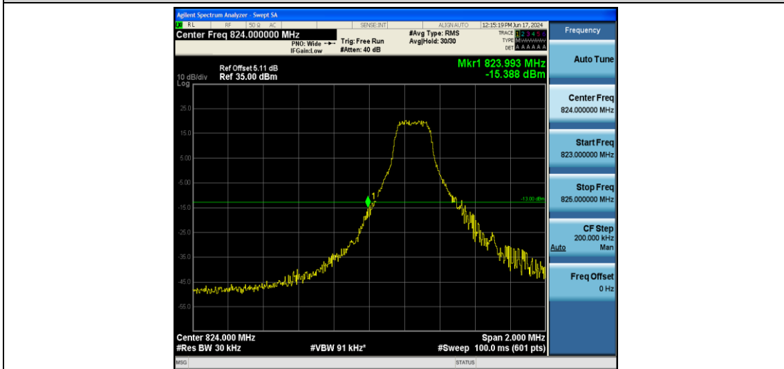
Band5-1.4MHz-16QAM-20407-1RB#5
