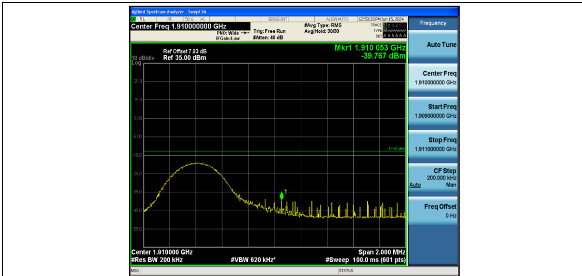
Band2-10MHz-16QAM-19150-1RB#49
