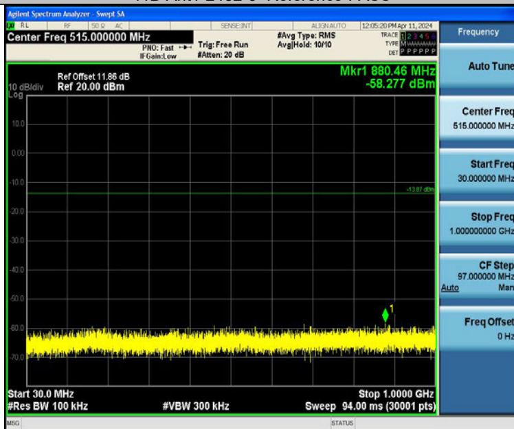
11B-Ant1-2462-30~1000-PASS
