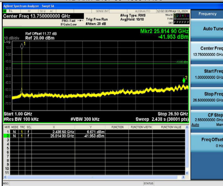
11B-Ant1-2437-1000~26500-PASS
