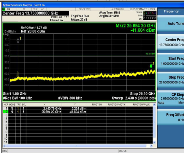
11N20SISO-Ant1-2437-1000~26500-PASS
