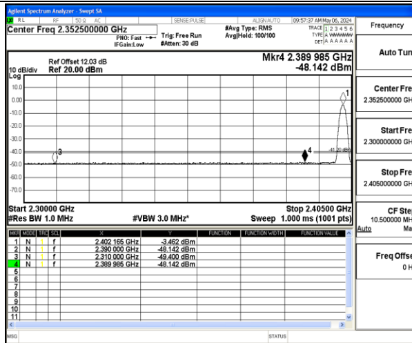
3DH5-Ant1-2402-PASS
