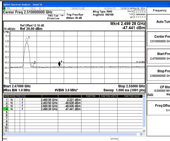
3DH5-Ant1-2480-PASS
