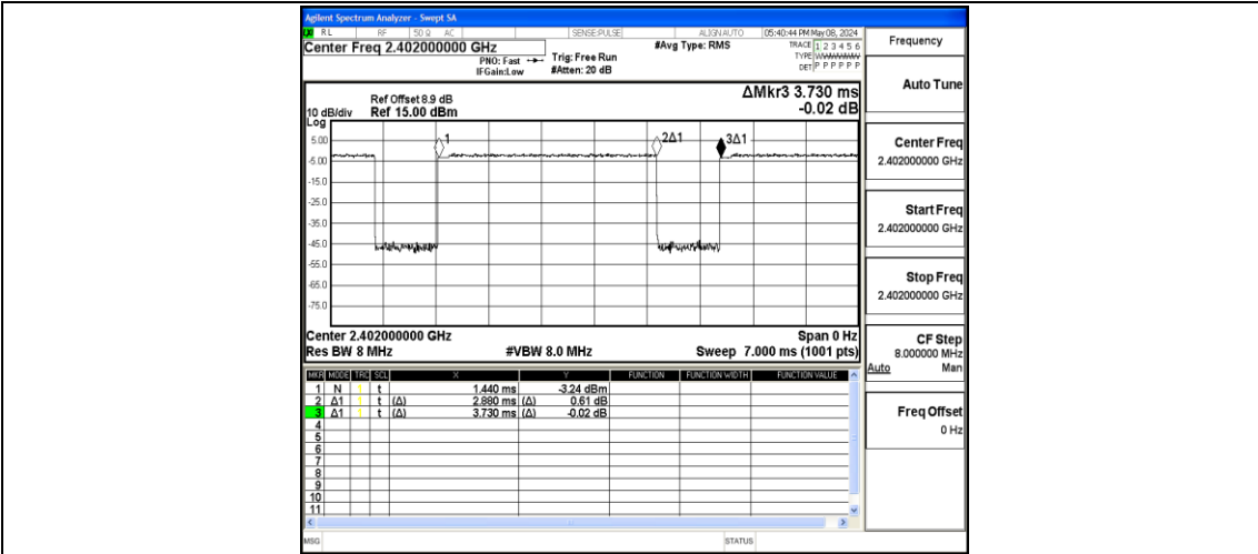
NTNV-3DH5-Ant1-2402
