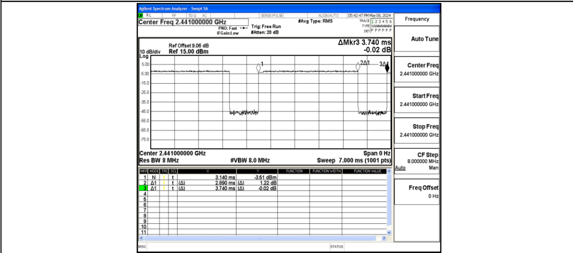
NTNV-3DH5-Ant1-2441
