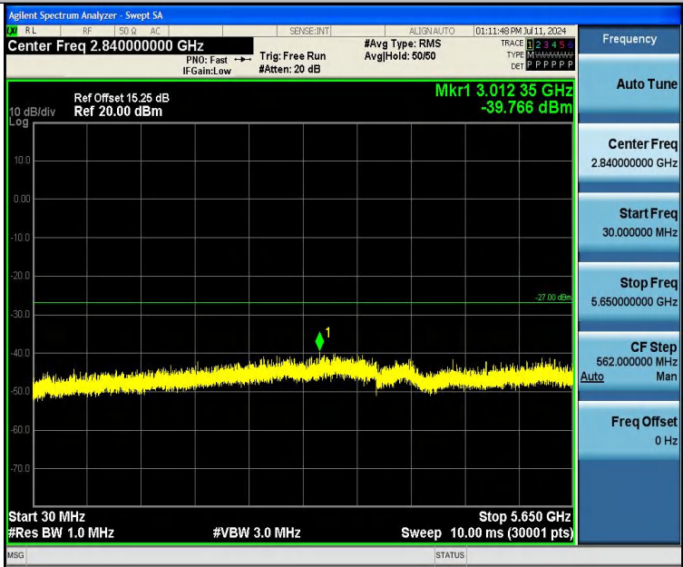
11AC20SISO-Ant1-5745-30~5650-PASS
