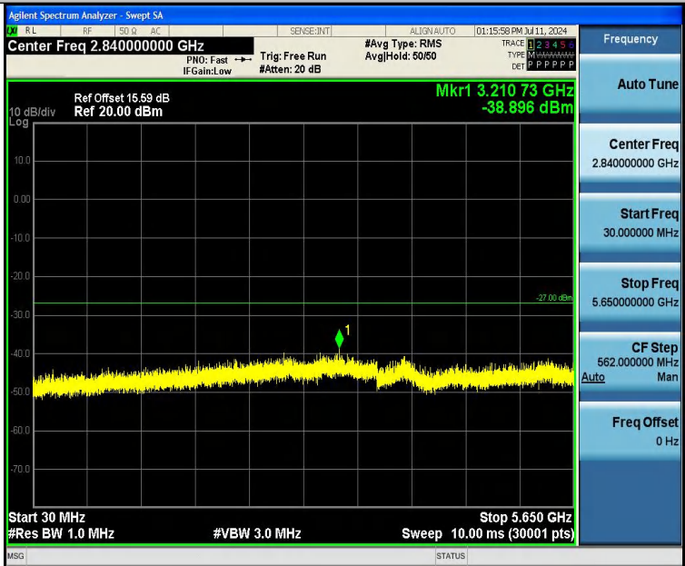
11AC20SISO-Ant1-5825-30~5650-PASS
