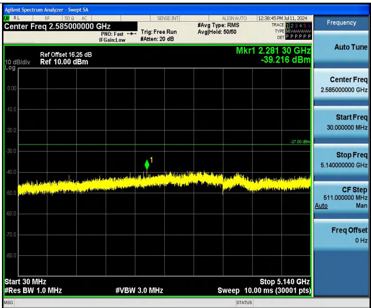
11N20SISO-Ant1-5180-30~5140-PASS
