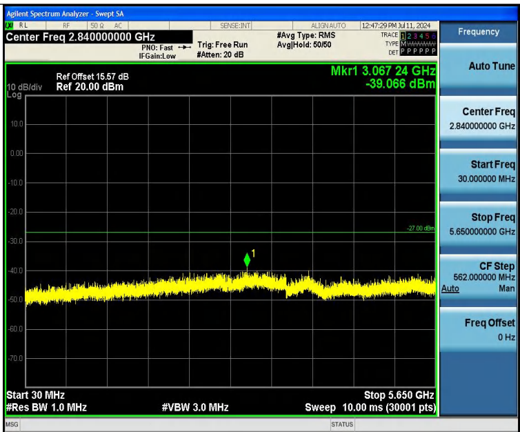
11N20SISO-Ant1-5785-30~5650-PASS
