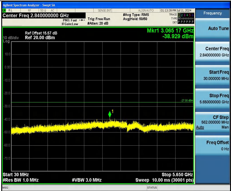
11AC20SISO-Ant1-5785-30~5650-PASS
