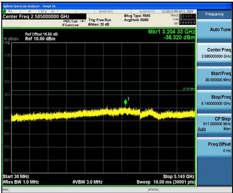
11A-Ant1-5240-30~5140-PASS
