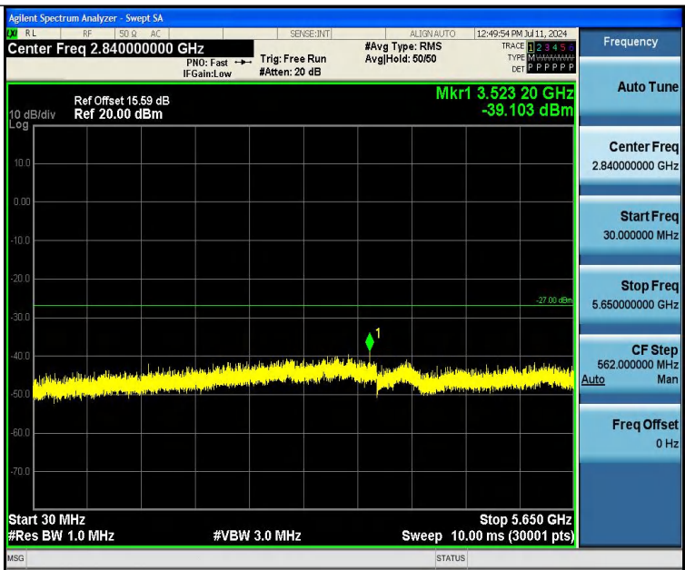
11N20SISO-Ant1-5825-30~5650-PASS
