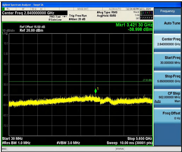
11A-Ant1-5825-30~5650-PASS
