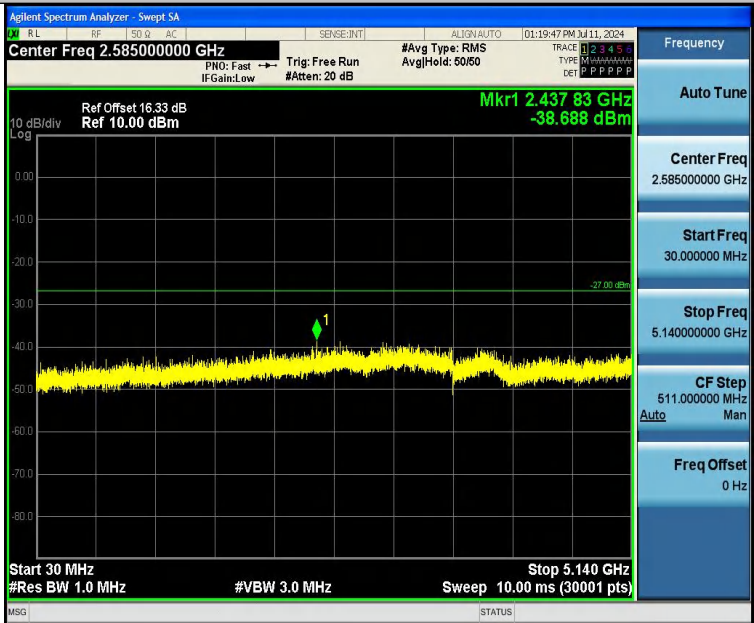
11AC40SISO-Ant1-5190-30~5140-PASS
