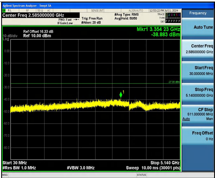
11N40SISO-Ant1-5190-30~5140-PASS
