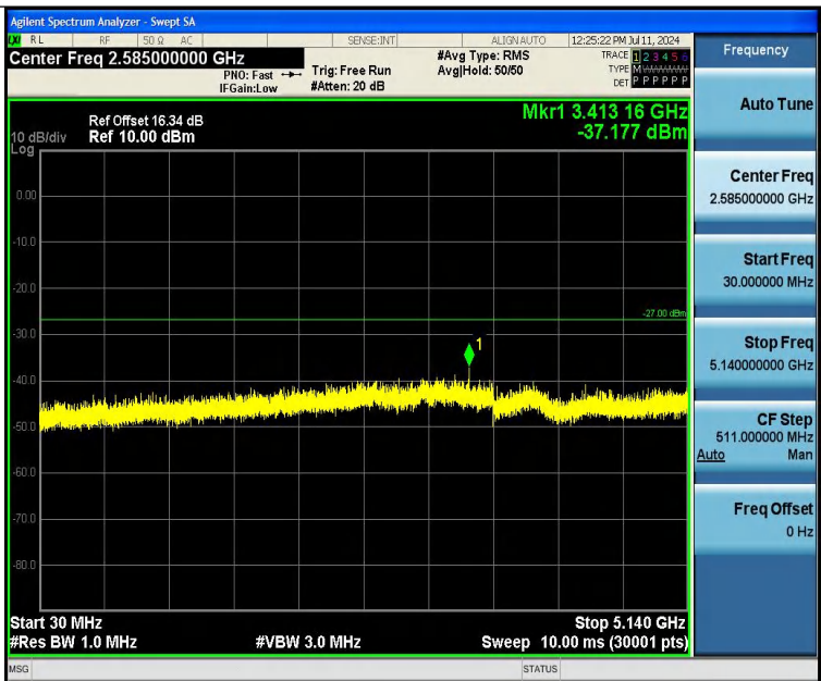
11A-Ant1-5200-30~5140-PASS
