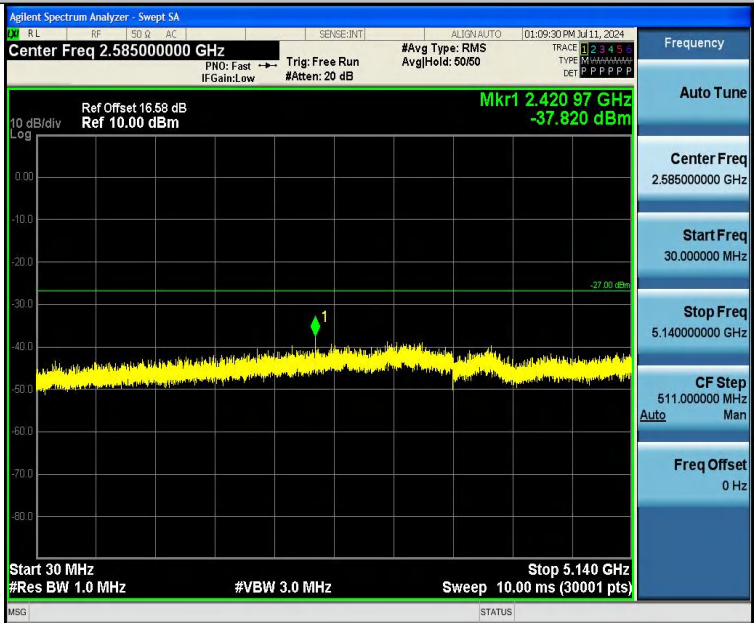
11AC20SISO-Ant1-5240-30~5140-PASS
