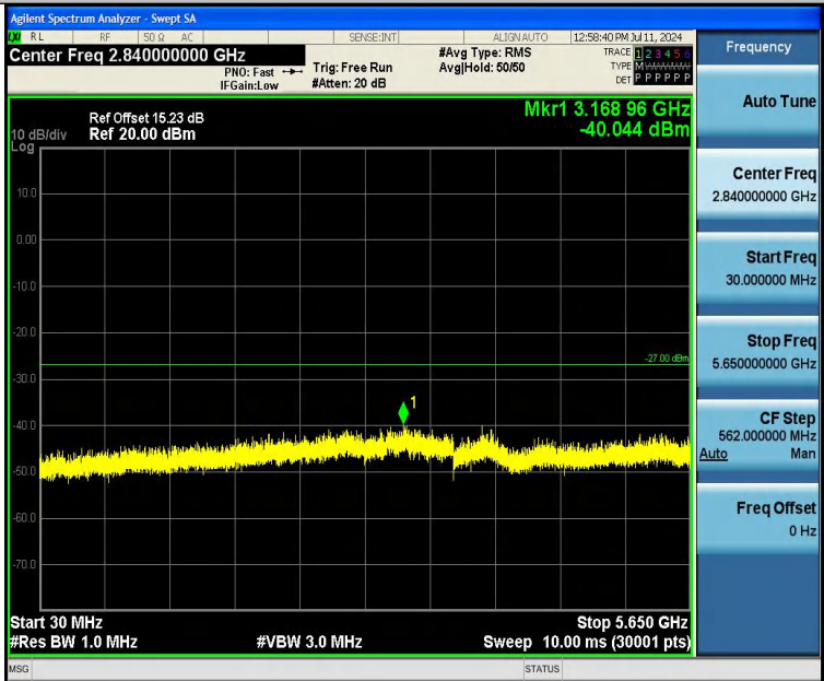
11N40SISO-Ant1-5755-30~5650-PASS
