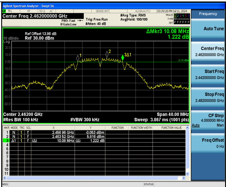
11B-Ant1-2462-PASS
