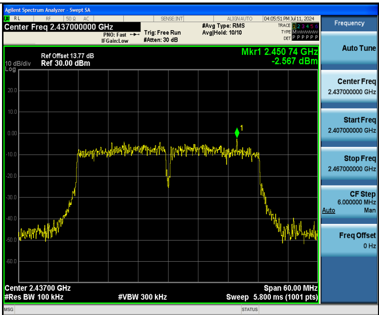
11N40SISO-Ant1-2437-0~Reference-PASS
