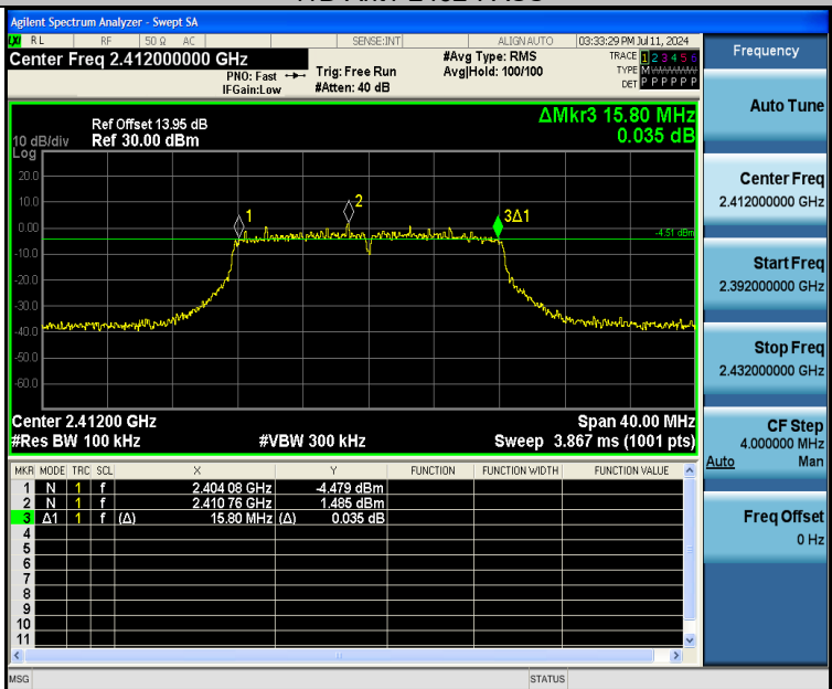
11G-Ant1-2412-PASS
