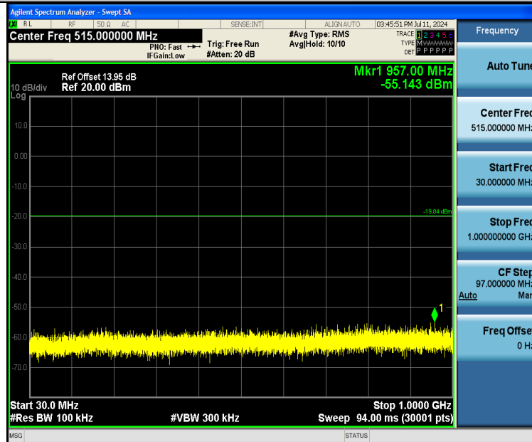
11N20SISO-Ant1-2412-30~1000-PASS
