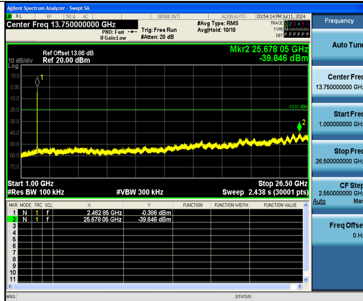
11N20SISO-Ant1-2462-1000~26500-PASS
