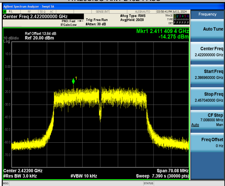
11N40SISO-Ant1-2422-PASS
