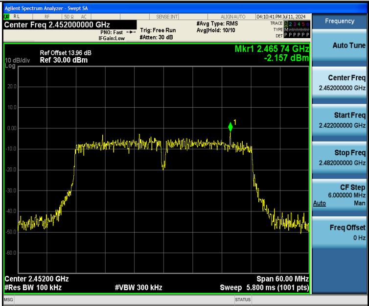
11N40SISO-Ant1-2452-0~Reference-PASS
