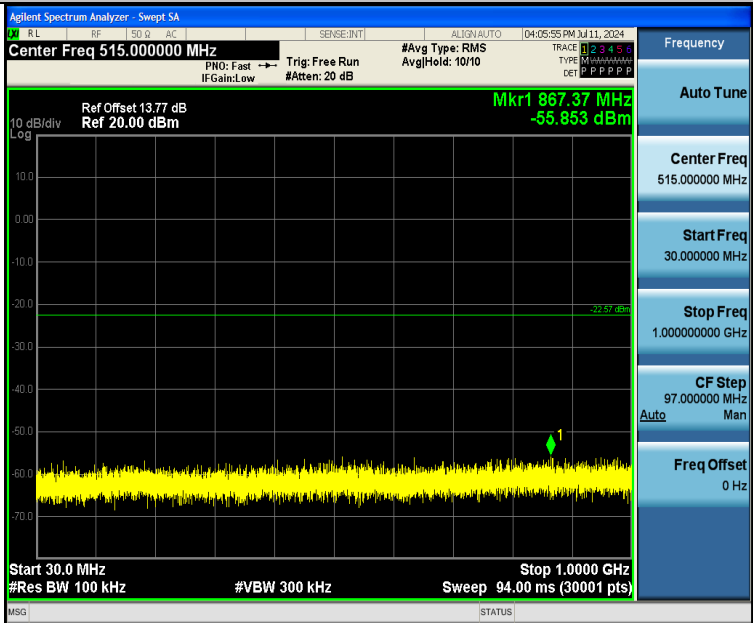
11N40SISO-Ant1-2437-30~1000-PASS
