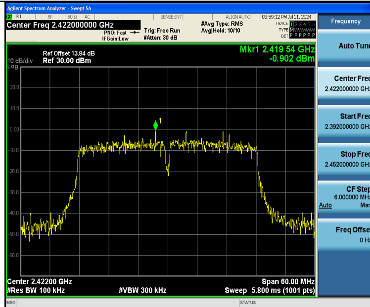
11N40SISO-Ant1-2422-0~Reference-PASS
