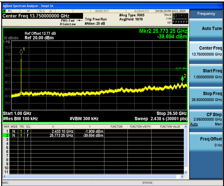
11N40SISO-Ant1-2437-1000~26500-PASS
