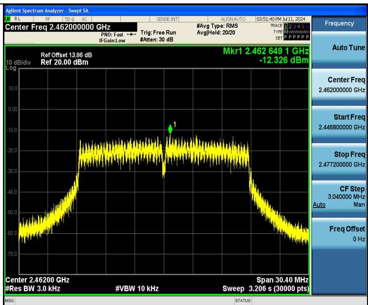
11N20SISO-Ant1-2462-PASS
