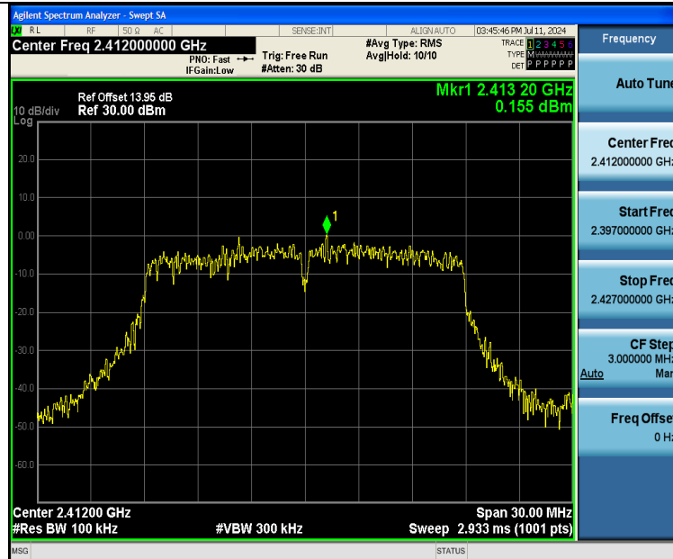
11N20SISO-Ant1-2412-0~Reference-PASS
