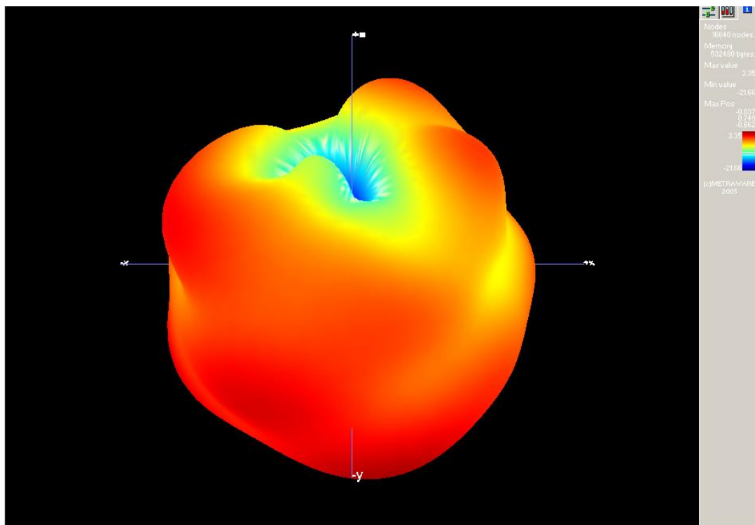
Picture2: direction diagram of 3D at 2.45GHz
