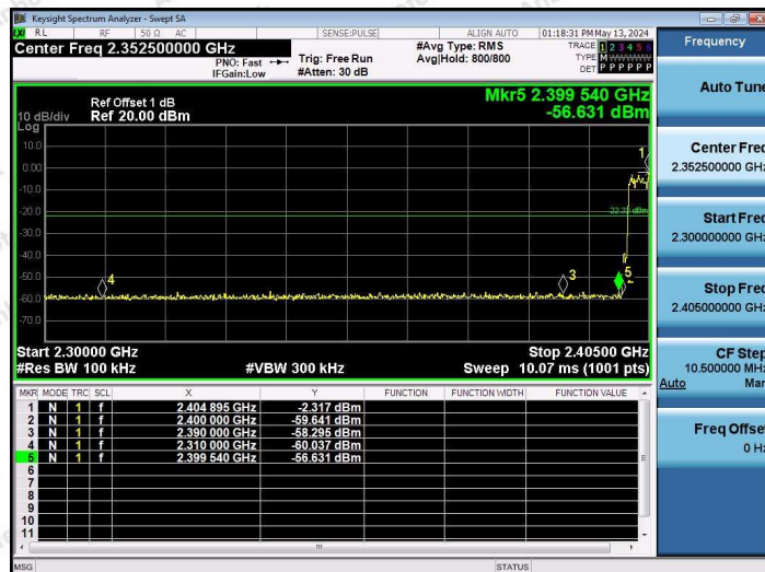
2DH5-Ant1-Hop_2402-PASS
