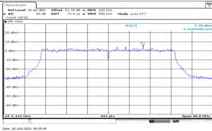
11AX20SISO_Ant1_2412_0~Reference
