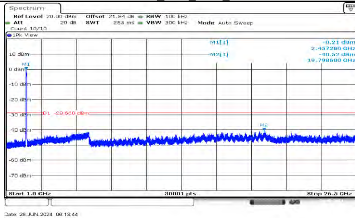
11AX40SISO_Ant1_2452_1000~26500
