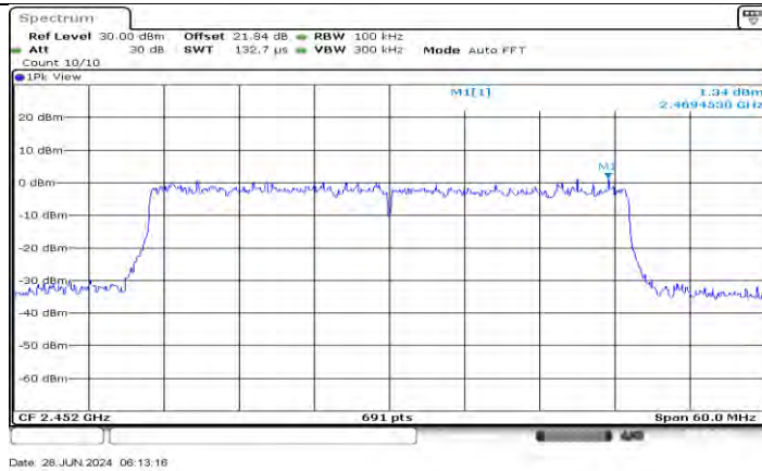
11AX40SISO_Ant1_2452_0~Reference
