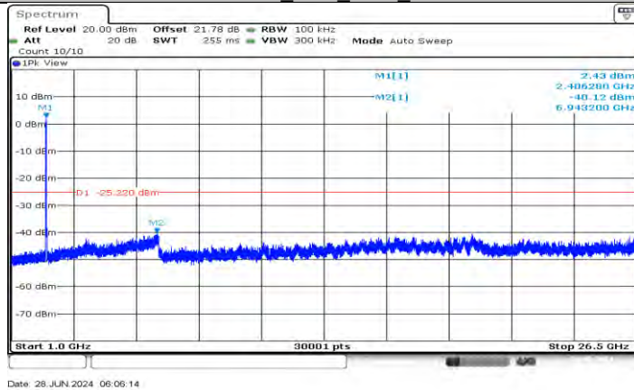
11AX20SISO_Ant1_2412_1000~26500
