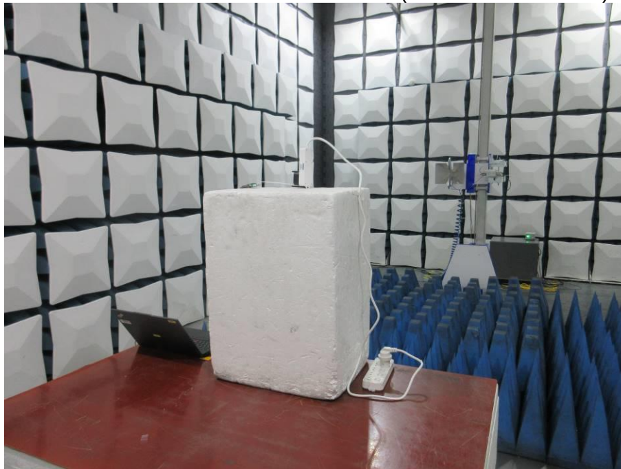
RADIATED RF MEASUREMENT SETUP (ABOVE 1 GHz-Y axis)
