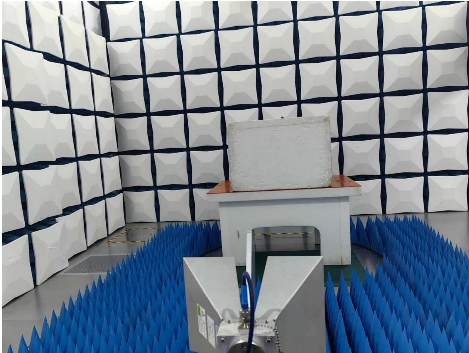
Test Set-up: Radiated spurious emission 1GHz to 5GHz
