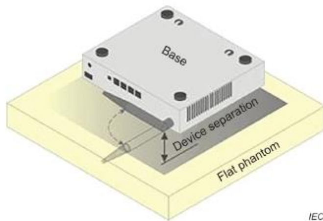
Figure 7 – Device with swivel antenna
