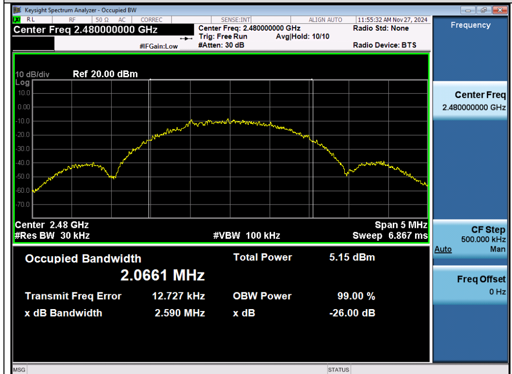
Test_Graph_LE2M_ANT1_2480_2Mbps_OBW
