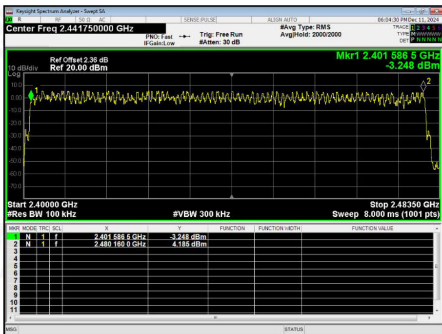
8-DPSK - 3-DH1 Test Plots
