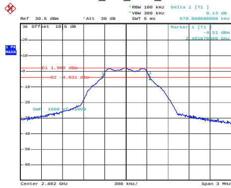
BLE_1M_Low_Channel
