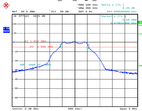
BLE_1M_High_Channel
