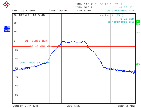
BLE_1M_Middle_Channel
