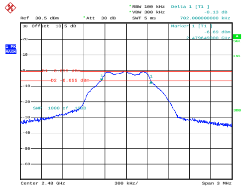
BLE_1M_High_Channel
