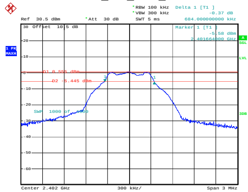
BLE_1M_Low_Channel
