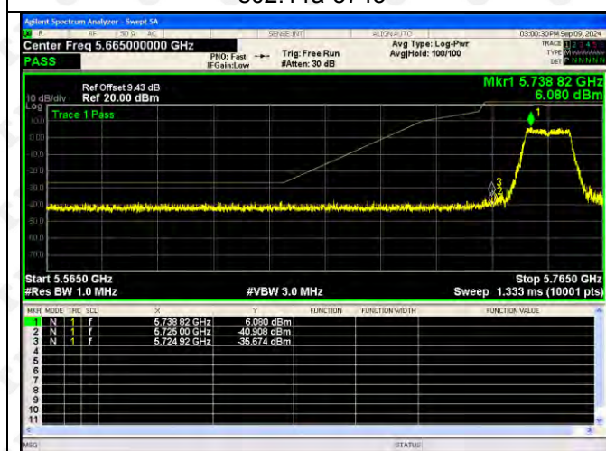
802.11ac(VH20)-5745
