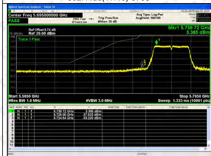
802.11ac(VH40)-5755
