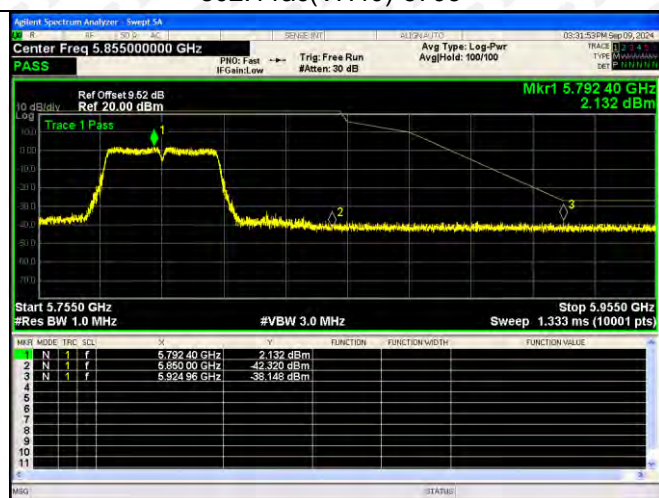
802.11ac(VH40)-5795
