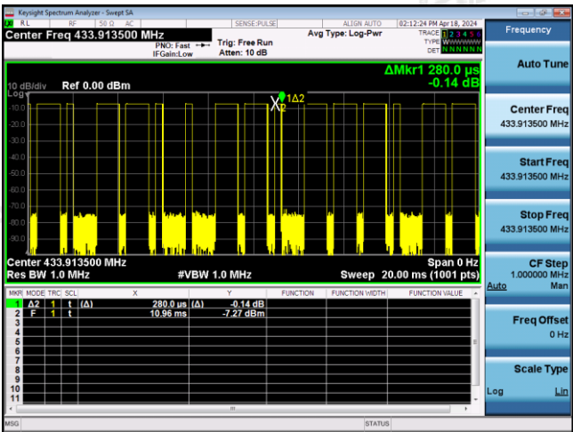
(Time per burst: 0.280ms*14pcs)
