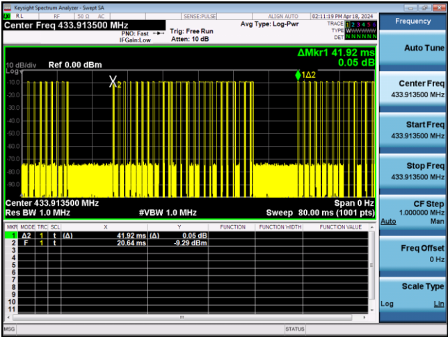
(Transmit cycle 41.92ms)
