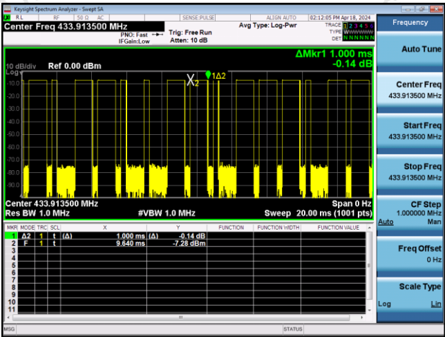
(Time per burst: 1.000ms*11pcs)
