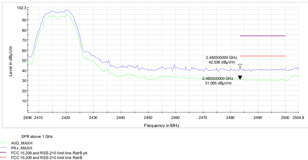
Figure 6.3-2: Band edge spurious emissions at high band edge
