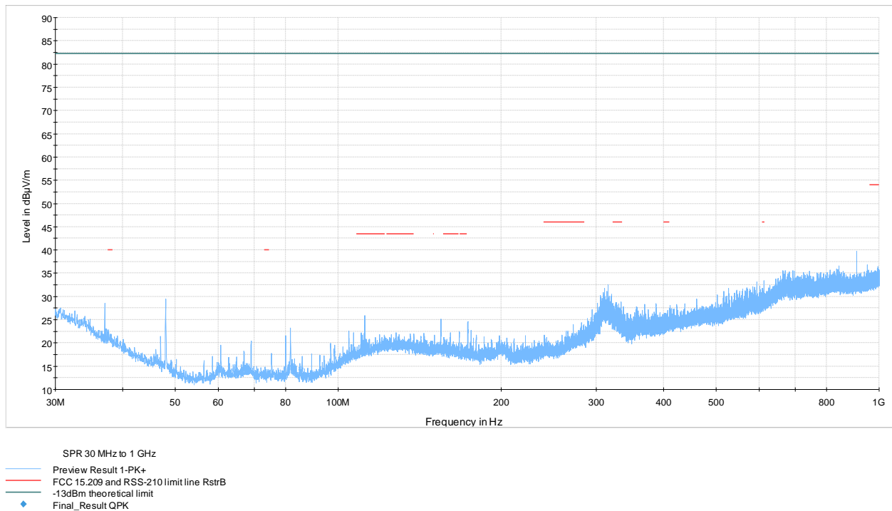
Figure 6.3-3: radiated spurious emissions from 30 MHz to 1000 MHz
