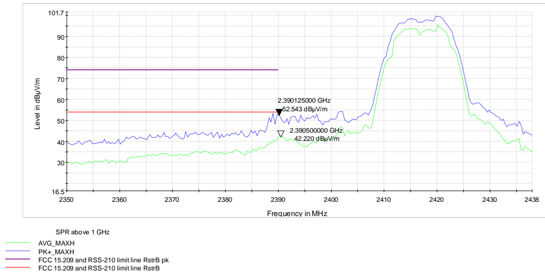
Figure 6.3-1: Band edge spurious emissions at low band edge
