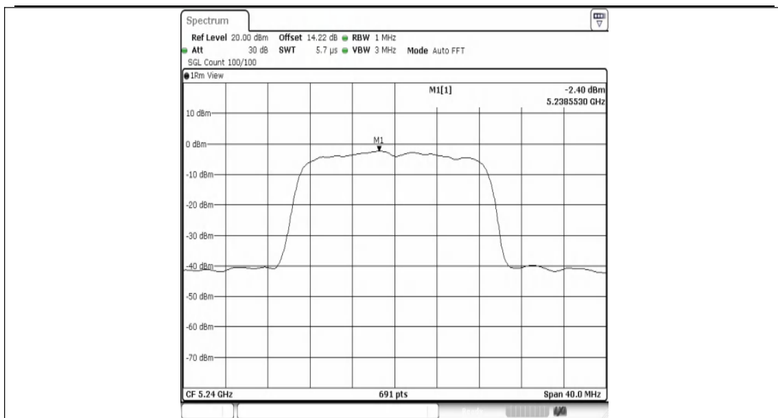
11AC20MIMO-Ant1-5240-PASS
