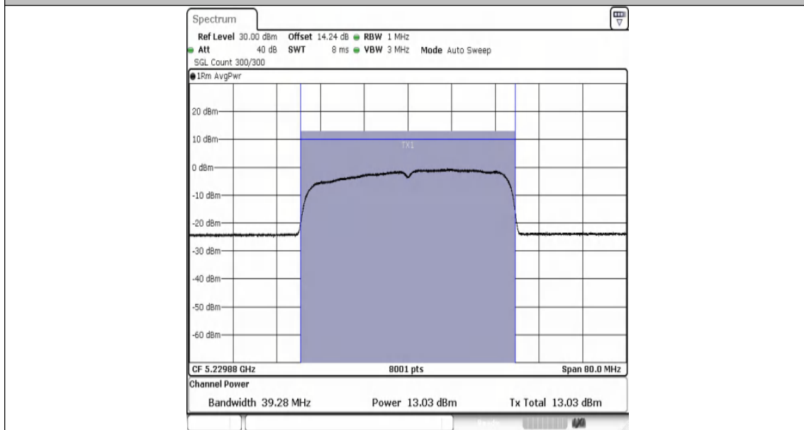
11AX40MIMO-Ant2-5230-PASS
