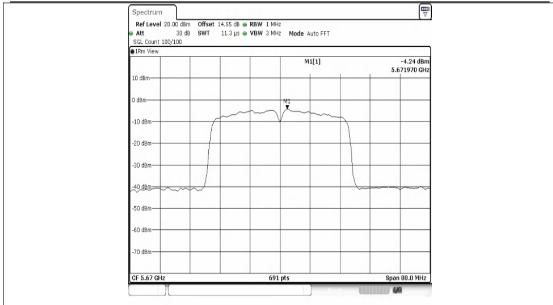
11N40MIMO-Ant1-5670-PASS
