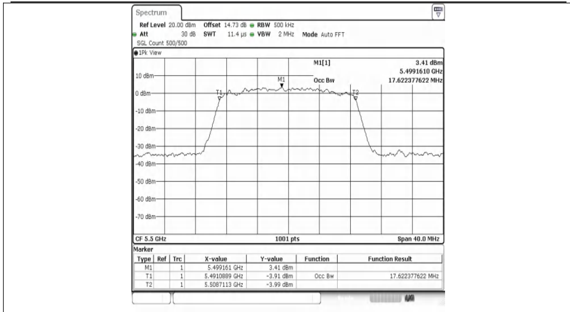
11AC20MIMO-Ant1-5500
