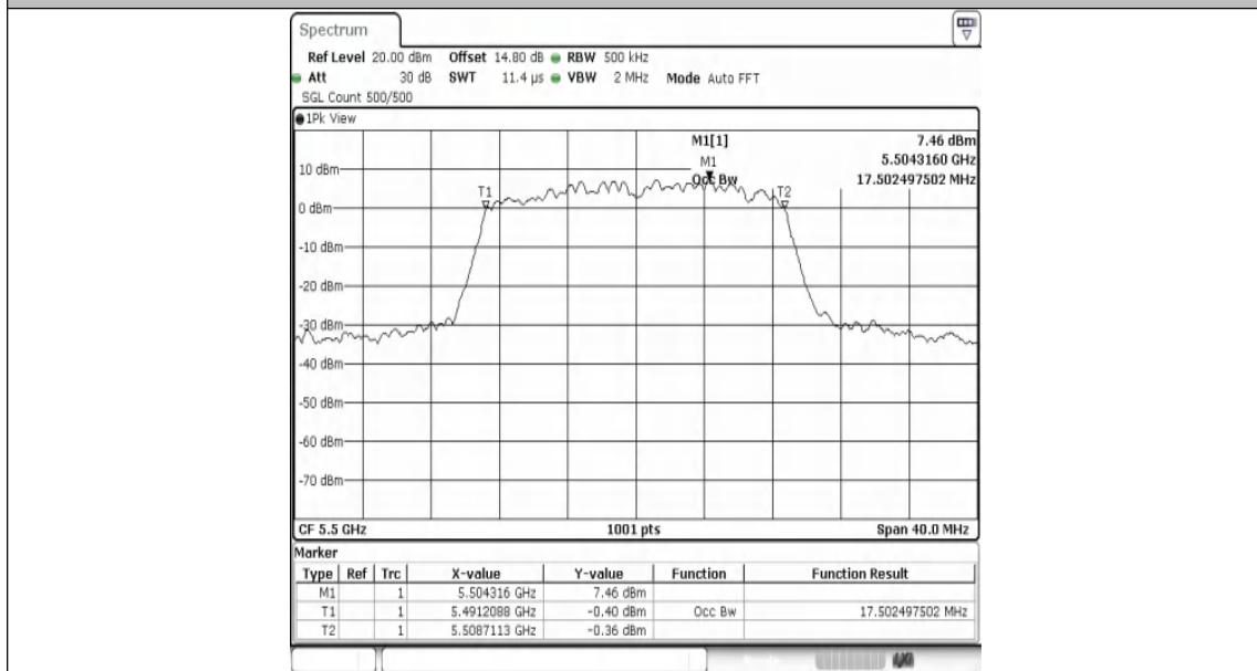
11AC20MIMO-Ant1-5500
