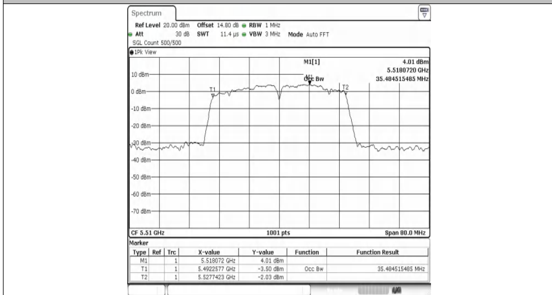
11AC40MIMO-Ant1-5510
