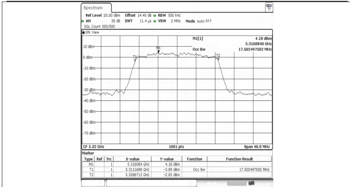
11AC20MIMO-Ant1-5320
