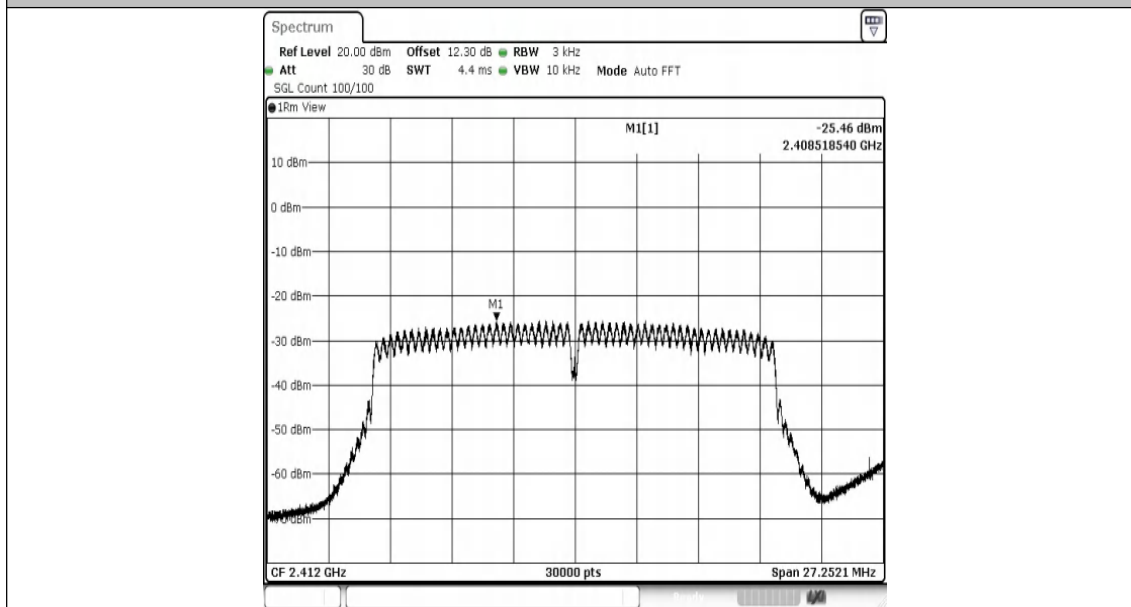
11N20MIMO-Ant2-2412-PASS
