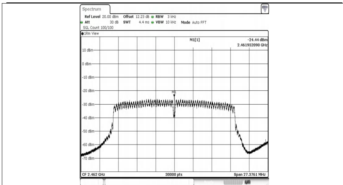
11N20MIMO-Ant1-2462-PASS
