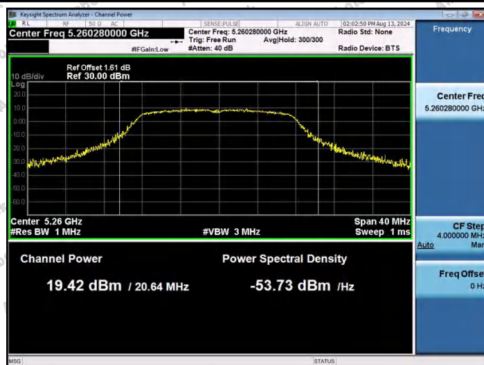
11A-Ant1-5260-PASS
