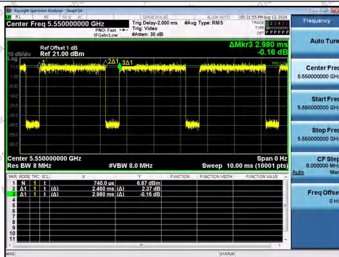
NTNV-11N40SISO-Ant1-5550
