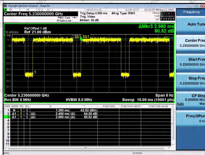
NTNV-11AC40SISO-Ant1-5230
