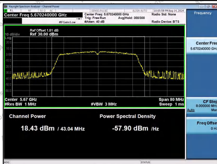
11N40SISO-Ant1-5670-PASS
