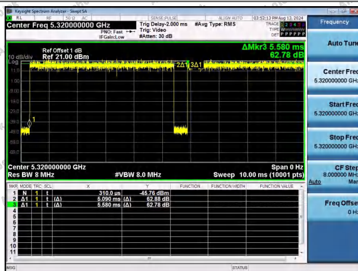
NTNV-11N20SISO-Ant1-5320
