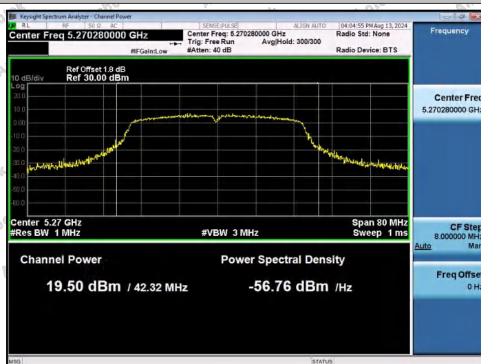
11AC40SISO-Ant1-5270-PASS
