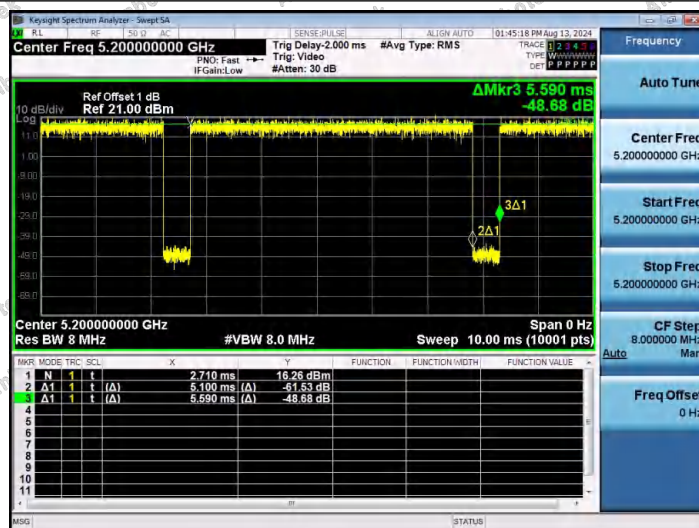
NTNV-11AC20SISO-Ant1-5200
