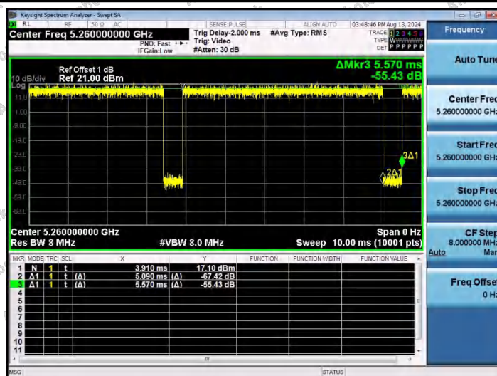
NTNV-11N20SISO-Ant1-5260
