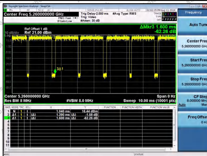
NTNV-11A-Ant1-5260
