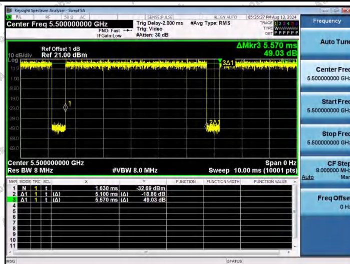
NTNV-11AC20SISO-Ant1-5500
