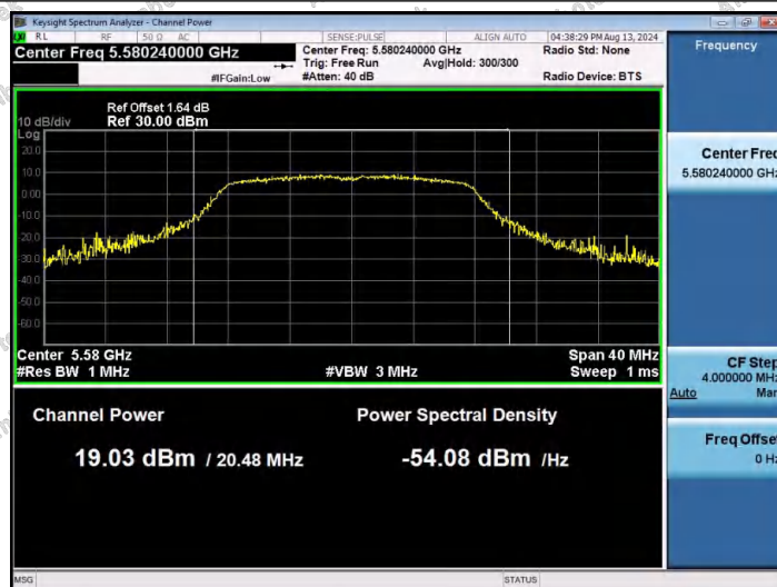
11A-Ant1-5580-PASS
