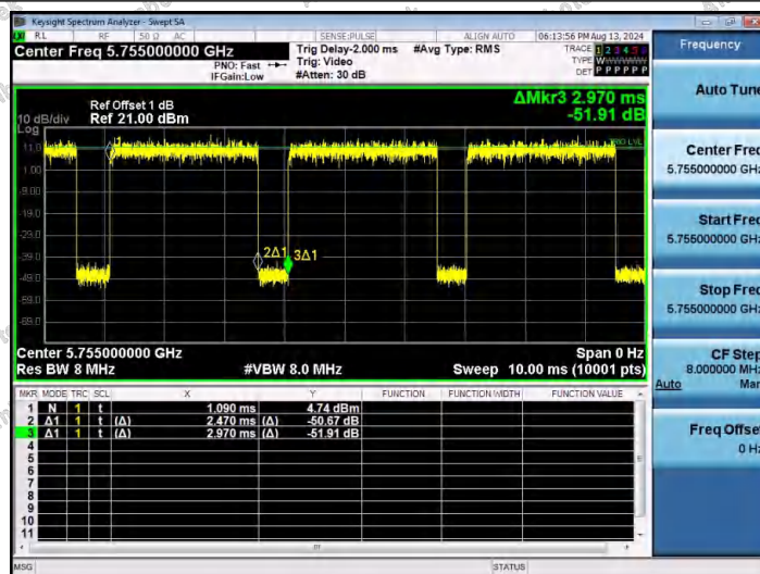
NTVN-11N40SISO-Ant1-5755
