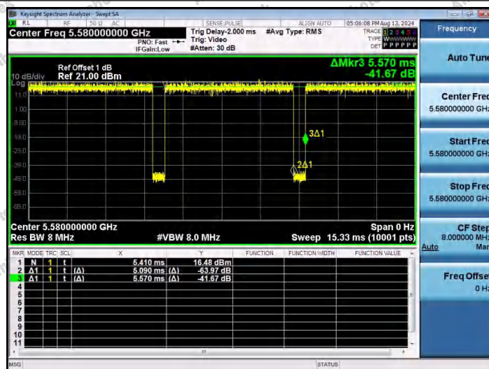
NTNV-11N20SISO-Ant1-5580
