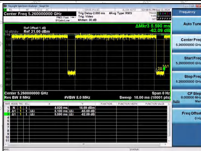
NTNV-11AC20SISO-Ant1-5260
