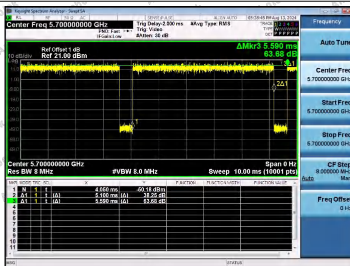
NTNV-11AC20SISO-Ant1-5700
