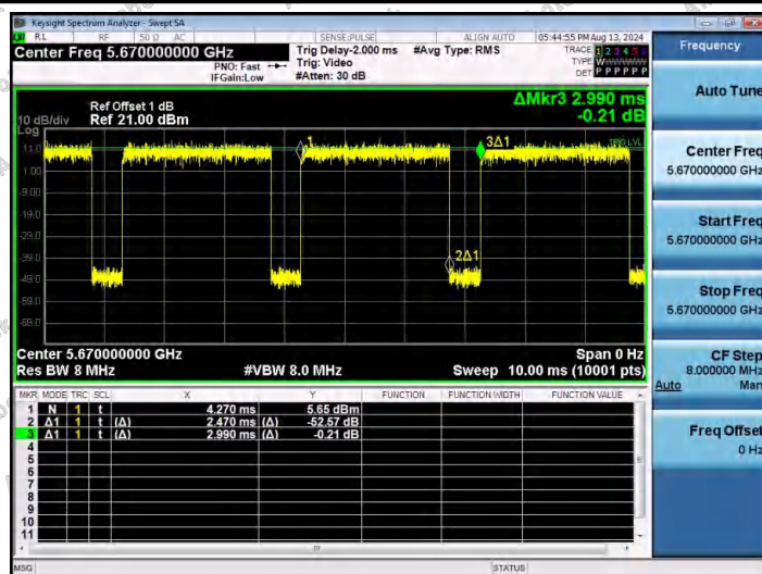
NTNV-11AC40SISO-Ant1-5670
