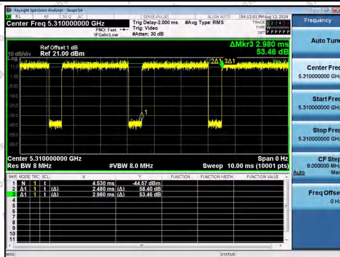
NTNV-11AC40SISO-Ant1-5310
