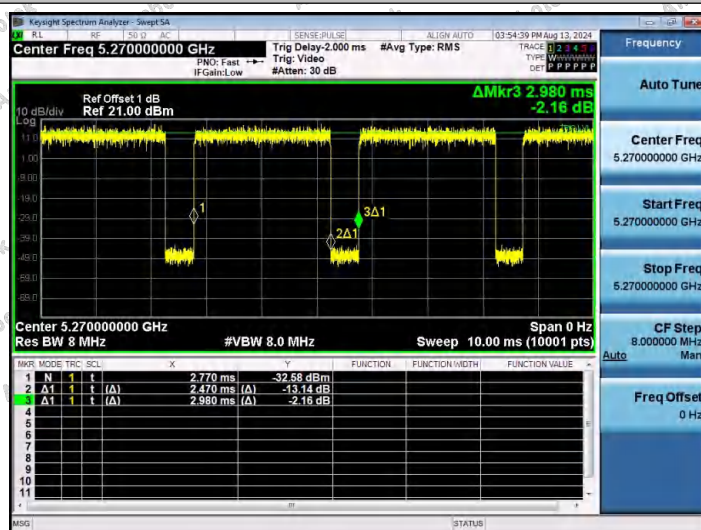
NTNV-11N40SISO-Ant1-5270
