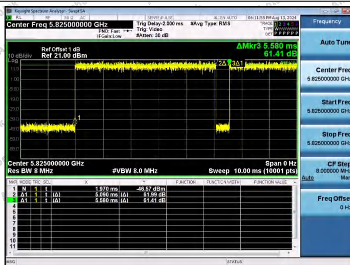
NTVN-11N20SISO-Ant1-5825
