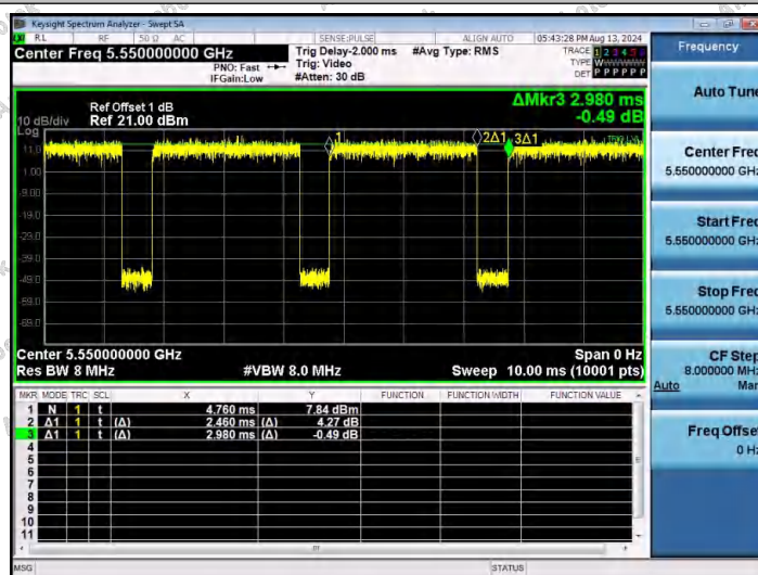
NTNV-11AC40SISO-Ant1-5550
