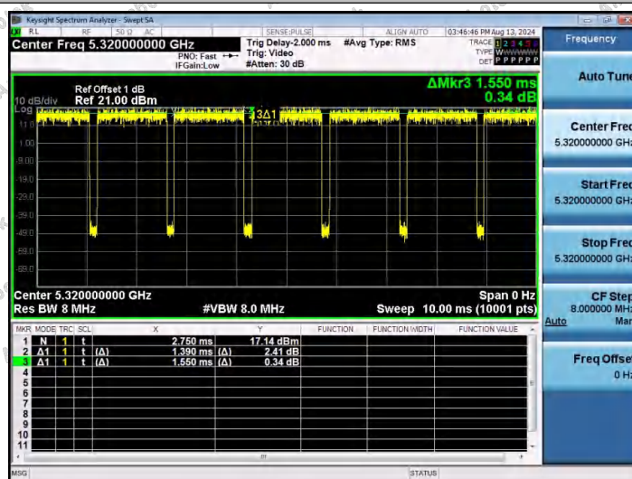
NTNV-11A-Ant1-5320
