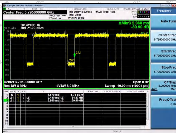
NTNV-11AC40SISO-Ant1-5795
