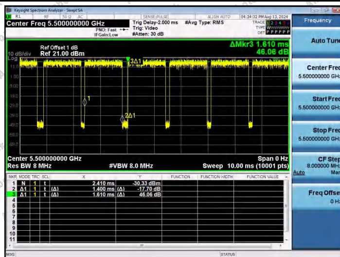
NTNV-11A-Ant1-5500
