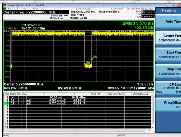
NTVN-11N20SISO-Ant1-5220
