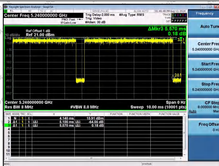
NTNV-11AC20SISO-Ant1-5240
