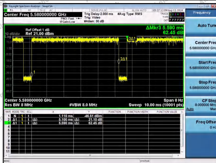
NTNV-11AC20SISO-Ant1-5580
