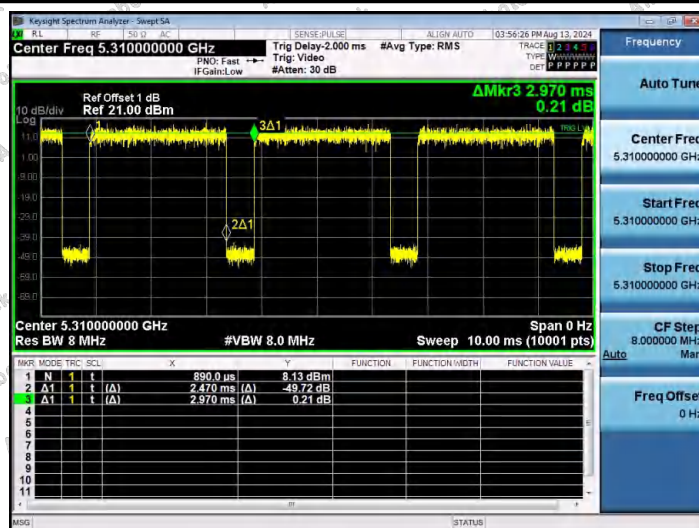
NTNV-11N40SISO-Ant1-5310
