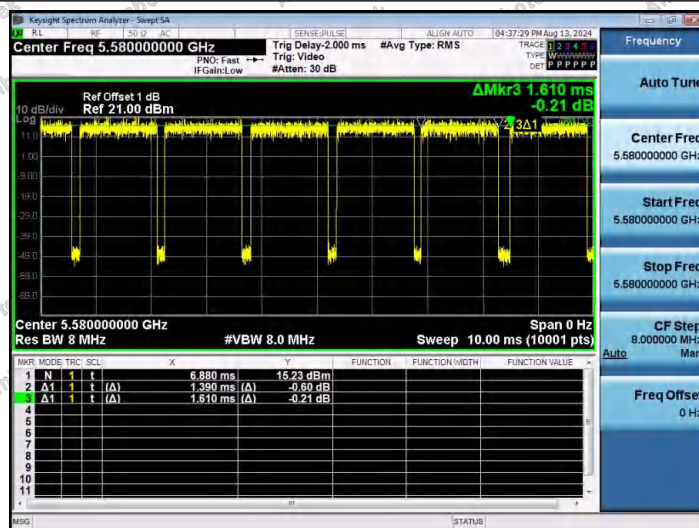
NTNV-11A-Ant1-5580
