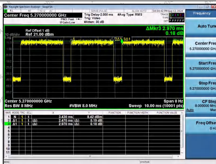
NTNV-11AC40SISO-Ant1-5270
