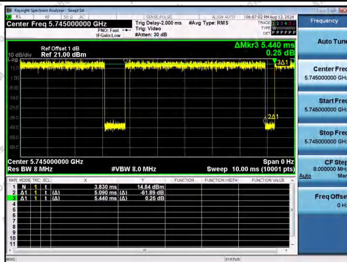
NTVN-11N20SISO-Ant1-5745
