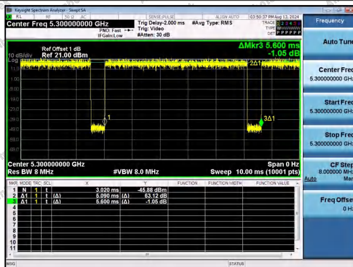
NTNV-11N20SISO-Ant1-5300
