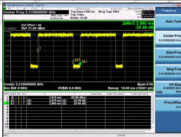
NTNV-11AC40SISO-Ant1-5510
