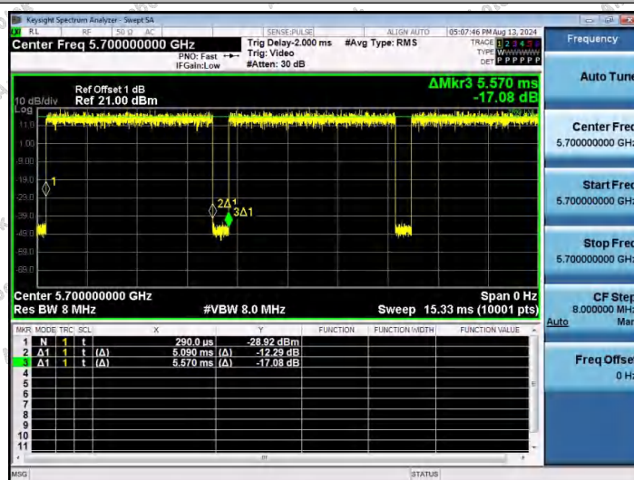
NTNV-11N20SISO-Ant1-5700
