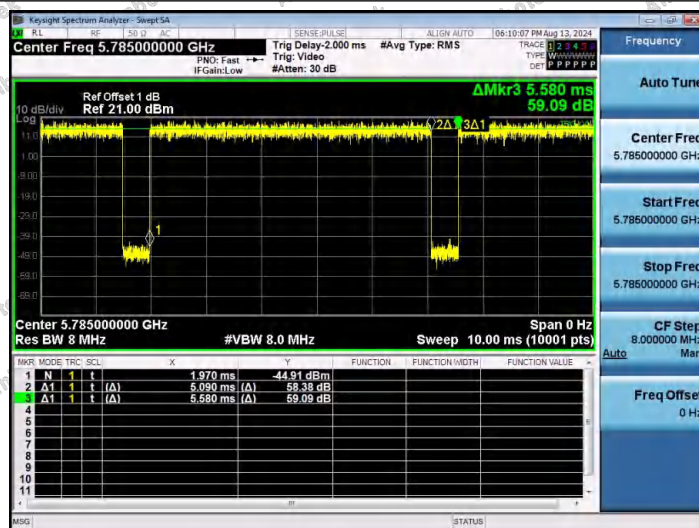
NTVN-11N20SISO-Ant1-5785
