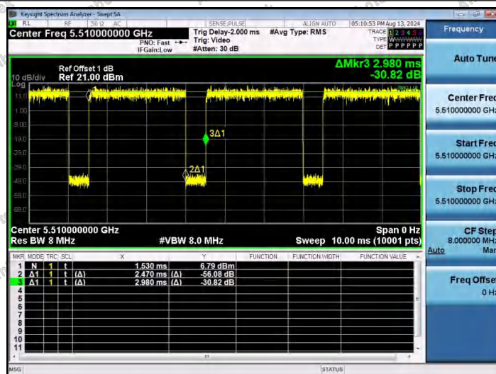
NTNV-11N40SISO-Ant1-5510
