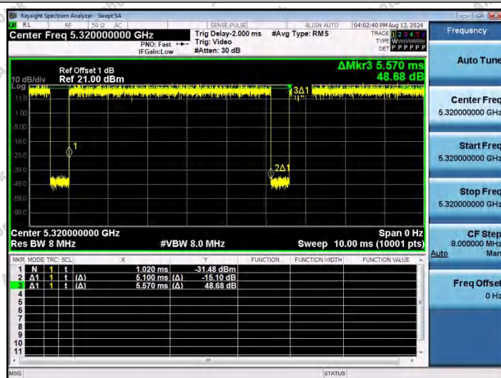
NTNV-11AC20SISO-Ant1-5320
