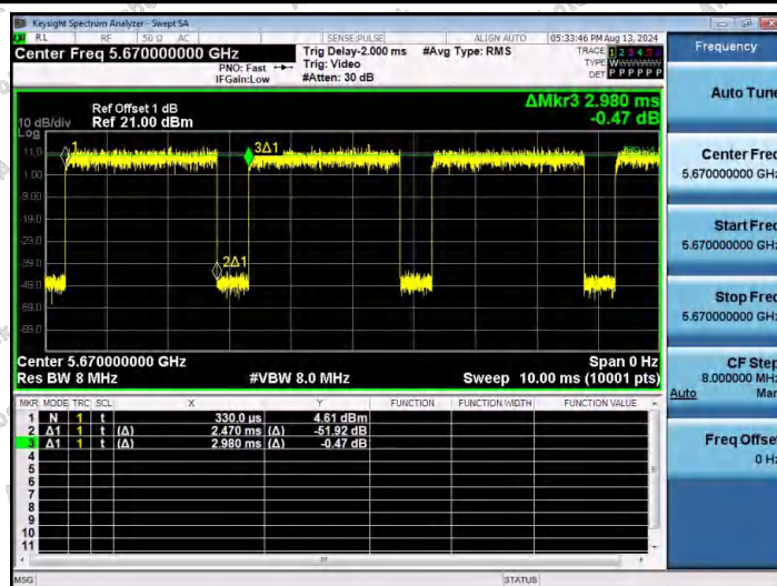
NTVN-11N40SISO-Ant1-5670
