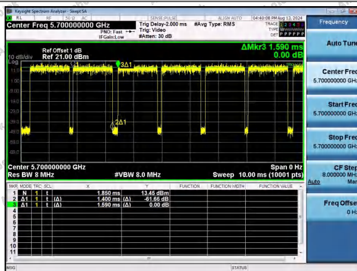
NTNV-11A-Ant1-5700
