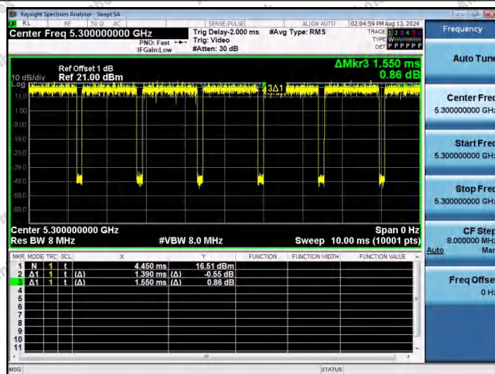
NTNV-11A-Ant1-5300
