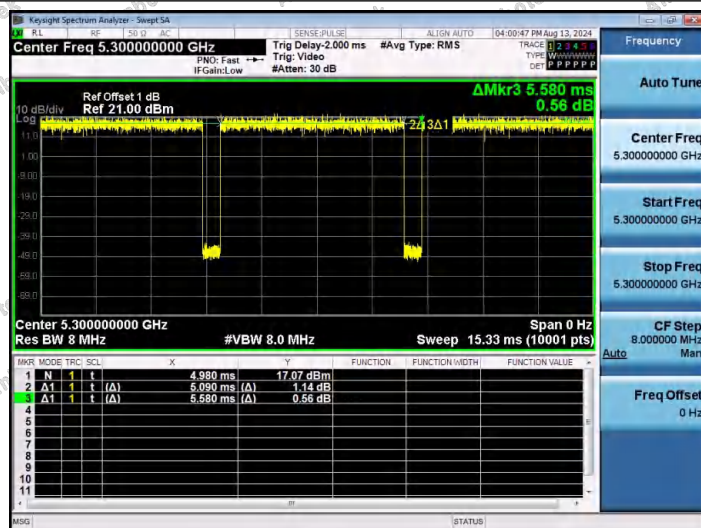
NTNV-11AC20SISO-Ant1-5300
